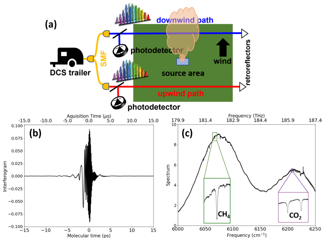
105 Figure 1: (a) Schematic of the dual-comb spectrometer gas concentration measurements on two paths from a \text{CH}_4 source area. Yellow lines indicate single-mode fiber (SMF) transmitting dual-comb light to an upwind (red) and downwind (blue) open-air paths. \text{CH}_4 is emitted from an area between the two paths under proper wind directions. RF signals from two photodetectors are sent back to the trailer and two interferograms (IGM) containing gas concentration information for each path are digitized. (b) A dual-comb spectroscopy phase-corrected IGM after 5 min acquisition time on the upwind path. ‘Acquisition time’ is the microsecond timescale of the measured RF voltage. ‘Molecular time’ is the timescale associated with the period of molecular oscillations which is typically picoseconds. (c) The Fourier transform of the IGM with insets showing \text{CH}_4 and \text{CO}_2 absorption lines and the laser baseline.
