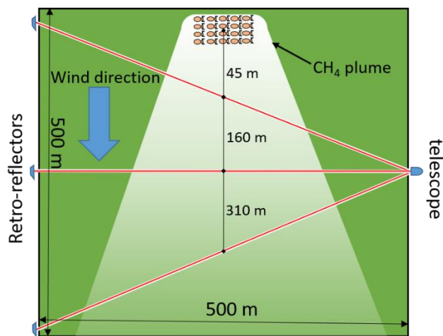
130 Figure 2: Schematic diagram showing the location of the hypothetical herd of cattle, transceiver, retroreflectors and three possible downwind paths used for the forward WindTrax simulations. A constant background of 2000 nmol/mol was assumed so no upwind path was used in the simulation and not shown in the figure.
