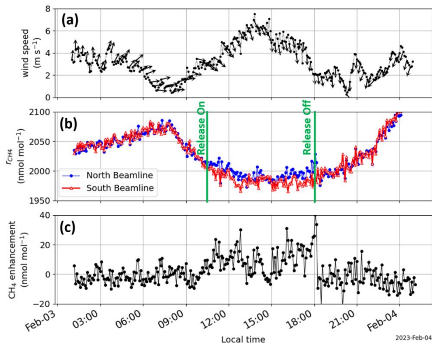
Figure 5: 5-min values of (a) wind speed and direction, (b) dry \text{CH}_4 mole fraction ( r_{\text{CH}_4} ), and (c) enhancement during a controlled \text{CH}_4 release of 3078 \text{ g d}^{-1} equivalent to 15 head of cattle assuming a \text{CH}_4 rate of 208 \text{ g head}^{-1} \text{ day}^{-1} . Wind arrows point in the direction from which the wind is blowing. During the release, wind was mostly from the south causing an enhancement on the North Beamline.
