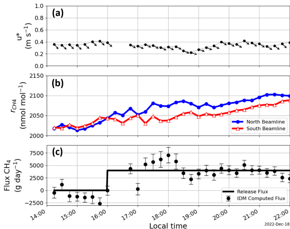
285 Figure 7: Timeseries of (a) wind friction velocity and direction, (b) \text{CH}_4 dry mole fraction ( r_{\text{CH}_4} ), and (c) release and IDM computed \text{CH}_4 flux for a \text{CH}_4 release of 3970 \text{ g day}^{-1} equivalent to 19 head of cattle. Wind arrows point in the direction from which the wind is blowing.
