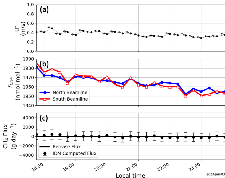
Figure 6: Time series of (a) wind friction velocity and direction, (b) dry \text{CH}_4 mole fraction ( r_{\text{CH}_4} ), and (c) release and IDM computed \text{CH}_4 flux a case of no released gas. The error bars are uncertainties due to the DCS measured concentrations calculated using Eq. 2. Wind arrows point in the direction from which the wind is blowing.
