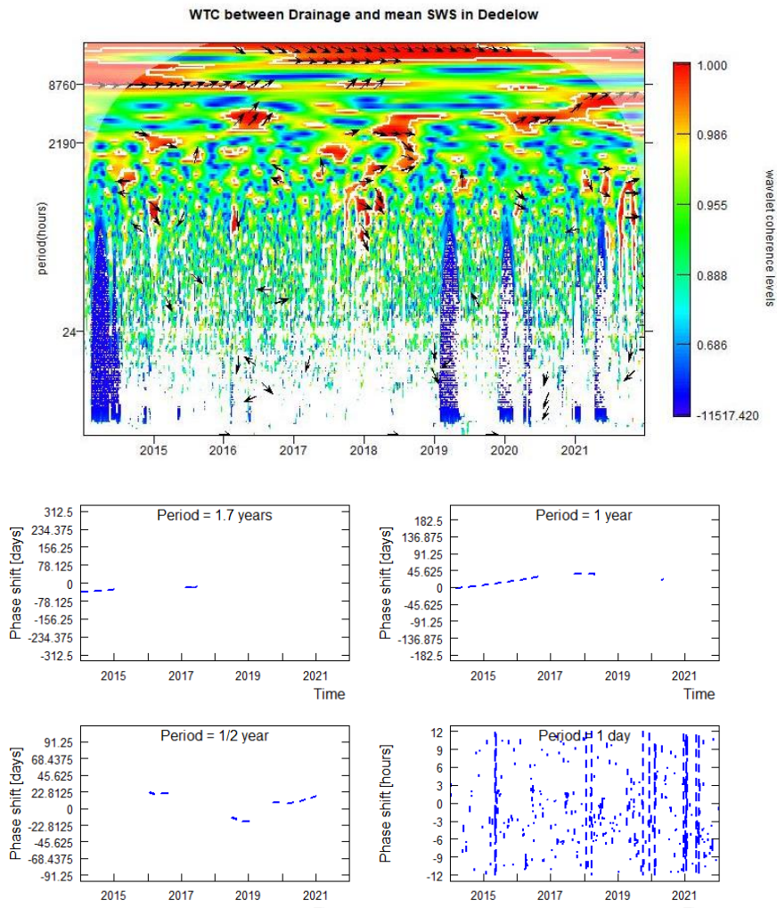
840 Figure C2: Wavelet coherence spectrum and time shifts between Q_{net} and SWS in Dedelow
