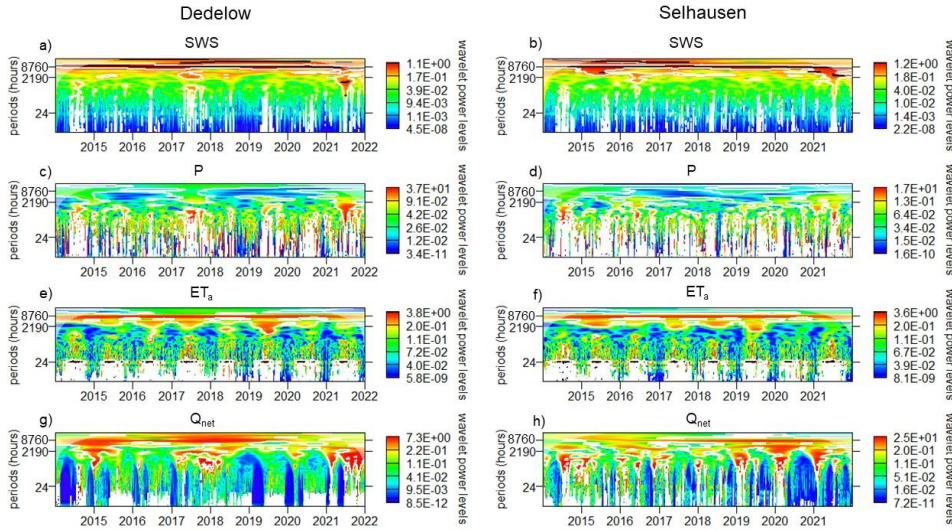
355 Figure 3: Wavelet spectra of the soil water storage change (SWS), P, ET_a and bottom drainage Q_{net} (up- and downward flux) of the lysimeters in Dedelow and Selhausen. Time is depicted on the x-axis and the y-axis denotes the periodicity in hours (24h = daily scale, 8760 h = annual scale). The colour indicates the wavelet power level that indicates shows the similarity of the frequency of the wavelet with the frequency of the time series at the given scale and at the point in time. Areas in the wavelet spectrum that deviate significantly from the red noise background spectrum (significance level = 10 %) are surrounded by the white edging. Since at smaller scales the white rim (indicating significant areas in the wavelet plots) is rather omnipresent, the average significant periodicities are indicated by black lines (e.g., panel f). A logarithmic scale for the wavelet power levels was chosen to amplify differences in wavelet coefficients between different parts of the spectra visually. The shaded area at the edge of the plot at higher scales is called the cone of influence. Here, edge effects due to the padding of the time series with zeroes at the beginning and the end might influence the appearance of the wavelet spectrum and thus should be interpreted with caution.
