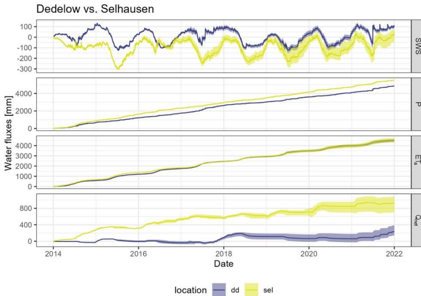
330 Figure 2: Hourly soil water storage change (SWS) and cumulative sum of precipitation (P), actual evapotranspiration ( ET_a ) and bottom flux (up- and downwards, Q_{net} ) of the lysimeters since 01-01-2014 in Dedelow (dd) and Selhausen (sel). The shaded areas represent the cumulative minimum and maximum values of the hourly data derived from the three lysimeters at each of the two sites.
