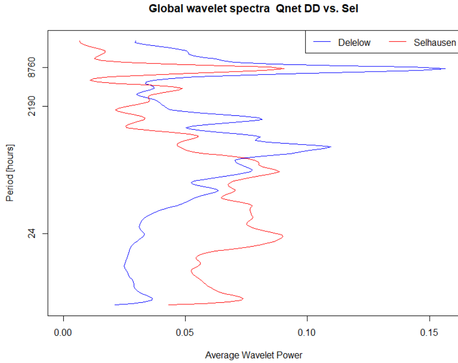
830 Figure B1: Global-Periods (hours) versus average wavelet power of the global wavelet spectra for Q_{net} from Dedelow and Selhausen.
