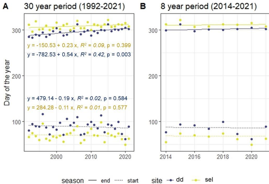
575 Figure 8: Variation of beginning and end of the vegetation period in Dedelow (DD) and Selhausen (SE) over a 30-year period from 1992 to 2021 (A) and over the observation period of 8 years from 2014 to 2021 (B). Calculations were executed according to Ernst and Loeper (1976) with hourly temperature data. “End” indicates the days of each year, when the growing season stopped, whereas “start” indicates the days of each year, when growing season started.
