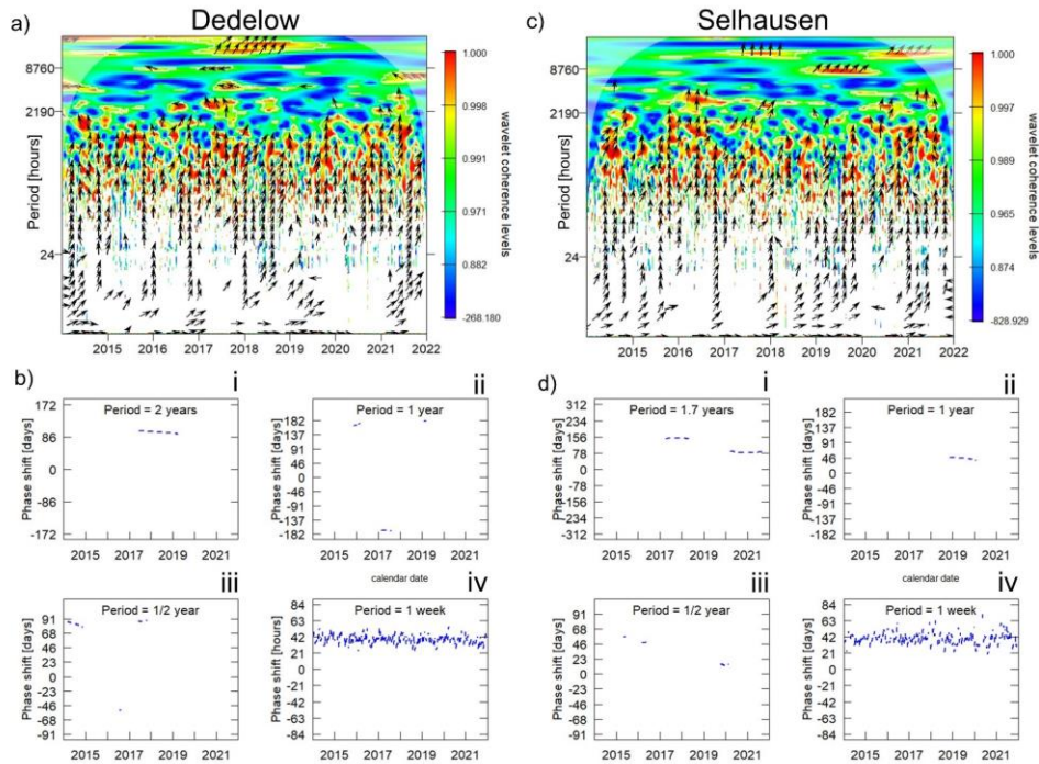
485 Figure 6: WCA between precipitation P and SWS in Dedelow (a) and Selhausen (c) and time shifts expressed in days and hours for selected scales in Dedelow (b) and Selhausen (d). For explanation of the plot layout refer to Figure 5.
