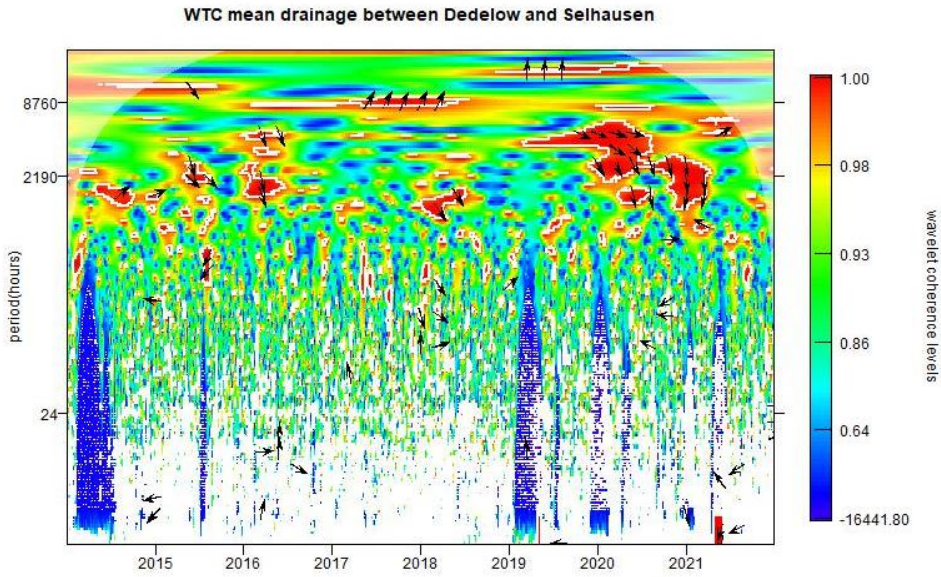
835 Figure C1: Wavelet coherence spectrum of Q_{net} in Dedelow and Selhausen
