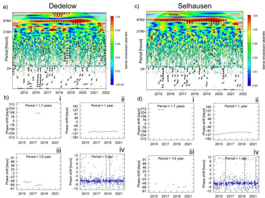
540 Figure 7: WCA between evapotranspiration- ET_a and SWS in Dedelow (a) and Selhausen (c) and time shifts expressed in days and (hours) for selected scales in Dedelow (b) and Selhausen (d). For explanation of the plot layout, we refer to Figure 5.
