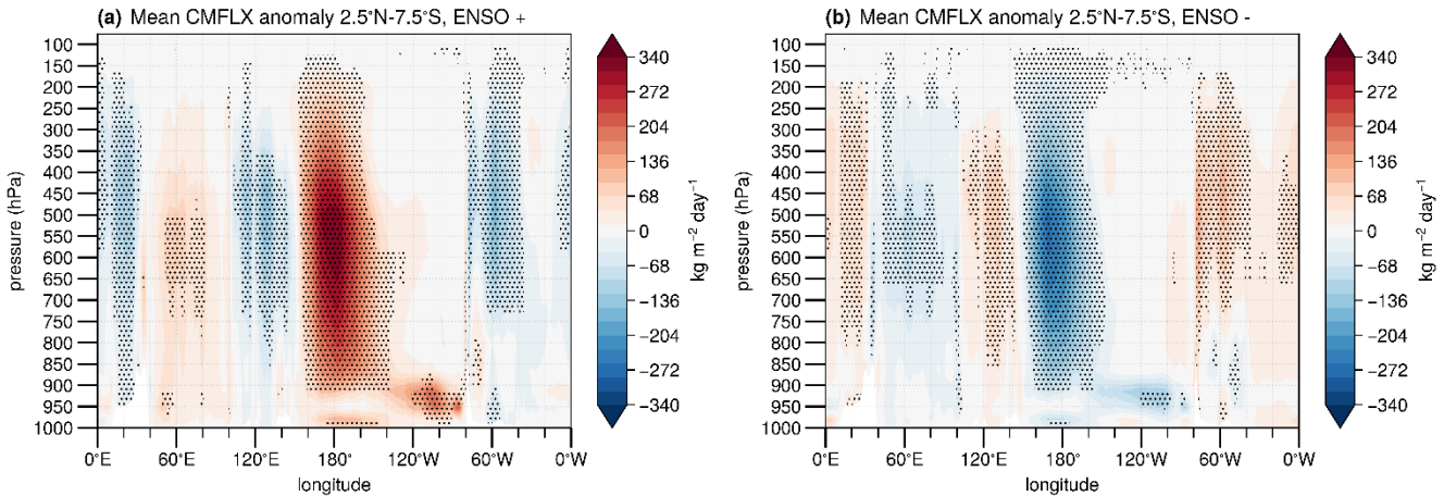
Figure 93. RAQMS-Aura convective mass flux (CMFLX) anomalies for a) positive and b) negative ENSO phases. Shaded regions indicate where the composite is significant at the 95% confidence level from a t test.
