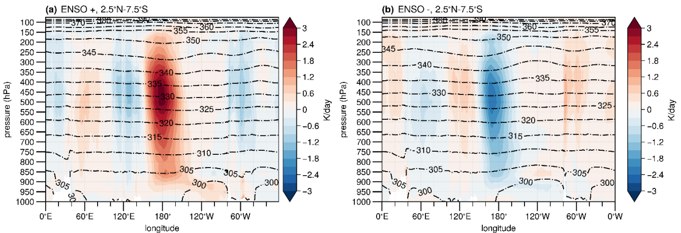
375 Figure 104. RAQMS-Aura diabatic heating anomalies (colors) and theta (contours) for a) positive and b) negative ENSO phases.
