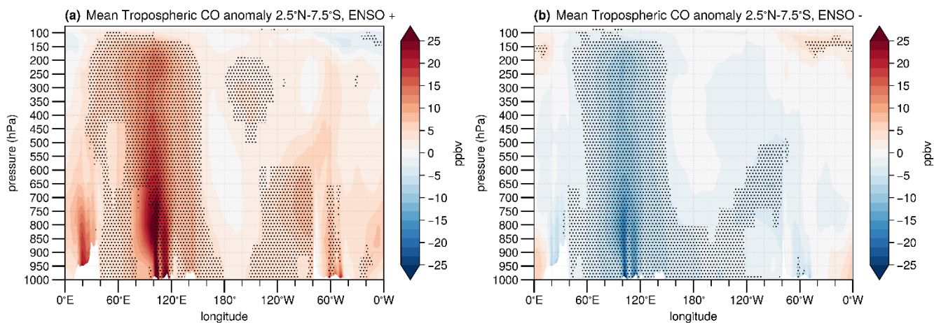
405 Figure 126. Anomalies in RAQMS-Aura CO profiles below the tropopause associated with a) El Niño and b) La Niña. Shaded regions indicate where the composite is significant at the 95% confidence level from a t test.
