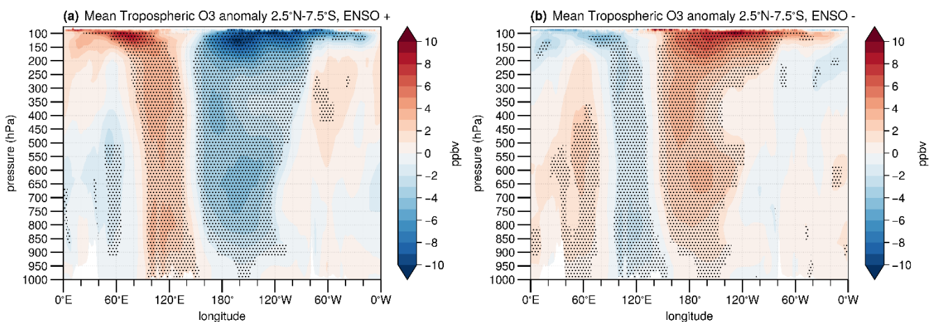
Figure 115. Anomalies in RAQMS-Aura ozone profiles below the tropopause associated with a) El Niño and b) La Niña. Shaded regions indicate where the composite is significant at the 95% confidence level from a t test.
