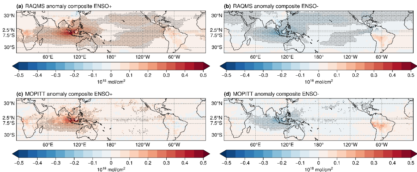
345 Figure 12. Composited CO column anomalies associated with El Niño in RAQMS-Aura (a) and MOPITT (c) and La Niña in RAQMS-Aura(b) and MOPITT(d). Shaded regions indicate where the composite is significant at the 95% confidence level from a t test.
