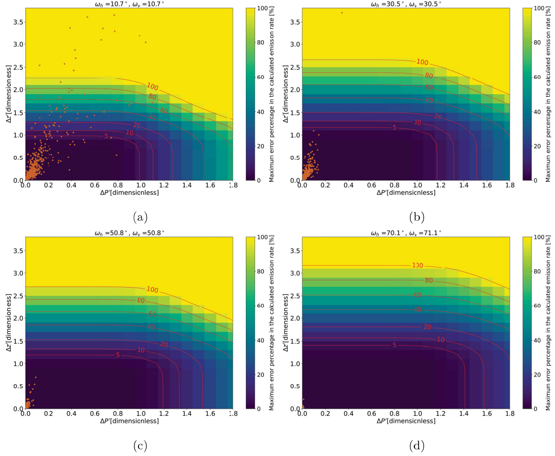
Figure 9. Contours indicate maximum calculated emission rate error (over 225 calculations corresponding to missing the plume by different percentages of the horizontal and vertical spacing) for varying dimensionless horizontal and vertical spacings for four different groups of plume opening angles: a) plume opening angle of 10.7^\circ , b) plume opening angle of 30.5^\circ , c) plume opening angle of 50.8^\circ , and d) plume opening angle of 71.1^\circ . The orange dots indicate the horizontal and vertical spacings for four different groups of plume opening angles a) between 0^\circ and 22.5^\circ , b) between 21.4^\circ and 45^\circ , c) between 45^\circ and 67.5^\circ and d) between 67.5^\circ and 90^\circ . Shown with red are the error contours.
