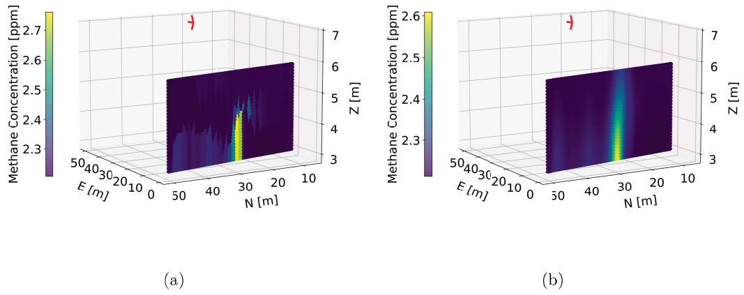
Figure D4. 3-dimensional interpolated concentration values for the upward curtain “4”, Figure8c using a) Nearest Neighbor and b)Gaussian smoother interpolation techniques. The red arrow indicate the average wind direction.
