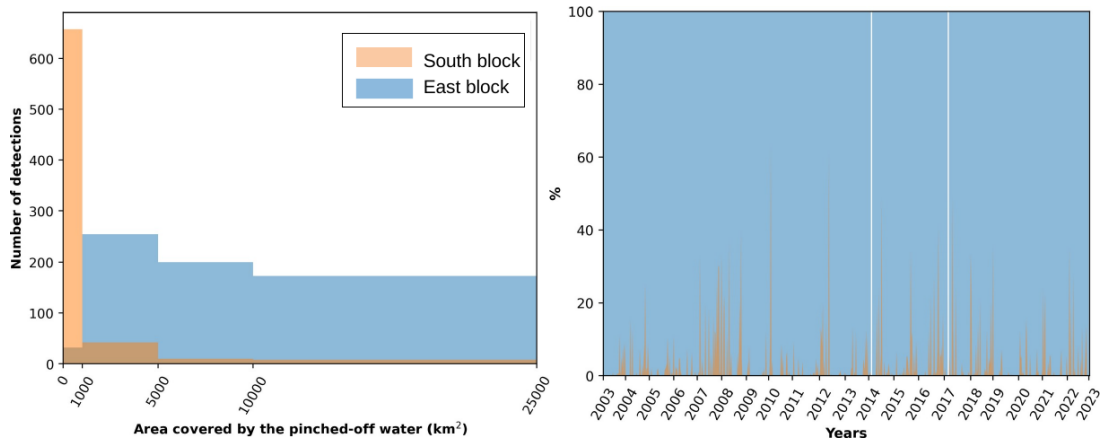
Figure 8. The histogram in the left panel illustrates the surface covered by the pinched-off water in the east (blue) and south (orange) blocks from 2003 to 2023. The right panel shows the percentage variation of each block contribution to the total pinched-off water. The white vertical lines represent days where the pinching-off events were absent in both blocks.
