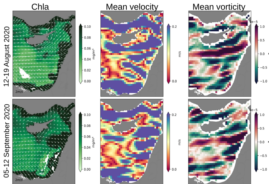
Figure 14. Two chlorophyll images (12-19 August 2020 and 05-12 September 2020) (left panel) compared the altimetry-derived average velocity field (middle panel) and relative vorticity (right panel). The chlorophyll images are overlaid by the average velocity field of the average wind speed for the corresponding days.
