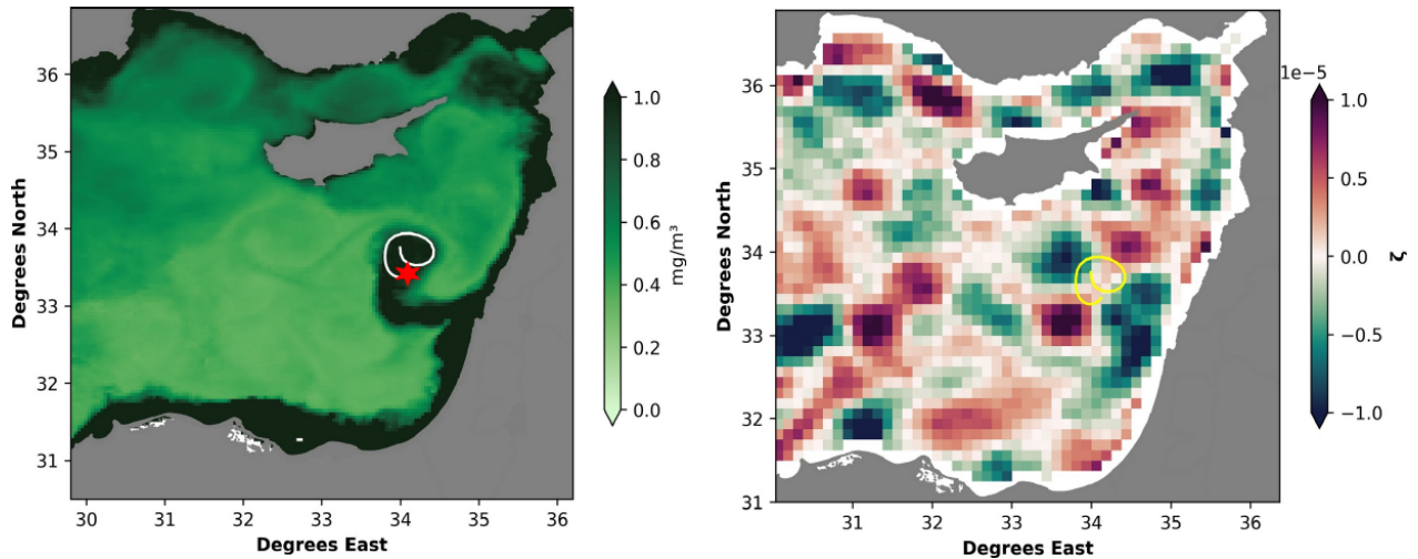
Figure 2. The left panel represents the 8-day average chlorophyll image for the days between 21 st to 28 th of August 2009, while the figure on the right panel represents the relative vorticity average for the corresponding days computed from the altimetry data. Both are overlaid on the trajectory of a drifter corresponding to these days, with the red star representing the the start location of the drifter.
