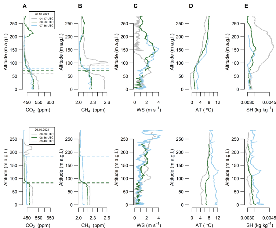
Figure 8. Selected vertical profiles of CH 4 and CO 2 mole fractions, wind speed, air temperature, and specific humidity measured during sampling campaign no. 7 (26.10.2021). Dashed lines on A-B indicate the boundary layer height determined separately for each individual CH 4 and CO 2 vertical profile. Explanations: WS – wind speed, AT – air temperature, SH – specific humidity.
