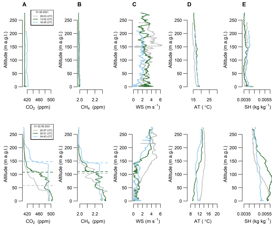
Figure 6. Selected vertical profiles of A) \text{CO}_2 and B) \text{CH}_4 mole fraction, C) wind speed, D) air temperature and E) specific humidity for campaign No. 3 (01-02.06.2021). Dashed lines in A-B indicate the boundary layer height determined separately for each individual \text{CH}_4 and \text{CO}_2 vertical profile. Explanations: WS – wind speed, AT – air temperature, SH – specific humidity.
