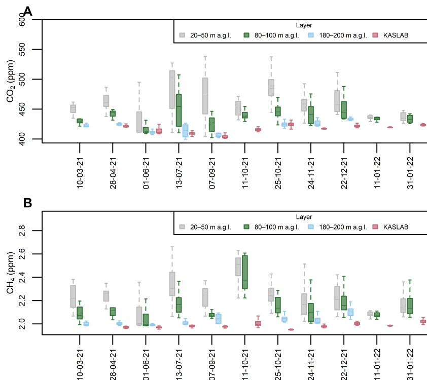
Figure 4. Box-plots of A) CO 2 and B) CH 4 mole fractions measured during flight campaigns at three altitude ranges (20–50 m, 80–100 m, and 180–200 m a.g.l.). The distributions are compared with background concentrations recorded at the KASLAB high-mountain station during the corresponding campaign periods.
