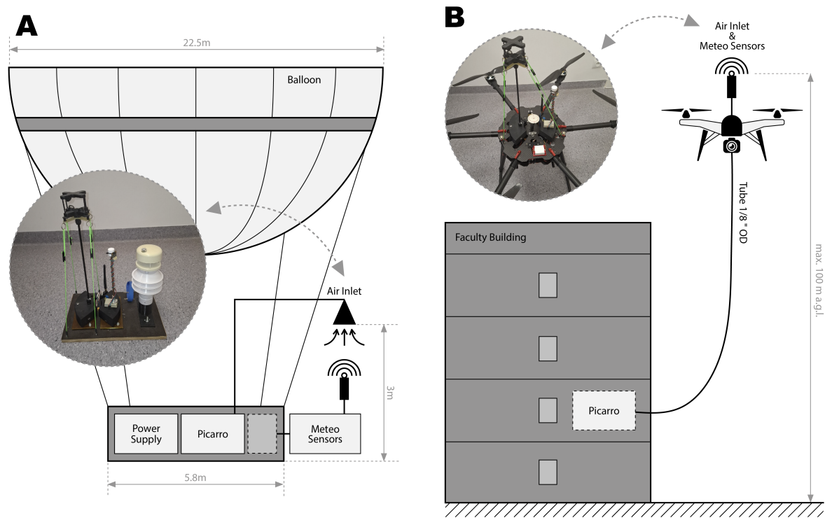
8 Figure 2. Measurement setup for platforms used in the study. A - balloon. B - UAV system.
