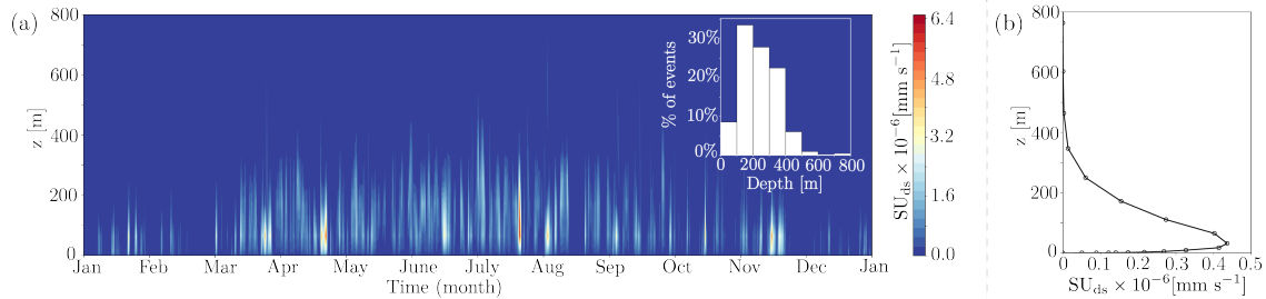
Figure 5. (a) Blowing snow sublimation rate for the year 2011 in \text{mm s}^{-1} , inset shows the histogram of blowing snow layer depth (m). (b) Yearly averaged of blowing snow sublimation rate with height ( \text{mm s}^{-1} ).
