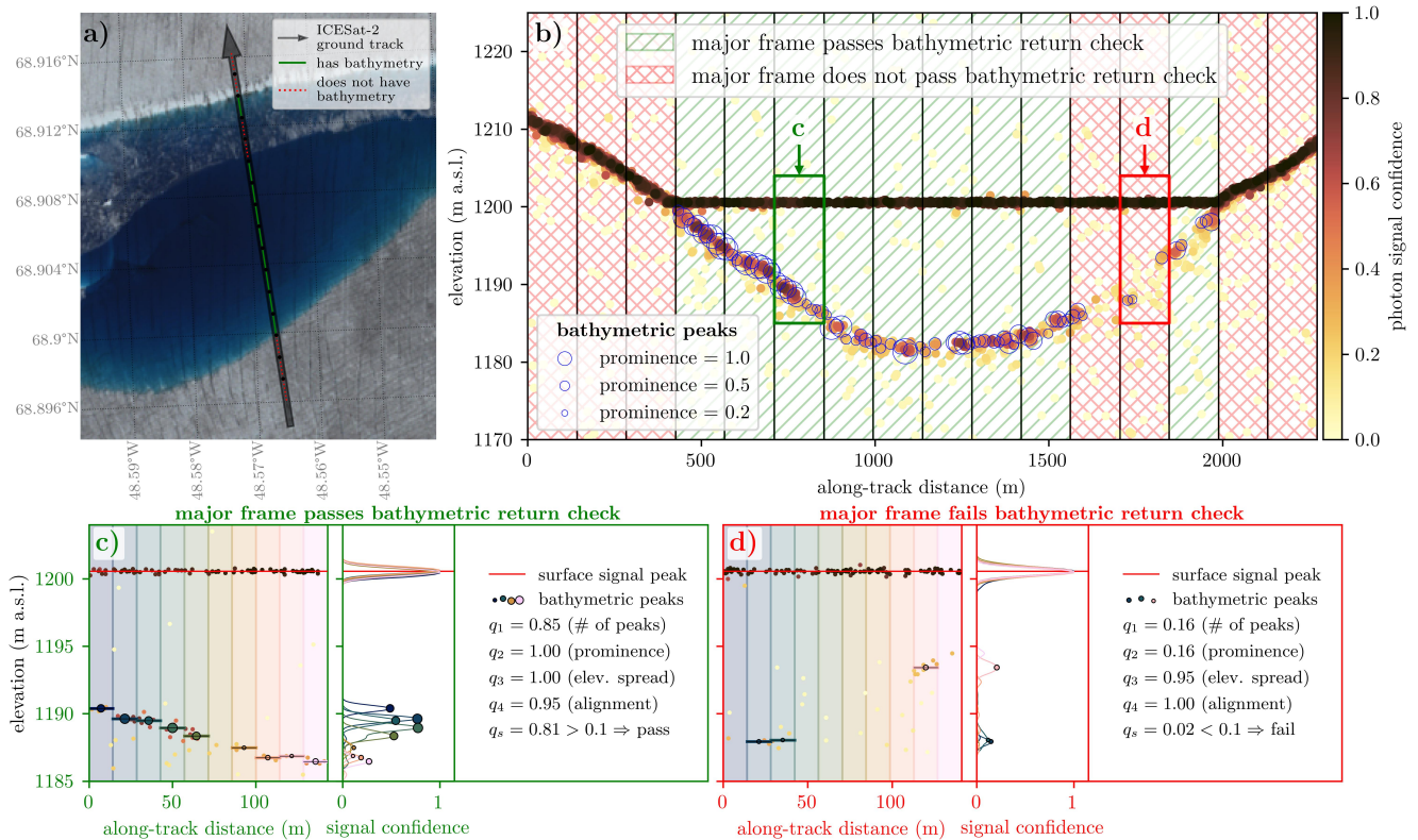
Figure 7. FLUID’s bathymetric signal check run on every ATL03 major frame that has passed the flatness check. a) Ground track for an along-track segment of ATL03 data over the GrIS, which crosses a supraglacial lake that has a thin partial ice cover near its northern shore. b) Corresponding along-track photon elevations, and locations of detected bathymetric photon density peaks. The vertical black lines are the major frame boundaries, and hatching indicates whether major frames passed the bathymetric signal check or not. c) and d) Bathymetric peak-finding procedure from photon density and associated values of the bathymetric return quality heuristics described in the text and defined in Appendix C, for a passing and a failing major frame, respectively. (Data from ICESat-2 Track 277 GT3R on 16 July 2019 and centered at 68.9062° N, 48.5689° W; granule: ATL03_20190716051841_02770403_006_02.h5, imagery: Sentinel-2 on 16 July 2019)
