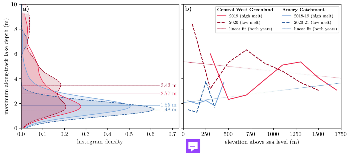
Figure 11. SuRRF lake segment depth statistics for two study regions in high and low melt years. a): Density of maximum lake depth distributions. The numbers shown are median lake segment depths during the corresponding melt season and study region. b): Elevation-binned means of maximum lake segment depths for each season and study region. The dotted lines are the linear fit to all data for the corresponding study region.
