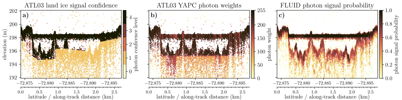
Figure 6. A comparison between existing photons-ATL03 photon signal confidence estimates and our method for melt lakes-lake segments in FLUID. (Data from ICESat-2 Track 81 GT2L on 2 January 2019 and centered at 72.8859° S, 67.3082° E; granule: ATL03_20190102184312_00810210_006_02.h5)
