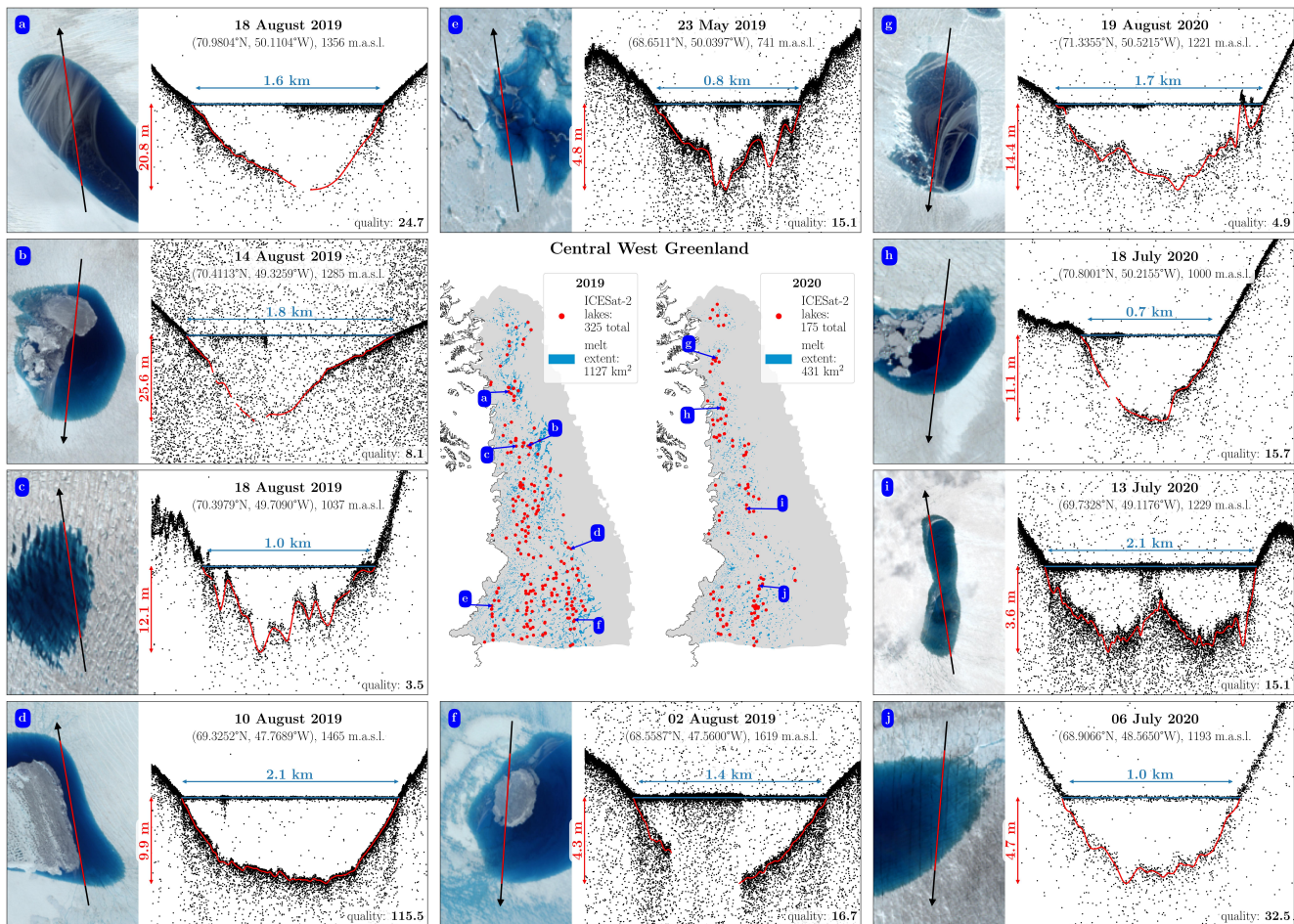
Figure 9. Center maps: FLUID/SURFF-SuRRF algorithm testing in Greenland. Locations of melt lakes-lake segments detected in ATL03 data for the Greenland Ice Sheet’s Central West drainage basin for melt seasons 2019 and 2020, mapped over the corresponding seasons’ maximum meltwater extent from Landsat 8. Panels a-j: Examples showing the underlying ATL03 photon clouds and water depths calculated by SuRRF, for some of the lakes-lake segments shown on the maps. Numbers in lower right of panels are SuRRF-SuRRF lake segment quality scores.
