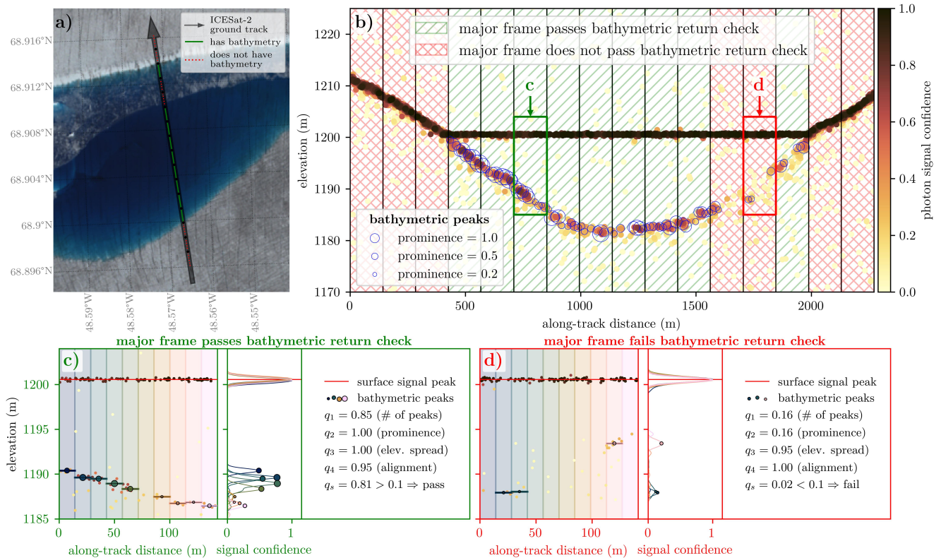
Figure 7. FLUID’s bathymetric signal check run on every ATL03 major frame that has passed the flatness check. a) Ground track for an along-track segment of ATL03 data over the GrIS, which contains crosses a supraglacial lake that has a thin partial ice cover near its northern shore. b) Corresponding along-track photon elevations, and locations of detected bathymetric photon density peaks. The vertical black lines are the major frame boundaries, and hatching indicates whether major frames passed the bathymetric signal check or not. c) and d) Bathymetric peak-finding procedure from photon density and associated values of the bathymetric return quality heuristics defined described in the text and defined in Appendix C , for a passing and a failing major frame, respectively. (Data from ICESat-2 Track 277 GT3R on 16 July 2019 and centered at 68.9062° N, 48.5689° W; granule: ATL03_20190716051841_02770403_006_02.h5, imagery: Sentinel-2 on 16 July 2019)
