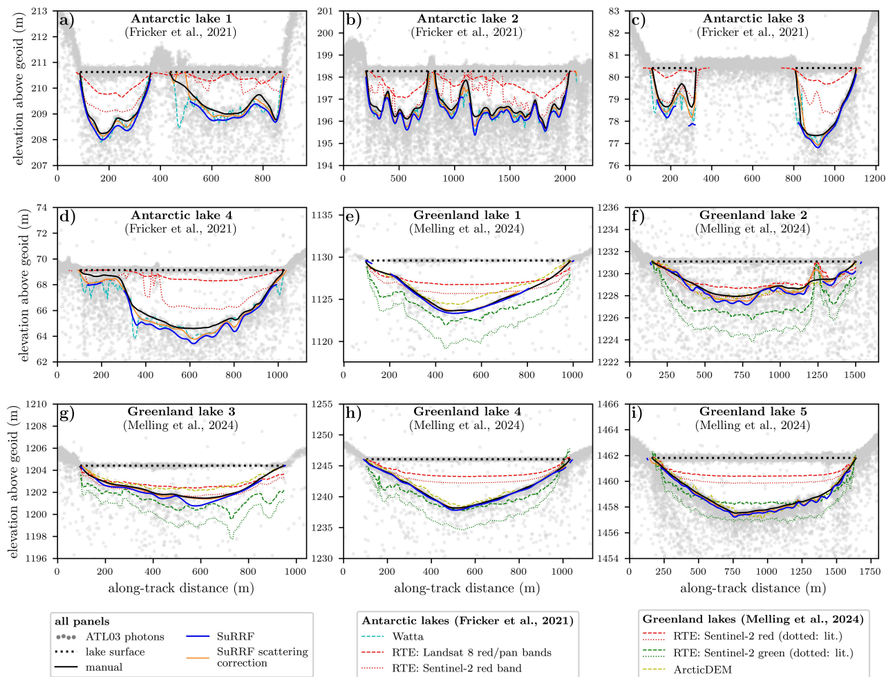
Figure 12. Comparison between SuRRF water depth estimates, manually annotated ICESat-2 depths and results from other methods for meltwater depth estimation for lakes in Antarctica and Greenland. a)-d): ICESat-2 melt lake segments on the Amery Ice Shelf, Antarctica, with manual annotations from Fricker et al. (2021). Other meltwater depth estimates that were reported by Fricker et al. are shown for the Watta algorithm (based on ICESat-2; Datta and Wouters, 2021) and for the RTE method applied to the average of Landsat 8’s red and panchromatic bands (Spergel et al., 2021) and to Sentinel-2’s red band (Moussavi et al., 2020). e)-i): ICESat-2 melt lake segments in Southwest Greenland with manual annotations from Melling et al. (2024). Other meltwater depth estimates that were reported by Melling et al. are shown for the RTE method individually applied to both Sentinel-2’s red and green bands, as well as estimates from post-drainage lakebed topography in ArcticDEM (based on Bowling et al. 2019). SuRRF depth estimates are shown only where the estimated bathymetric signal confidence exceeds 0.5. To align along-track depths with the ATL03 photons (gray dots), the elevations of photons below the water surface elevation of each lake (black dotted lines) were corrected by dividing their vertical distance from the lake’s surface by the refractive index for the speed of light in water.
