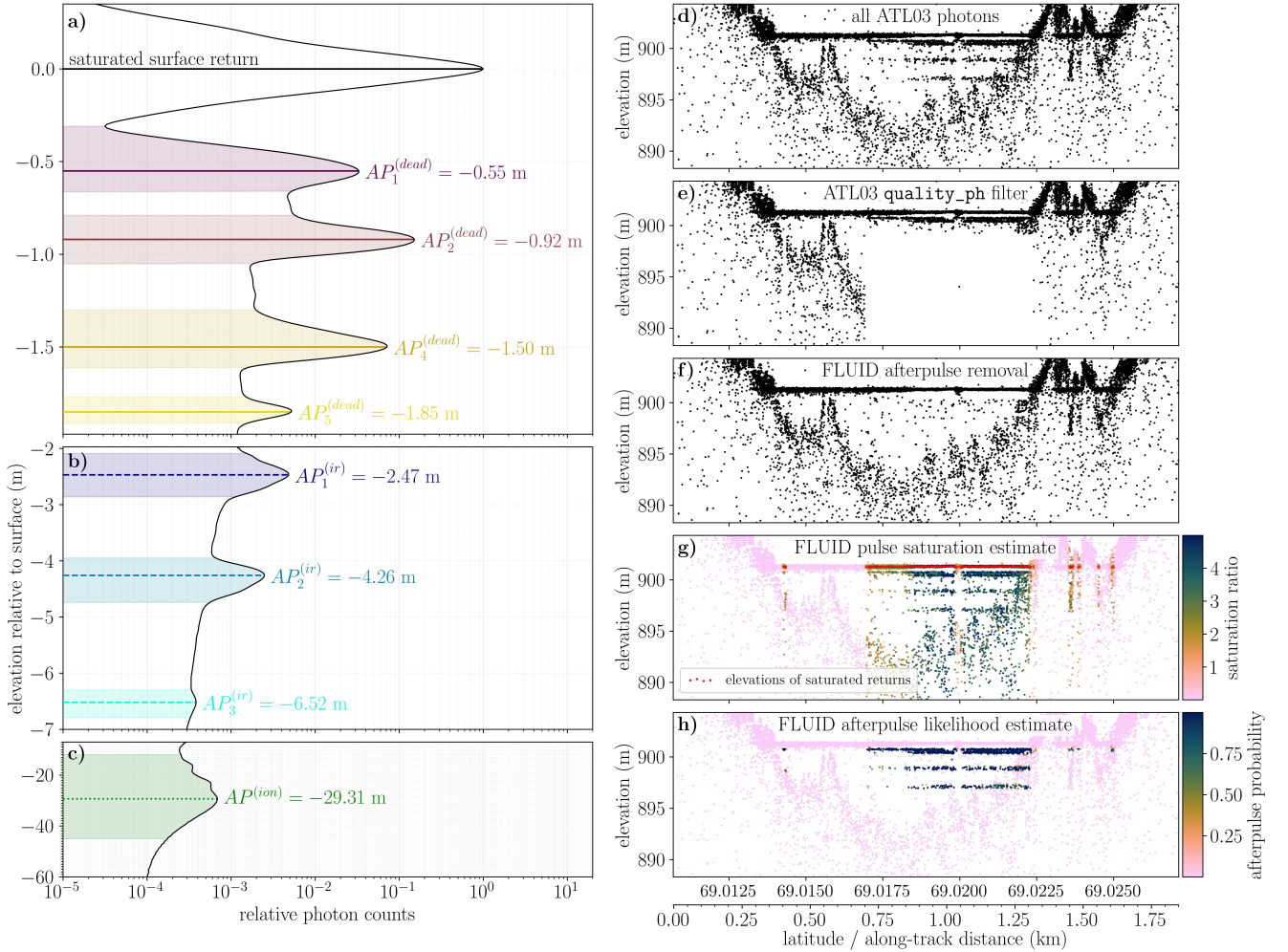
Figure 5. FLUID afterpulse removal. (a) to (c): Histogram of photon elevations in saturated pulses over from ICESat-2 melt lakes segments, relative to the elevation at which saturation occurred. The secondary peaks that appear below the saturated surface return are afterpulses that are caused by (a) dead-time of the ATLAS sensor; (b) internal reflections in the instrument; and (c) PMT ionization. Note that (a), (b) and (c) have different vertical scales. d) to h): Implementation of FLUID’s afterpulse removal for a short along-track segment of ATL03 data that contains crosses a supraglacial lake, with sections of highly saturated (specular) pulses. Known locations of ATLAS afterpulses (a) to (c) are used to remove likely afterpulse photons. (Data from ICESat-2 Track 1222 GT2L on 17 June 2019 and centered at 69.0189° N, 49.0444° W; granule: ATL03_20190617064249_12220303_006_02.h5)
