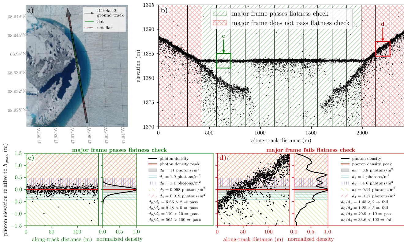
Figure 4. FLUID “flatness check” applied to every ATL03 major frame for identifying potential supraglacial lakeslake segments . a) Ground track of an along-track segment of ATL03 data over the Greenland Ice Sheet, with crossing a partially ice-covered supraglacial lake; b) Corresponding along-track photon elevations, with major frame boundaries marked by vertical black lines and flatness check outcomes shown in hatching; c) and d) Photon density ratios for a passing and a failing segment, respectively. (Data from ICESat-2 Track 216 GTIL on 12 July 2019 and centered at 68.9370° N, 47.9657° W; granule: ATL03_20190712052659_02160403_006_02.h5, imagery: Sentinel-2 on 13 July 2019)
