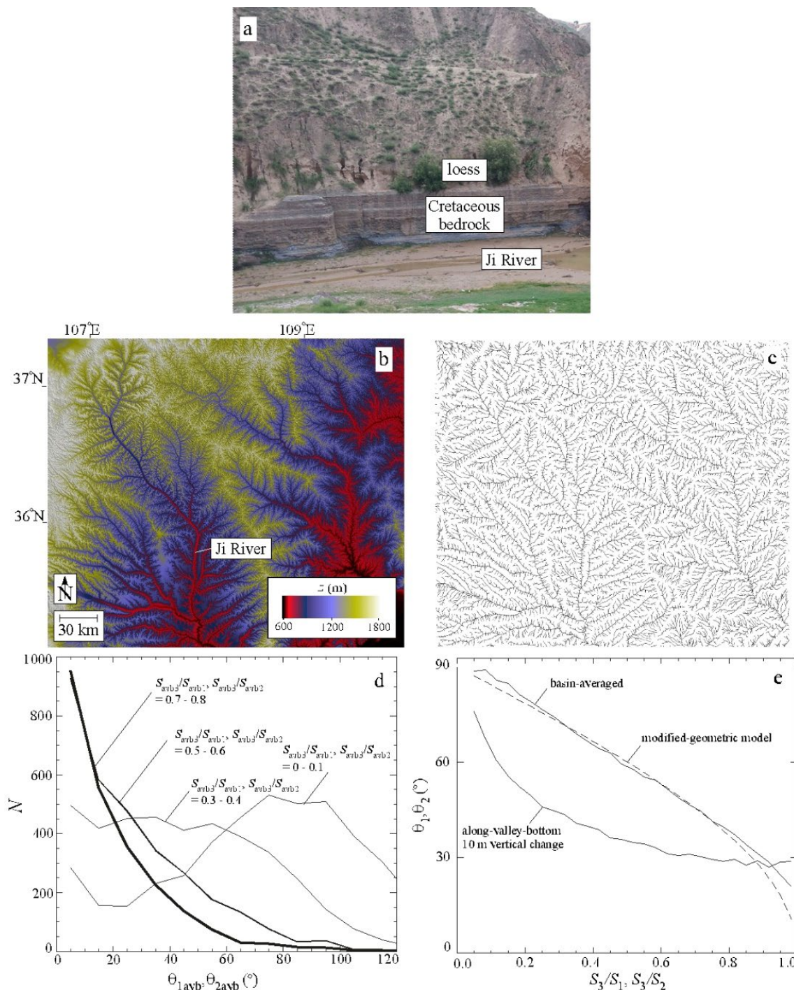
435 Figure 9: Results of the junction extraction for a portion of the Loess Plateau region of China. (b) Color map of topography. (c) Valley bottom network extracted for the study area. (d) Plot of histograms of AVB junction angles for four ranges of slope ratios. (e) Plot of junction angles as a function of slope ratios for both BA and AVB properties.
