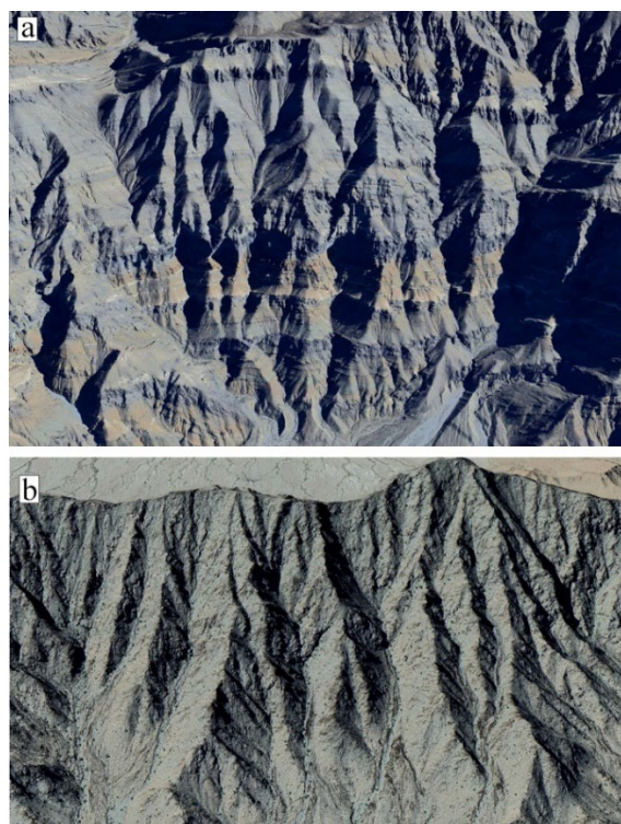
Figure 13: Oblique aerial photographs of portions of subparallel drainage networks incised into bedrock in (a) sedimentary rocks of the Lost Chance Range, California, and the granite and schist of the Mohawk Mountains, Arizona.
