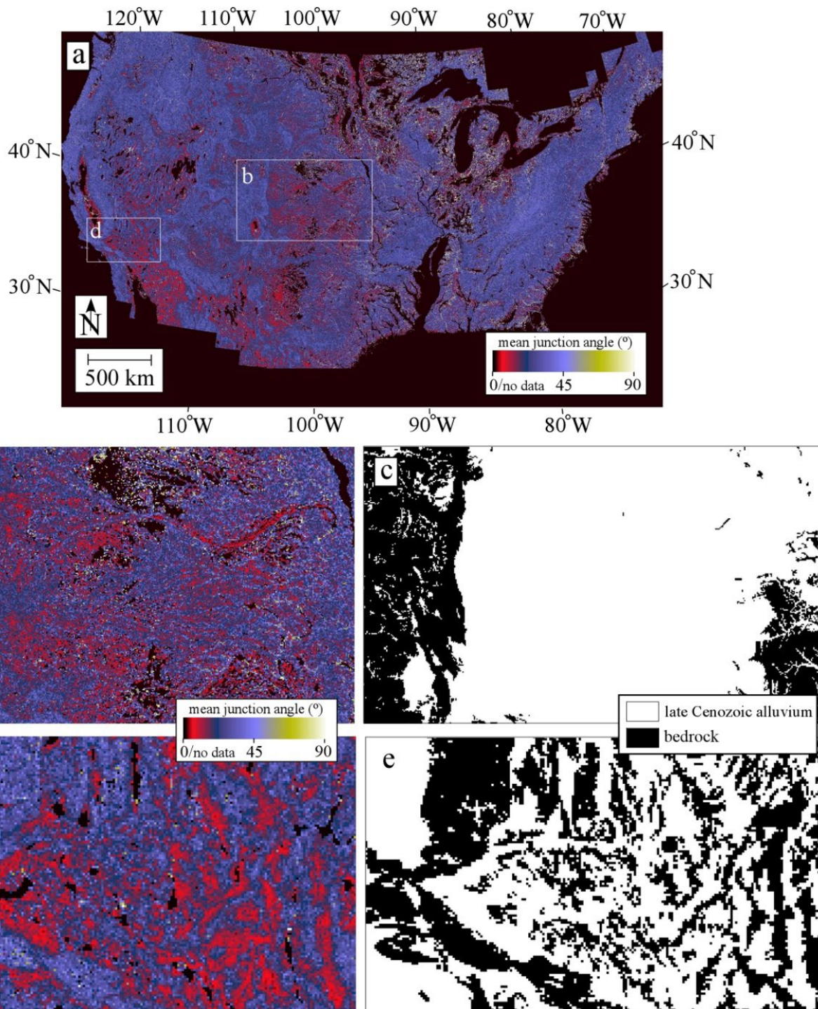
465 Figure 11: Color maps of junction angles averaged for every 2.5 x 2.5 km in the conterminous U.S.A. Junction angles tend to be lower in areas with late-Cenozoic deposits of (b)&(c) the Great Plains and (d)&(e) the Basin and Range province of the southwestern U.S.A.
