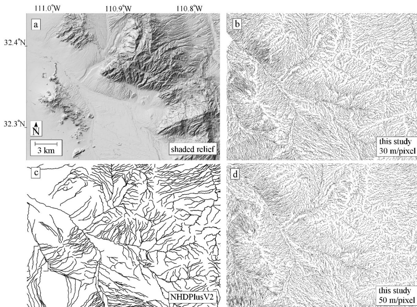
330 Figure 6: Comparison of the tributary fluvial valley bottom networks for the larger Tucson region. (a) Shaded-relief image of the 30 m pixel -1 National Elevation Dataset (NED). Fluvial valley networks obtained in this study using (b) 30 m pixel -1 NED data, (c) the NHDPlusV2 data (McKay et al., 2012), and (d) using 50 m pixel -1 DEM data.
