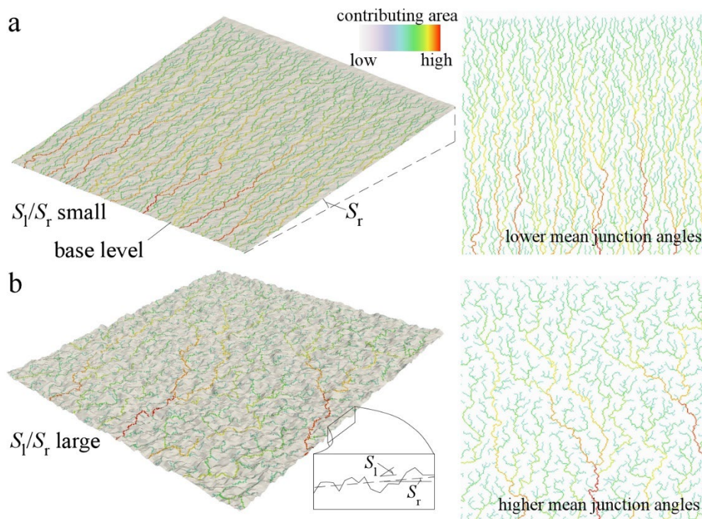
115 Figure 2: Conceptual illustration of how differences in the ratio of microtopographic amplitude (quantified by the root-mean-squared variation in local slope, S_l ) to the large-scale or regional slope, S_r , may control fluvial network junction angles. The landforms illustrated in both (a) and (b) have small-scale random microtopography superimposed on a planar tilted slope. The flow patterns defined by contributing area were determined by hydrologic correction and the steepest-descent routing algorithm. Landforms with a lower S_l/S_r (shown in a) result in more parallel fluvial valleys compared to landforms with a higher value of S_l/S_r (shown in b). The specific examples in this figure are ours but the concept closely follows Castellort and Yamato (2013).
