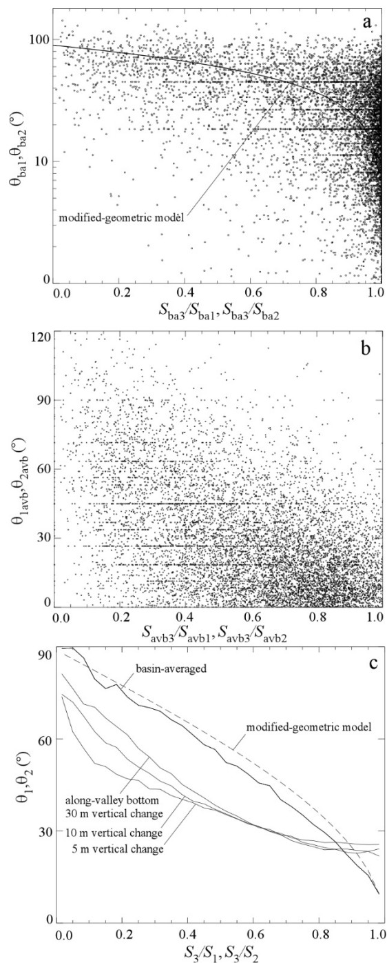
Figure 8: Plots illustrating the relationships of junction angles to the ratios of slopes downslope and upslope of the junctions for the portion of southern Arizona illustrated in Figure 5. (a) Plot of junction angles measured using BA properties as a function of the ratio of slopes downslope and upslope. (b) Plot of junction angles measured using AVB properties as a function of the ratio of slopes downslope and upslope. (c) Plots of junction angles measured both AVB (using three different values of the elevation change over which slopes and orientations are computed) and BA properties.
