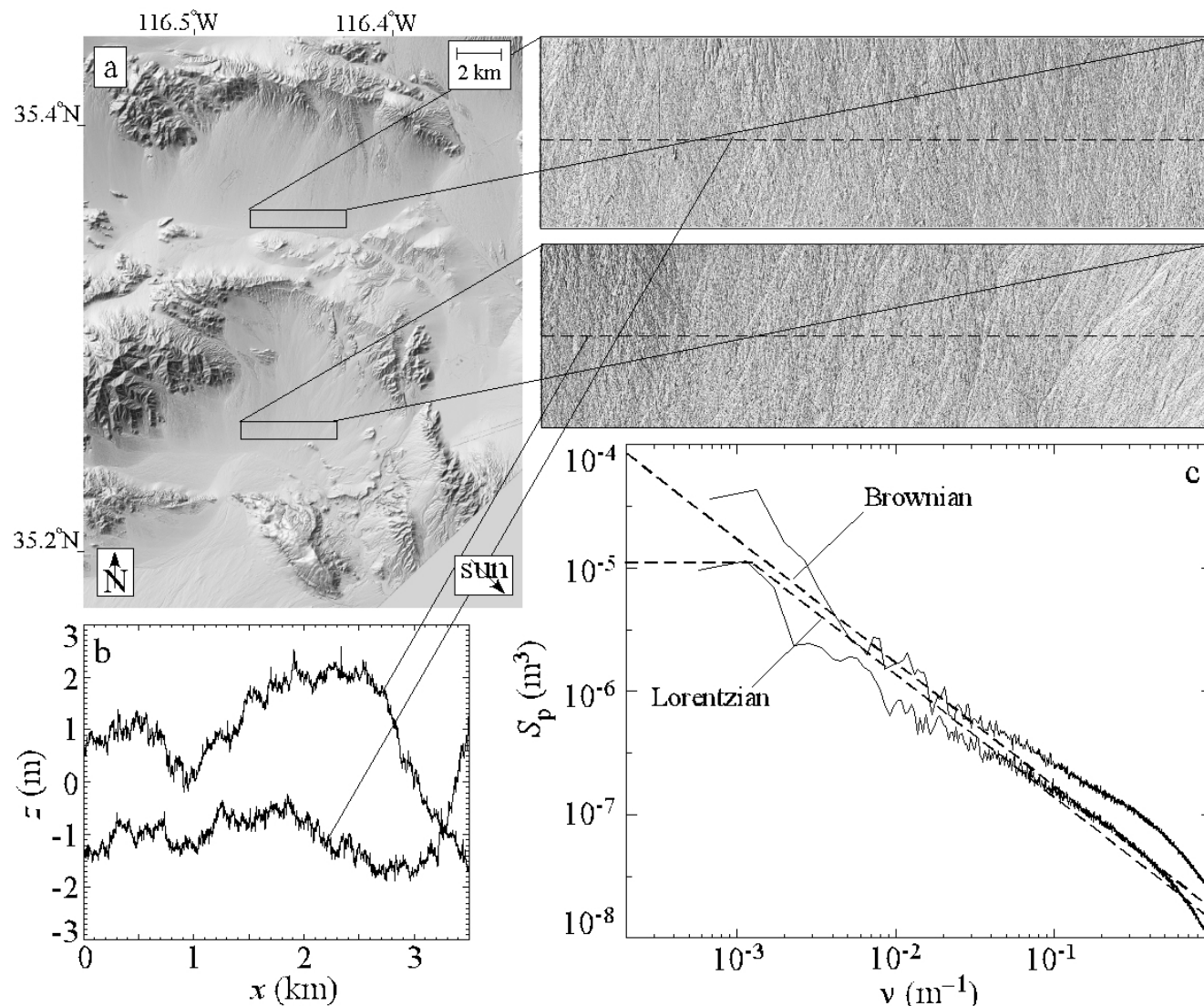
310 Figure 5: Quantification of the power-spectral properties of example Holocene alluvial piedmonts in the Ft. Irwin region of eastern California. (a) Shaded relief image of example areas with zoom-in on transects shown on graphs. (b) Elevation, z , versus distance, x , of example transects. (c) Plot of the power spectrum, S_p , as a function of the natural wavenumber, v , for the landforms in (a). Also plotted are the power spectra associated with a Brownian walk and a Lorentzian, i.e., a Brownian walk that transitions to a constant spectrum at low wavenumbers.
