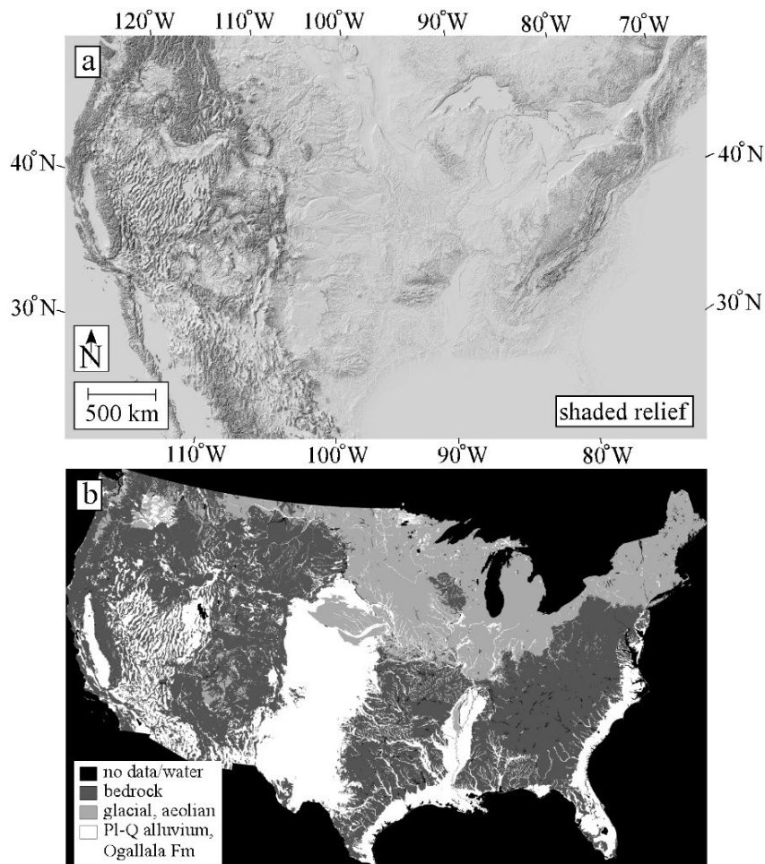
450 Figure 10: (a) Shaded relief map of the conterminous U.S.A. in Lambert conformal conic projection. (b) Surficial geologic map of the conterminous U.S.A. (Soller et al., 2009) simplified to three units.
