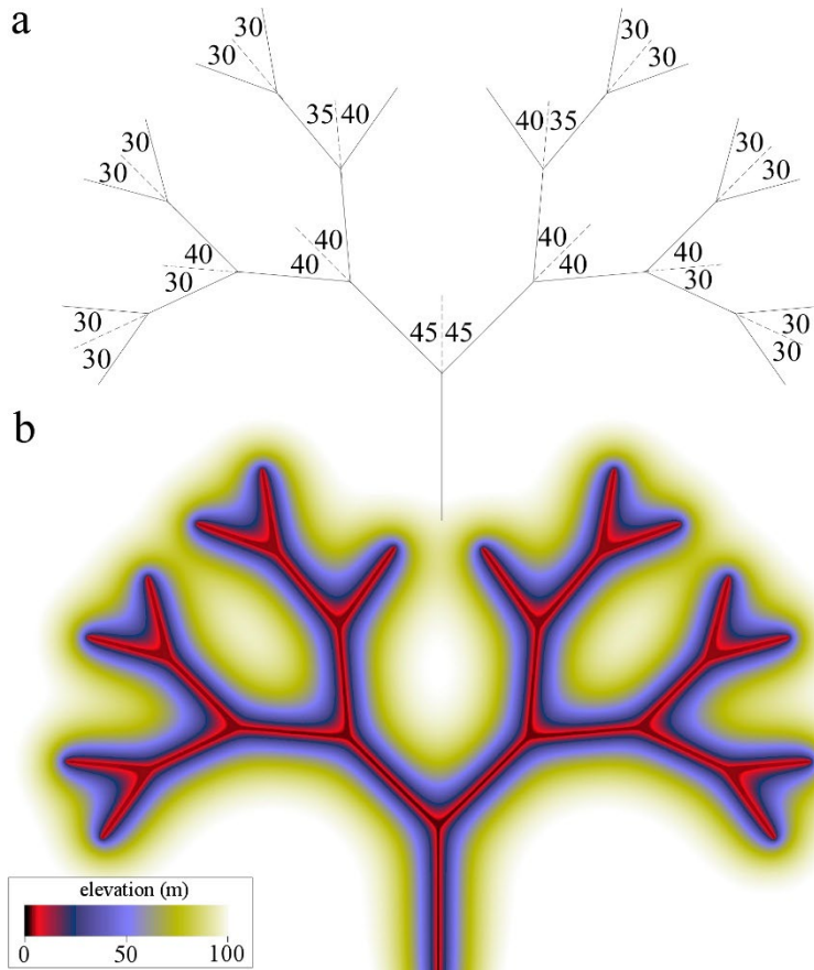
275 Figure 4: Images of the idealized branching network used to test the junction-angle-extraction algorithm. (a) network, illustrating examples of the three types of junction angles present in the network. (b) Color map of the topography of the synthetic landform.
