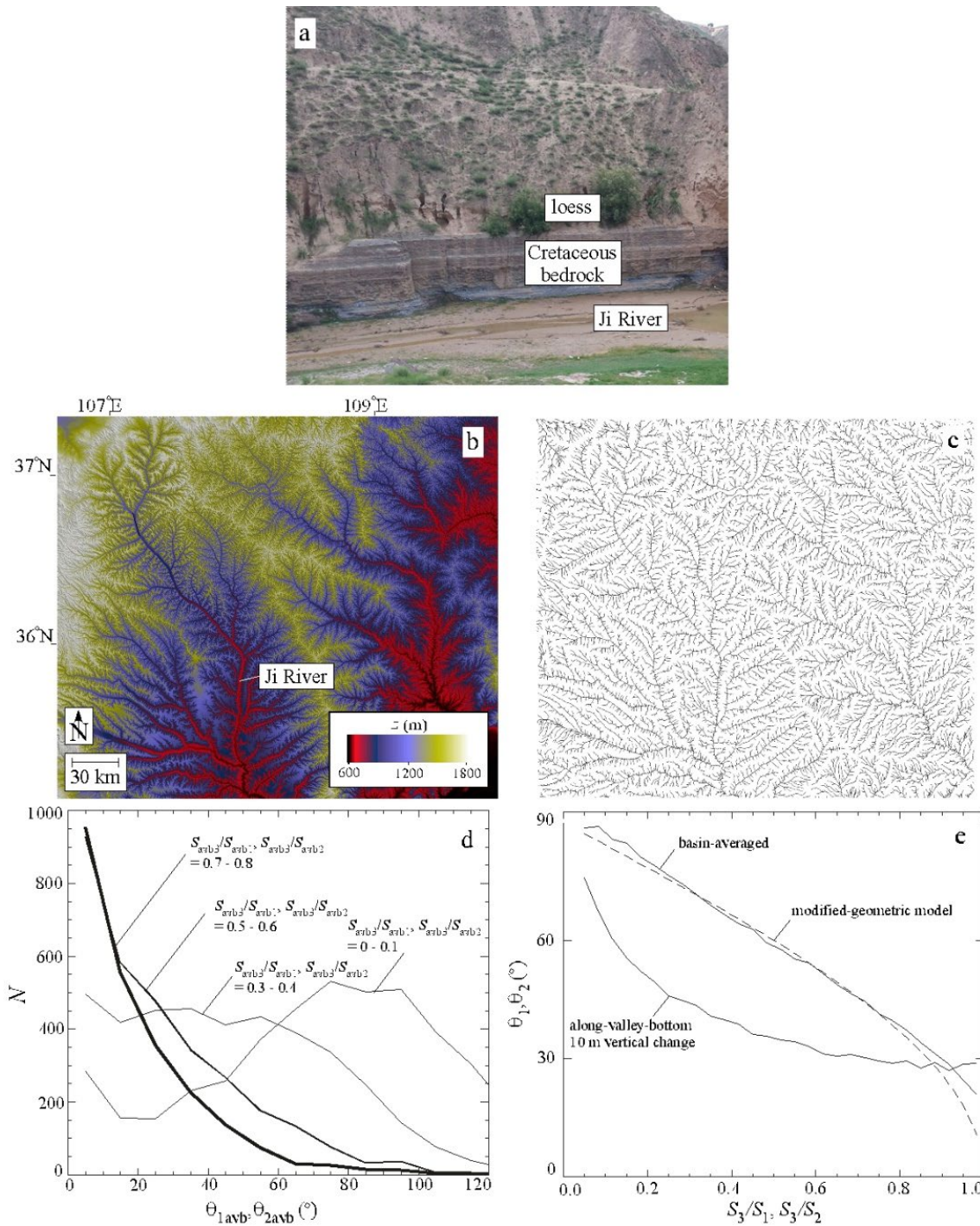
450 Figure 9: Results of the junction extraction for a portion of the Loess Plateau region of China. (b) Color map of topography. (c) Valley bottom network extracted for the study area. (d) Plot of histograms of AVB junction angles for four ranges of slope ratios. (e) Plot of junction angles as a function of slope ratios for both BA and AVB properties.
