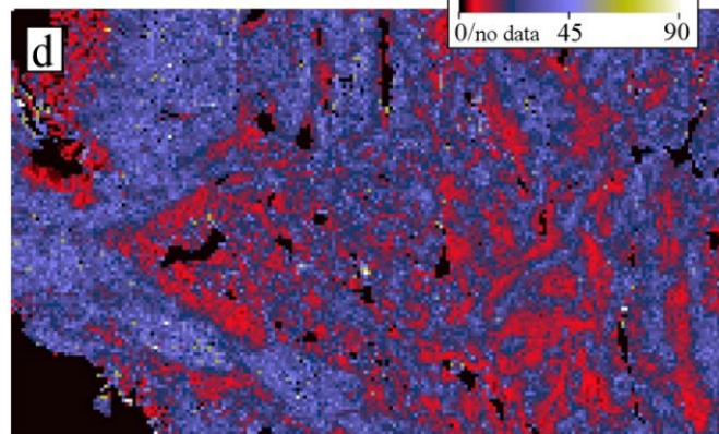
Figure 11: Color maps of junction angles averaged for every 2.5 x 2.5 km in the conterminous U.S.A. Junction angles tend to be lower in areas of late-Cenozoic alluvial piedmont deposits of (b)&(c) the Great Plains and (d)&(e) the Basin and Range province of the southwestern U.S.A.
