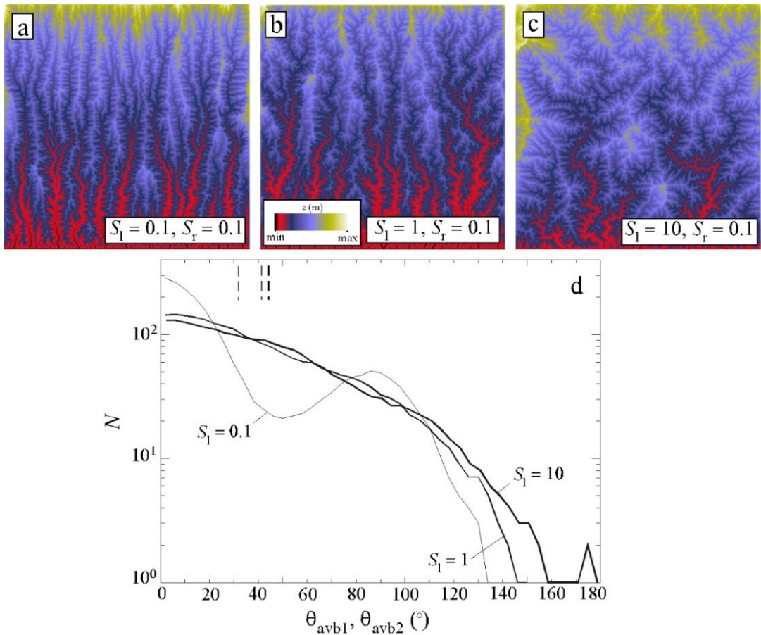
540 Figure 13: Results of landscape evolution models using the landscapes whose fluvial networks are illustrated in Figs. 12a-12c as initial topographies. (a)-(c) Color maps of steady-state landscapes. (d) Plot of histograms of junction angles extracted from the landscapes in (a)-(c).
