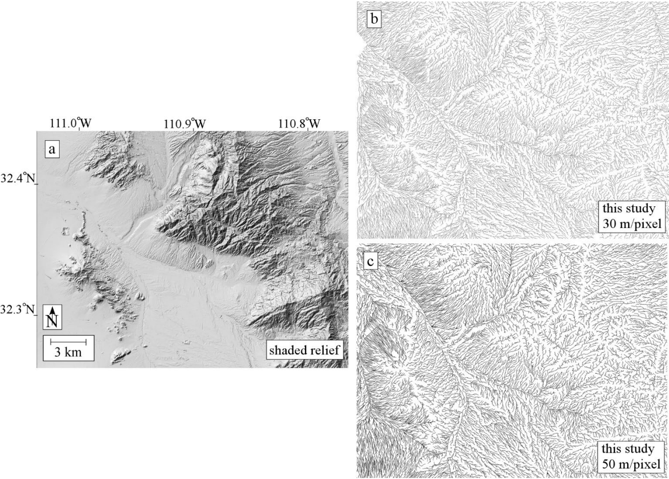
345 Figure 6: Comparison of the tributary fluvial valley bottom networks for the larger Tucson region. (a) Shaded-relief image of the 30 m pixel -1 National Elevation Dataset (NED). Fluvial valley-bottom networks obtained in this study using (b) 30 m pixel -1 NED data and (c) using 50 m pixel -1 NED data.
