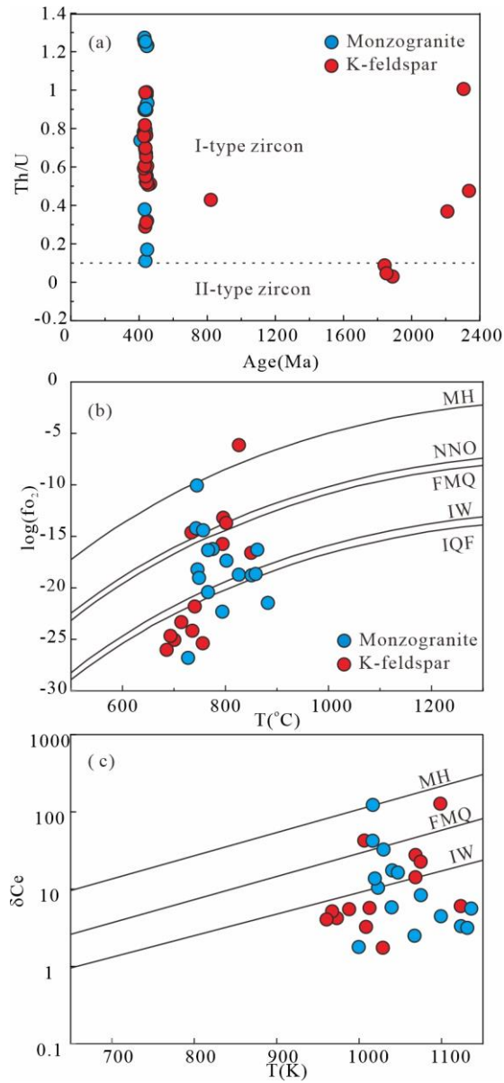
Figure 7 Age-Th/U (a), T-log(fO 2 ) (b) and T-δCe (c) diagrams of zircon
