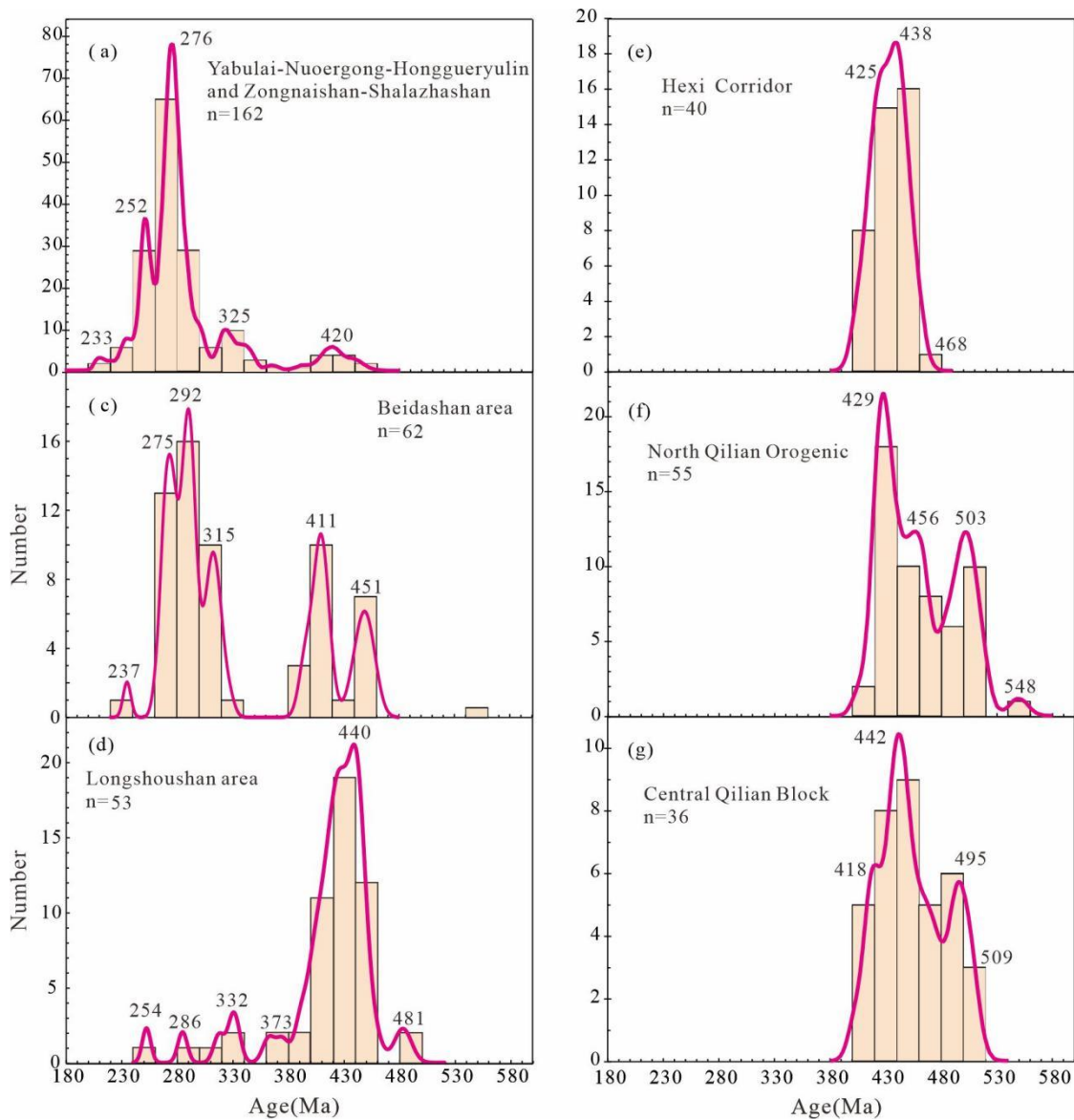
395 Figure 12 Kernel density estimate (KDE) plots for Palaeozoic and Mesozoic magmatic ages in the Alxa Block, North Qilian Belt and Central Qilian Block. Ophiolitic rocks are not included. Data are in Supplementary materials Table S1. All dates are zircon U-Pb ages (histogram bin width is 20).
