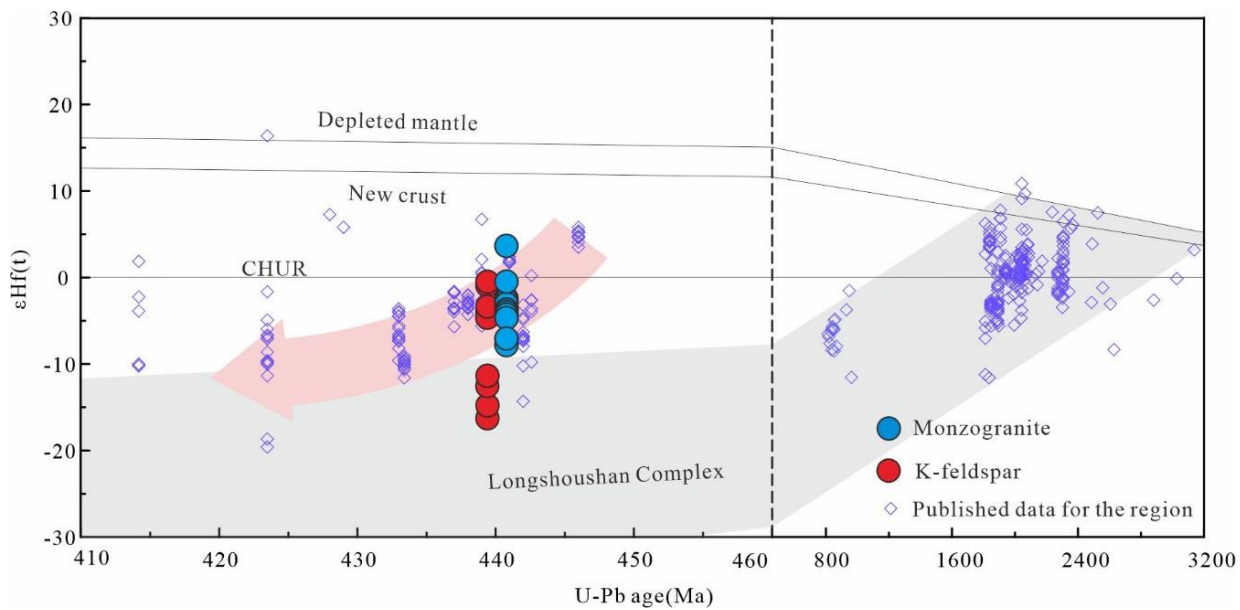
335 Figure 10 Zircon \epsilon_{\text{Hf}}(t) -age (Ma) diagram for samples in this study and published data for the region. The source of the published data can be found in Supplementary materials Table S1 (The red arrow represents the variation trend of \epsilon_{\text{Hf}}(t) ).
