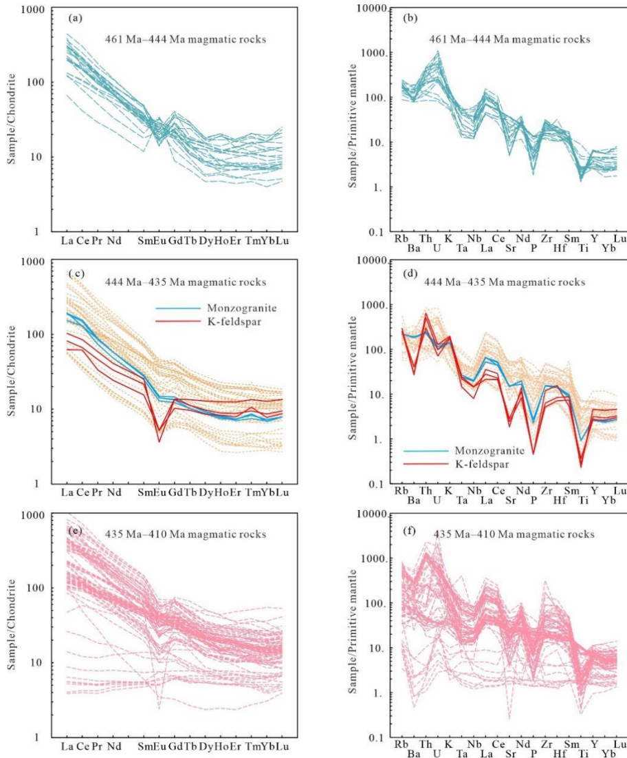
Figure 5 Chondrite-normalized REE patterns and primitive mantle-normalized trace element patterns for Early Paleozoic magmatic rocks (chondrite and primitive mantle values are from Sun and McDonough, 1989). The source of the published data can be found in Supplementary materials Table S1.
