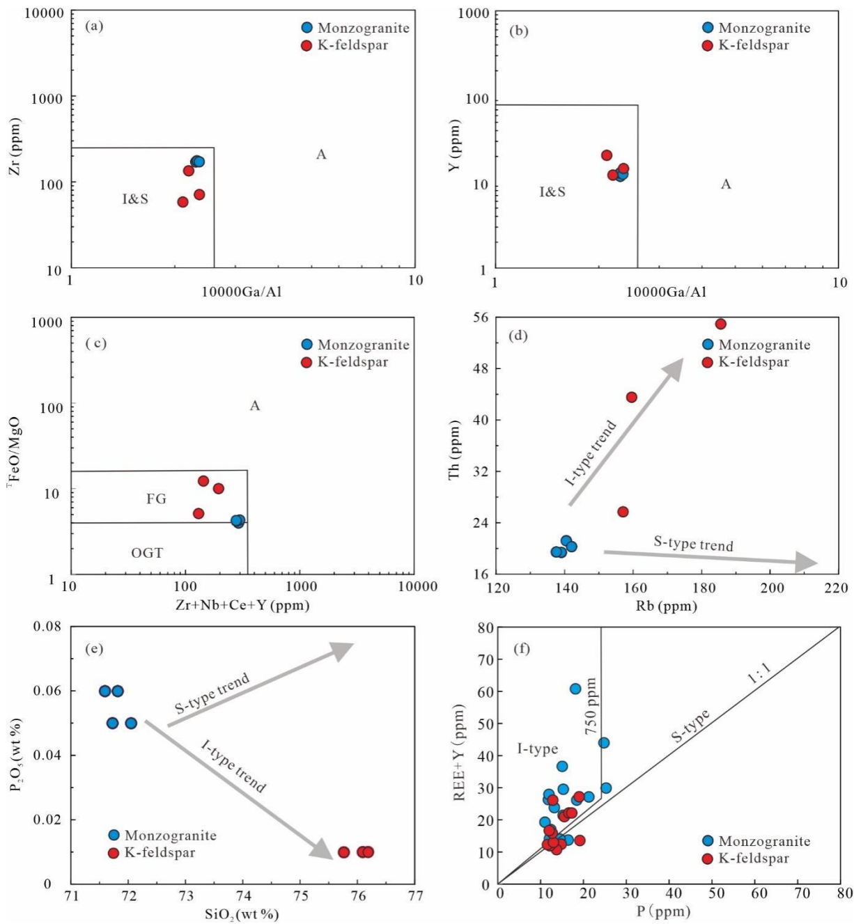
295 Figure 8 Discrimination diagram of granitoid genetic types. (a, b, c) 10000 Ga/Al vs. Zr, 10000 Ga/Al vs. Y and Zr+Nb+Ce+Y vs. TFeO/MgO (after Whalen et al., 1987); (d) Rb vs. Th; (e) SiO 2 vs. P 2 O 5 ; (f) P vs. REE+Y (after Burnham and Berry, 2017).
