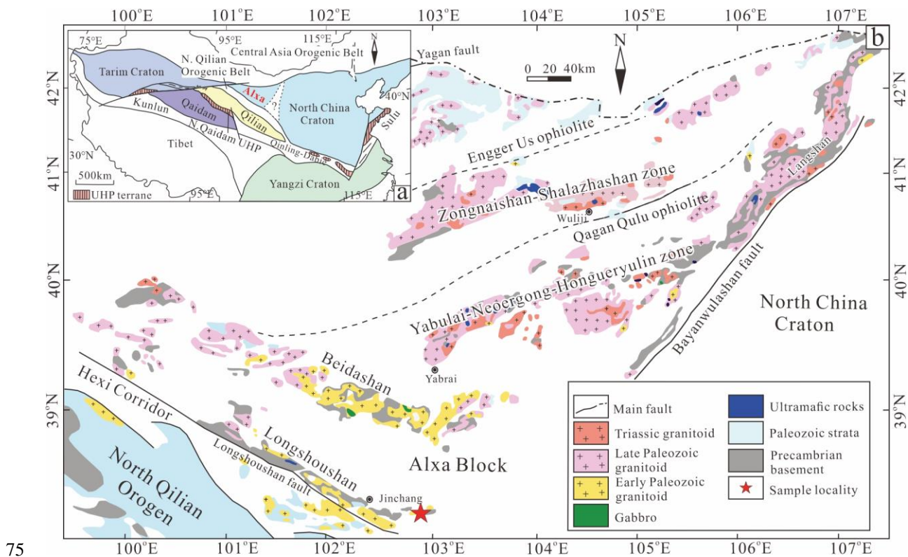
Figure 1 (a) Sketch geological map showing the tectonic location of the Alxa Block (modified from Song et al., 2013). (b) Simplified geological map of the Alxa Block Phanerozoic granitoids (modified from Zheng et al., 2014; Hui et al., 2021). AB- Alxa Block; CQB- Central Qilian Block; NCC- North China Craton.
