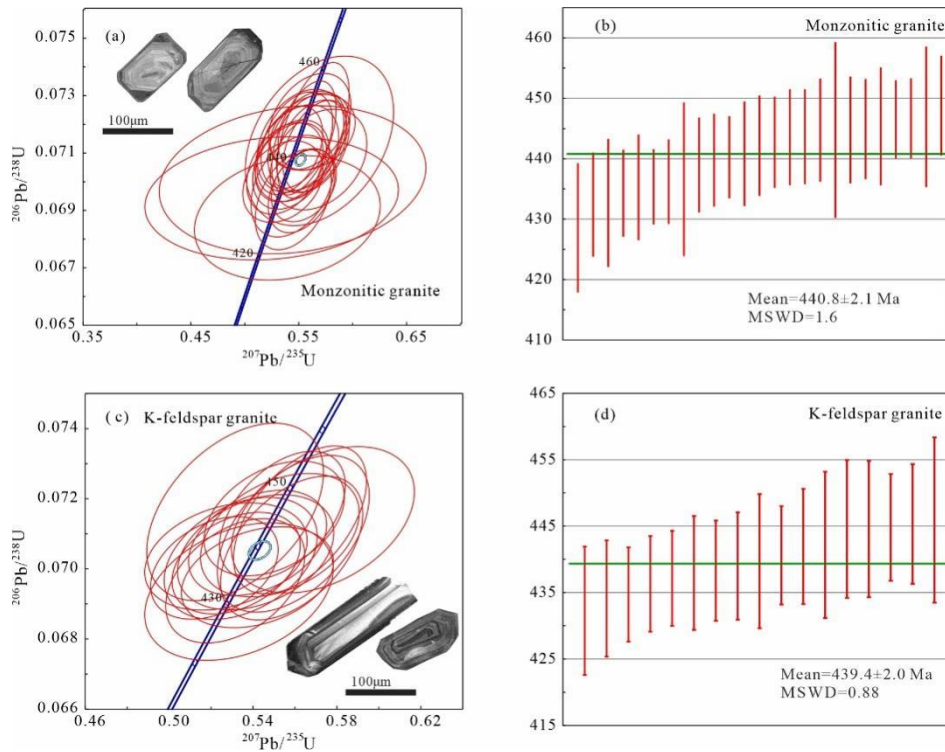
Figure 6 Concordia diagrams for zircon LA-ICP-MS U-Pb analyses.
