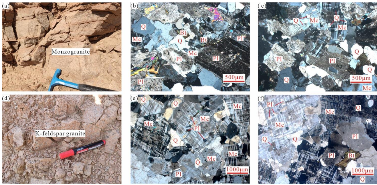
Figure 3 Field photographs and photomicrographs of monzogranite (a, b, c) and K-feldspar granite (d, e, f) (b, c, e, f-perpendicular polarized light). Q-quartz; Kfs-feldspar; Pl- plagioclase; Mc-Microcline; Bt-biotite.
