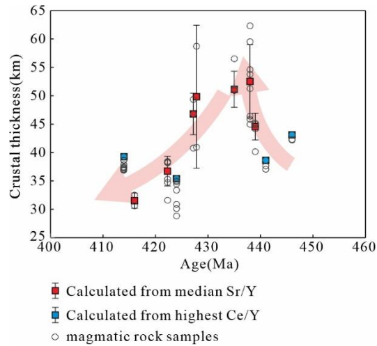
430 Figure 13 Plot of crustal thickness versus age of magmatic rocks for each data subset in the Longshoushan, southwestern Alxa Block. Data are in Supplementary materials Table S1.
