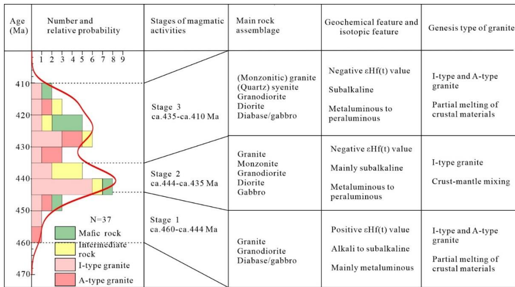
Figure 14 Integrated column of magmatism evolution of Early Paleozoic in the Longshoushan area. On the left is the histogram of age distribution of Early Paleozoic magmatic rocks in the Longshoushan area. Data are in Supplementary materials Table S1
