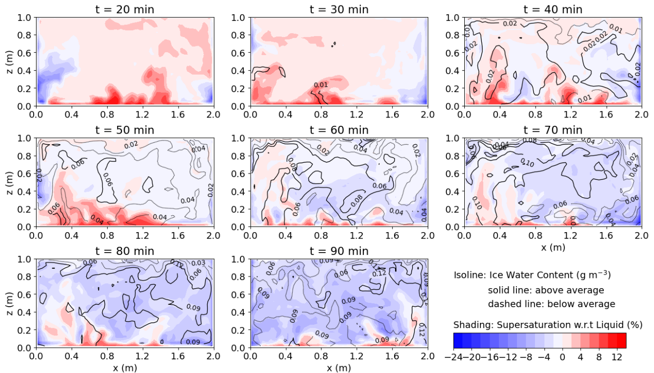
Figure 6. The ice mass concentration (represented by isolines; unit: \text{g m}^{-3} ) where solid lines indicate above-average values, and dashed dotted lines indicate below-average values, alongside supersaturation with respect to liquid (indicated by shading), observed at the end of each time period. Red shading represents supersaturation, while blue shading indicates subsaturation. For clarity of the isolines, the increments are 0.01, 0.02, and 0.03 \text{g m}^{-3} for the first row ( t = 20\text{--}40 min), second row ( t = 50\text{--}70 min), and third row ( t = 80\text{--}90 min), respectively.
