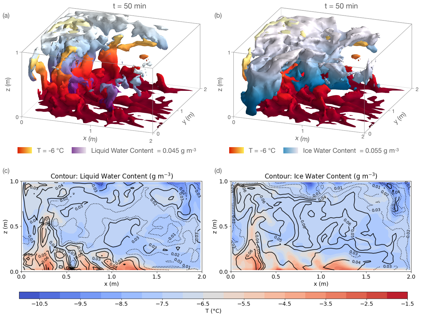
Figure 3. A snapshot at t = 50 min showing the large-scale circulation and its effect on the distribution of flow properties within the chamber. The 3D isosurfaces (a–b) depict warm air isosurface of at T = -6^\circ\text{C} (the red-to-yellow color in panels (a) and (b)), liquid water content isosurface [the purple-to-white color in panel (a)], and ice water content isosurface [the blue-to-white color in panel (b)] at t = 50 min. Gradient colors represent different heights, with lighter colors indicating distance closer to the chamber top, to enhance the three-dimensional 3D visualization. The isosurfaces are opaque, causing some warm air isosurfaces to be obscured by the liquid water and ice crystal isosurfaces. The central slices of panels a–b at y = 1 m are displayed in panels c–d, respectively, with shading indicating temperature and contour lines representing liquid water content (c) or ice water content (d). The solid contour lines indicate above-average values, and dotted contour lines indicate below-average values.
