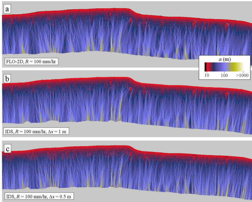
470 Figure 7: Color maps of specific contributing area, a (m), for the hillslope pictured in Figure 1a as predicted by (a) FLO-2D and IDS using DEMs of different resolutions: (b) \Delta x = 1 m and (b) \Delta x = 0.5 m. All results correspond to R = 100 mm hr -1 .
