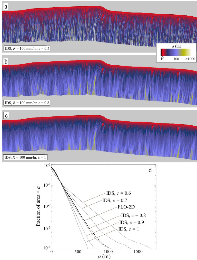
Figure 8: (a)-(c) Color maps of specific contributing area, a (m), for the hillslope pictured in Figure 1a as predicted by IDS for different values of the parameter c quantifying the weighting of the local grid point relative to the downslope grid point. (a) c = 0.5 , (b) c = 0.8 , (c) c = 1 . (d) Cumulative frequency-size distribution of specific contributing area, a (m), for a range of values of c and for the results of FLO-2D.
