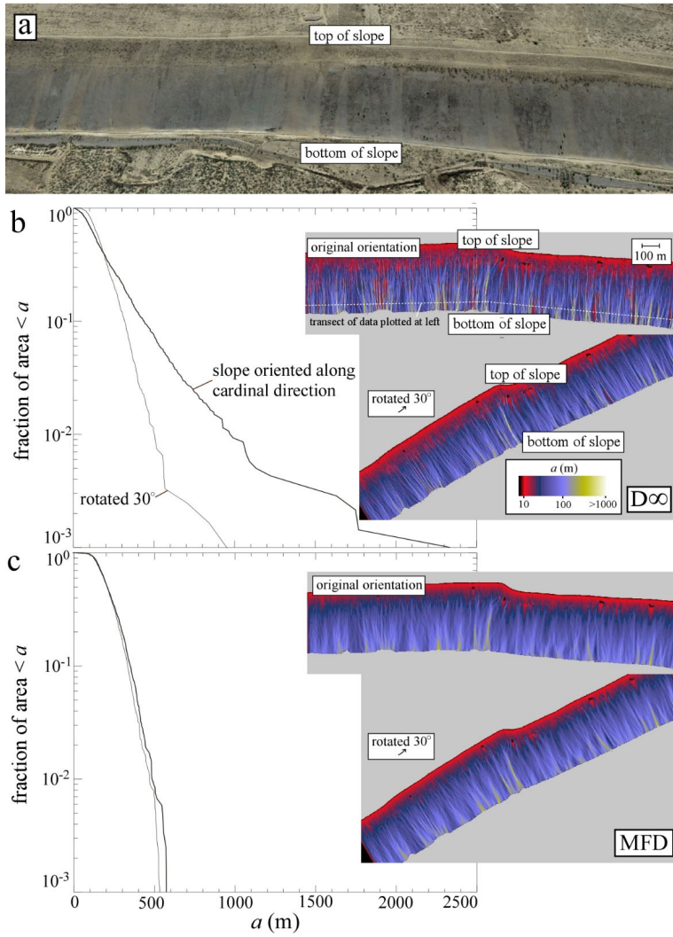
155 Figure 14: Dependence of the specific contributing area, a (m), predicted by (b) D_\infty and (c) MFD on the relative orientation of the hillslope to the cardinal and ordinal directions of the grid. (a) The monitored hillslope in Pinal County, AZ, USA, that motivated this work. (b) Rotating the hillslope by 30° results in more than a factor-of-two of difference in predicted a values using D_\infty . (c) The same rotation has almost no effect with MFD.
