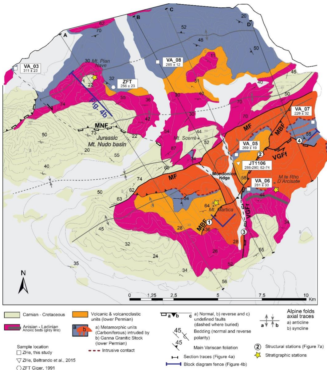
Figure 3: Geological map of the Study area (modified after Scaramuzzo et al., 2022). ZHe: zircon (U-Th)/He; ZFT: zircon fission-track. Fault codes: MF, Marzio Fault; MBF, Martica - Boarezzo Fault; VGFr, Valganna Fault ramp segment; VGff, Valganna Fault flat segment. The Mt. Nudo basin is Jurassic in age (Kalin and Trumpy, 1977).
