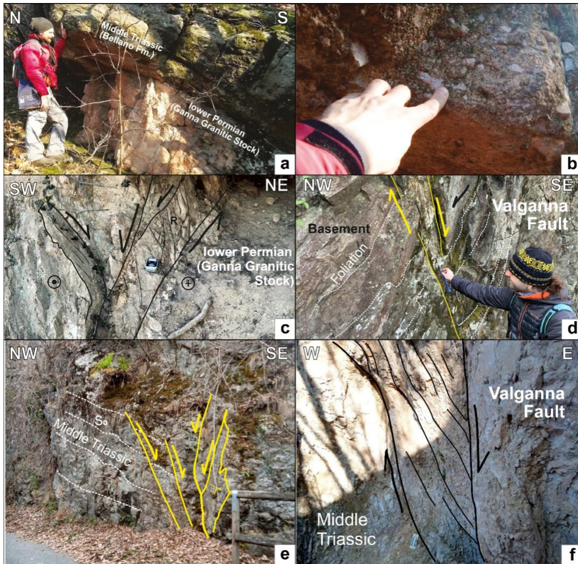
315 Figure 6: a) middle Permian unconformity highlighted by the contact between the lower Permian Ganna Granitic Stock and the Anisian Bellano Fm.; b) detail of the base of the Bellano Fm.; c, d, e, f, mesoscopic structural features of Valganna Fault (c, d, e, f).
