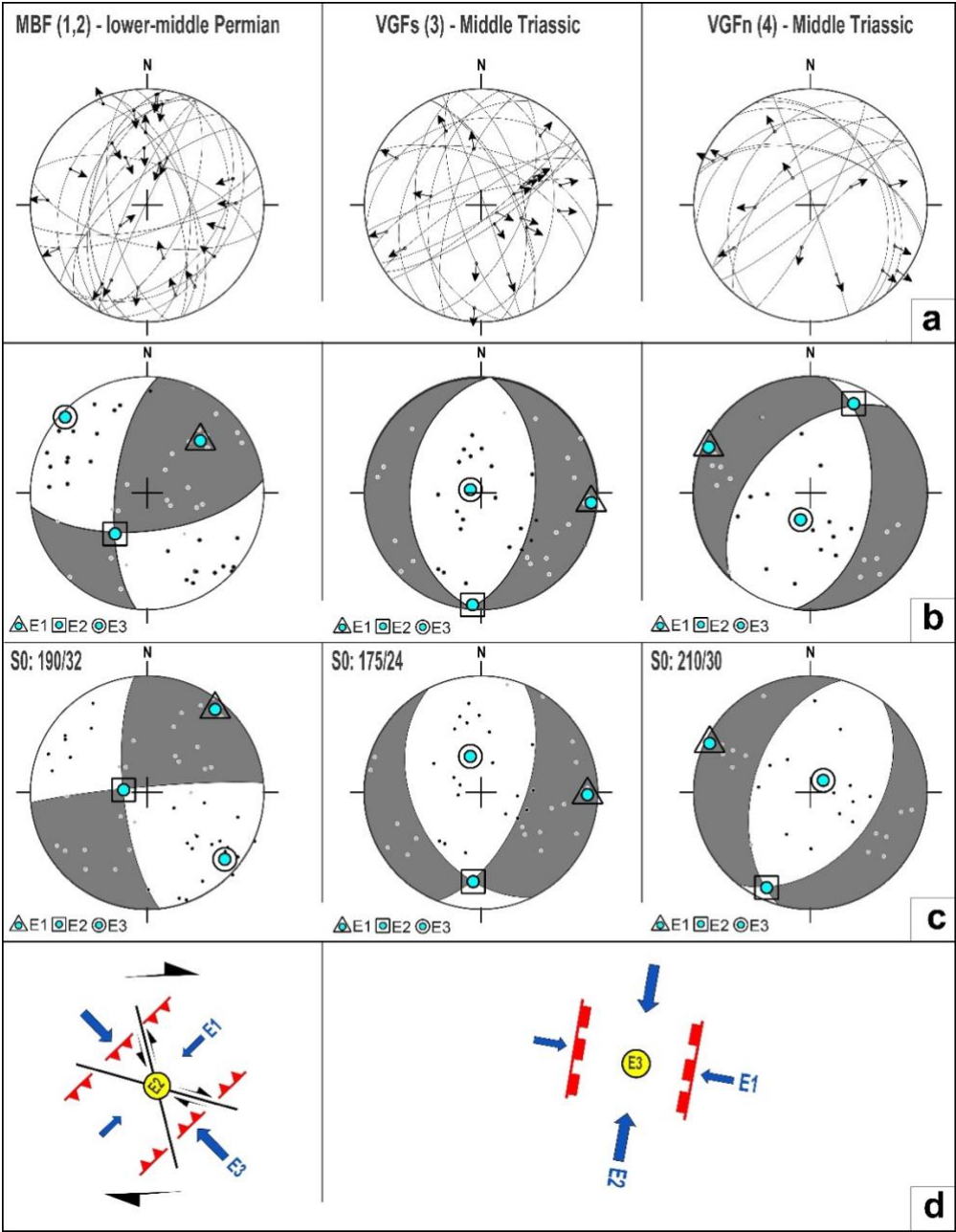
325 Figure 7: Fault slip data and inversion: a) fault slip data along the faults described in the text (see Figure 3 for the location of the structural stations); b) kinematic inversion, P and T axes and the best fit fault plane solutions are represented; c) kinematic inversion after restoration to the nearest bedding orientation (S0); Codes: MBF: Martica-Boarezzo Fault; VGf: Valganna Fault – ramp segment; VGfn – Valganna Fault – flat segment; d) schematic diagrams summarizing the relationships between the orientations of strain axes and the strike a kinematics of expected fault.
