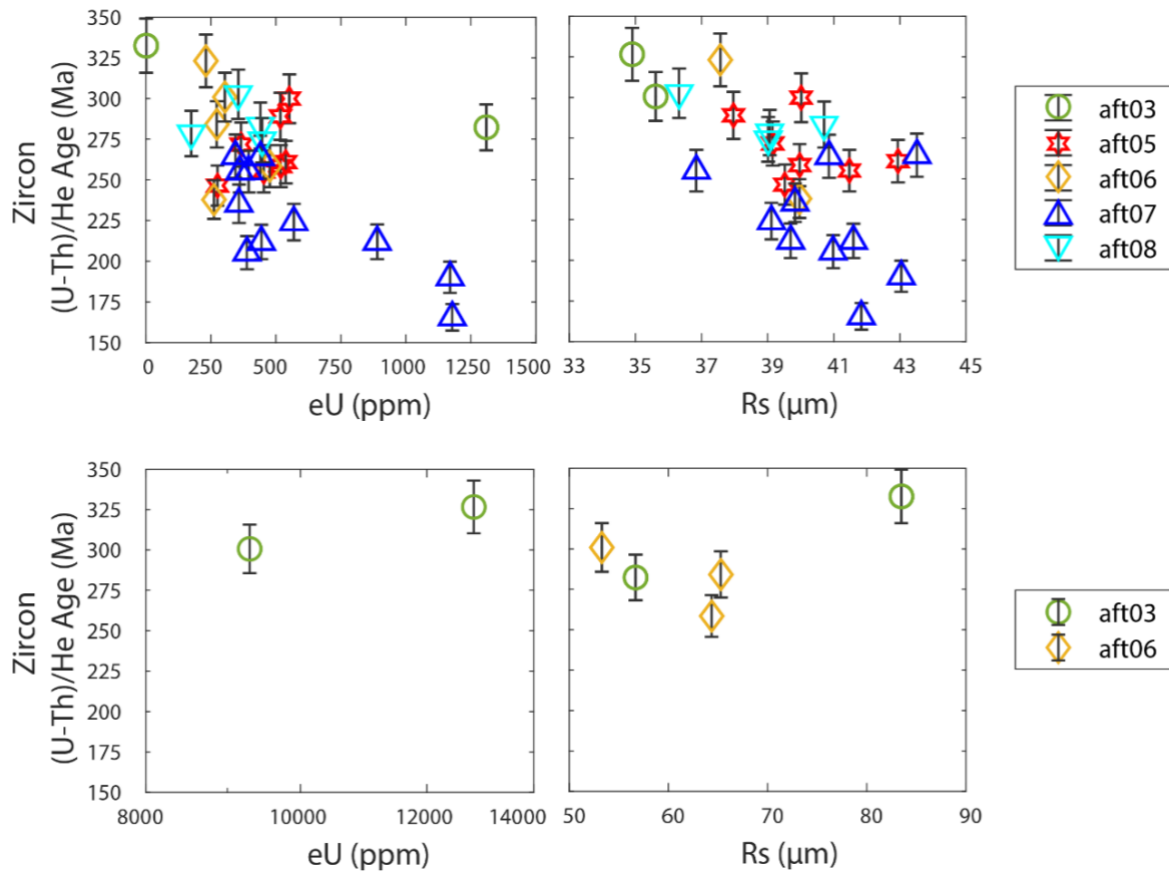
345 Figure 8: Diagram showing all zircons (U-Th)/He data plotted against effective uranium (Ue) concentrations and equivalent spherical radius (Rs). Uncertainties are one standard deviations.
