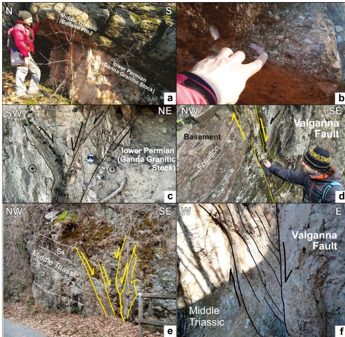
Figure 6: a) middle Permian unconformity highlighted by the contact between the lower Permian Ganna Granitic Stock and the Anisian Bellano Fm.; b) detail of the base of the Bellano Fm.; c, d, e, f, mesoscopic structural features of Valganna Fault (c, d, e, f).
