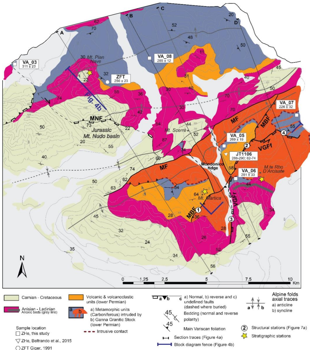
225 Figure 3: Geological map of the Study area (modified after Scaramuzzo et al., 2022). ZHe: zircon (U-Th)/He; ZFT: zircon fission-track. Fault codes: MF, Marzio Fault; MBF, Martica - Boarezzo Fault; VGFr, Valganna Fault ramp segment; VGf, Valganna 230 Fault flat segment. The Mt. Nudo basin is Jurassic in age (Kalin and Trumpy, 1977).
