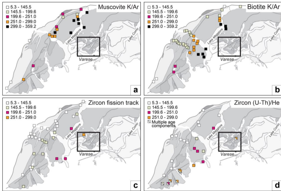
Figure 2: a) Muscovite K/Ar ages compiled from McDowell, 1970; Hunziker, 1974; Zwingmann, 2004; Wolff et al., 2012; b) Biotite K/Ar ages compiled from Jager and Faul, 1960; Carraro and Ferrara, 1968; McDowell, 1968; McDowell, 1970; Hunziker, 1974; Hurford, 1986; Siegesmund et al., 2008; Wolff et al., 2012; c) Zircon fission track ages compiled from Hurford, 1986; Bertotti et al., 1999; Siegesmund et al., 2008; Wolf et al., 2012; d) Zircon (U-Th)/He ages compiled from Wolff et al., 2012; Beltrando et al., 2015. Sample with multiple age components are from detrital rocks and partially reset basement rocks (Beltrando et al., 2015).
