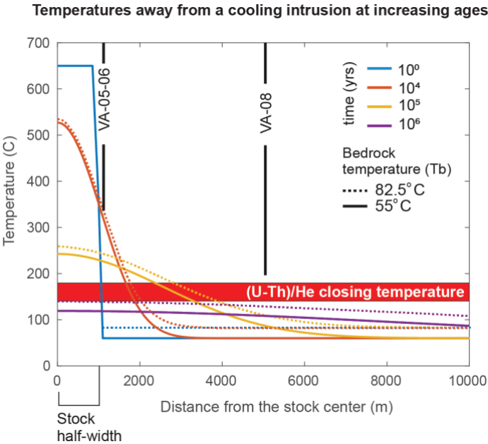
Figure 9: One dimensional transient thermal response to an intrusion (halfwidth = 1000 m). Intrusion depth was assumed to be shallow and into country rock at background temperature ranging between 55°C and 82.5°C.; initial intrusion temperature of 650 °C, and thermal diffusivity of 32 km 2 /Myr.
