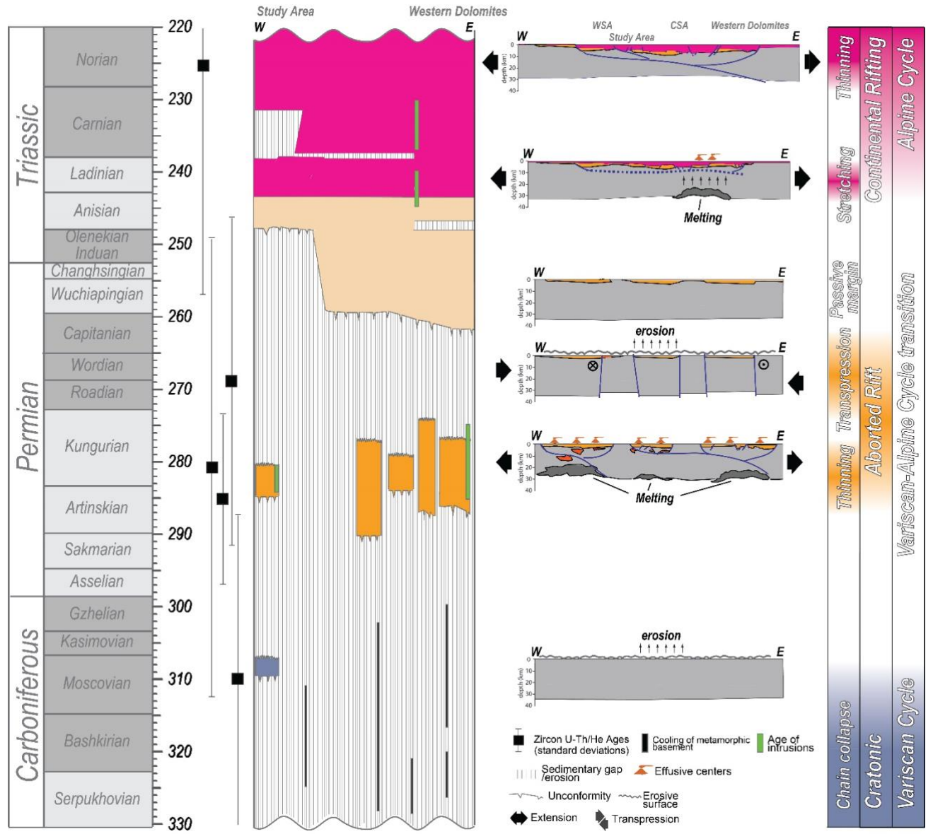
Figure 10. Conceptual and summary scheme of the Variscan-Alpine Cycle transition as constrained in this work and from other works (WSA, Western Southern Alps; CSA, Central Southern Alps): chronostratigraphic scheme redrawn after Schalteger and
