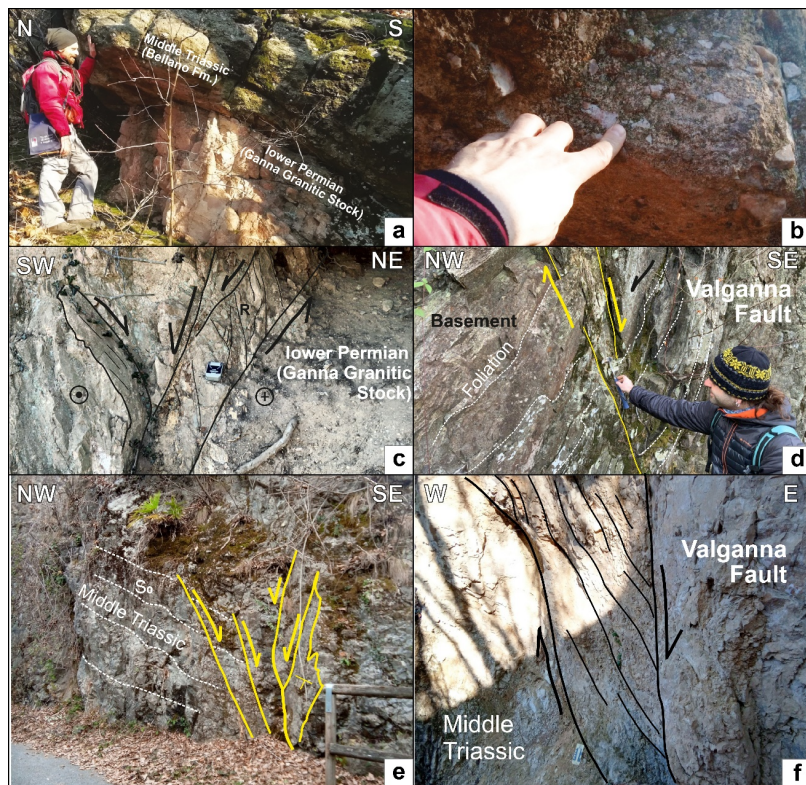
Figure 6: a) middle Permian unconformity highlighted by the contact between the lower Permian Ganna Granitic Stock and the Anisian Bellano Fm.; b) detail of the base of the Bellano Fm.; c, d, e, f, mesoscopic structural features of Valganna Fault (c, d, e, f).
