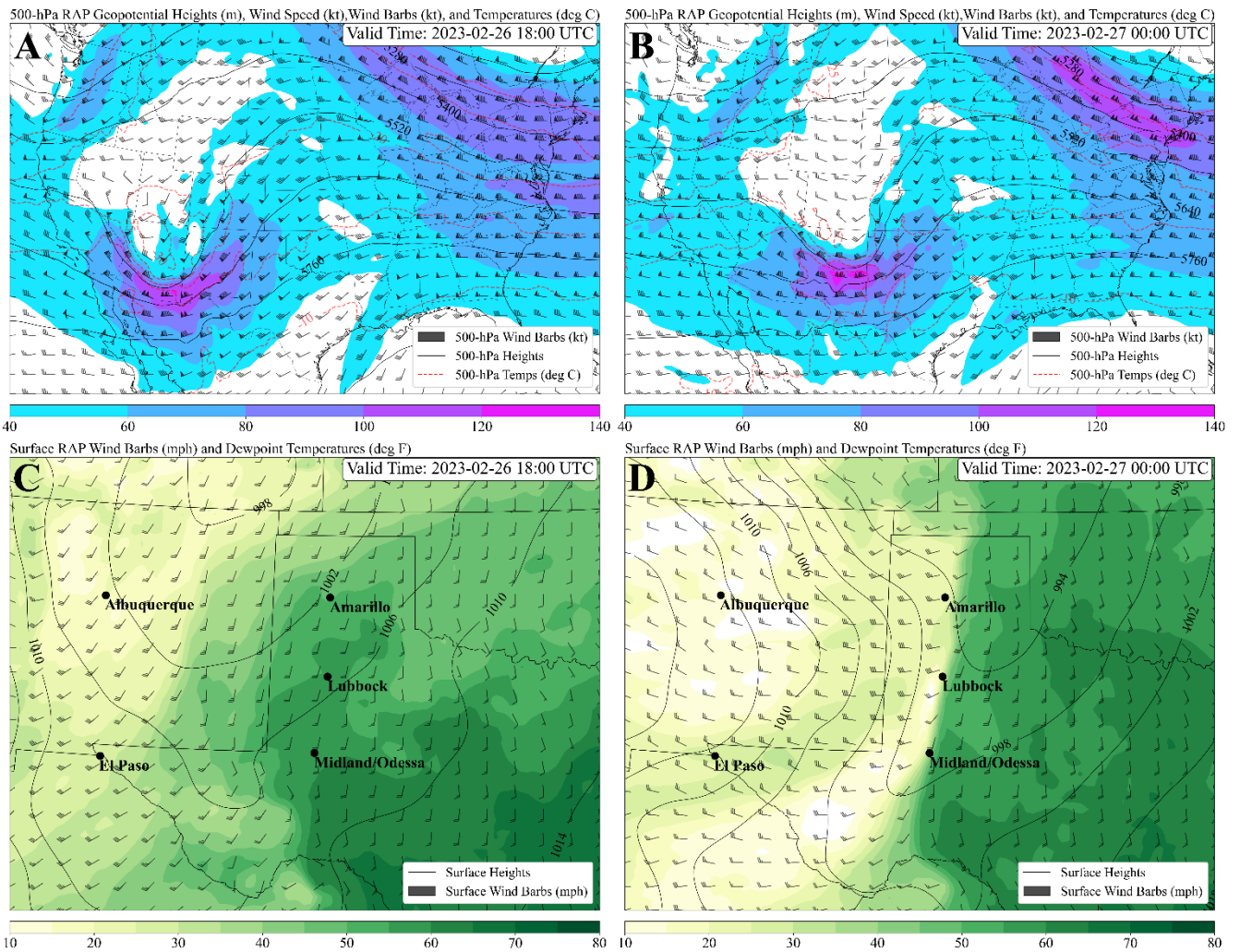
205 Figure 2. 500 mb geopotential heights (m), wind speed (kt, shaded), wind barbs (kt), and temperature ( ^{\circ}\text{C} ) for 26 February 2023 at 18:00 UTC, 12:00 central time, when the dust event started (A) and 27 at 00:00 UTC, 18:00 central time, when the dust event intensified and turned into a dust storm across west Texas (B) and surface wind barbs (mph) and dewpoint temperature ( ^{\circ}\text{C} , shaded) for February 26 at 18:00 UTC, 12:00 central time (C) and 27 at 00:00 UTC, 18:00 central time (D).
