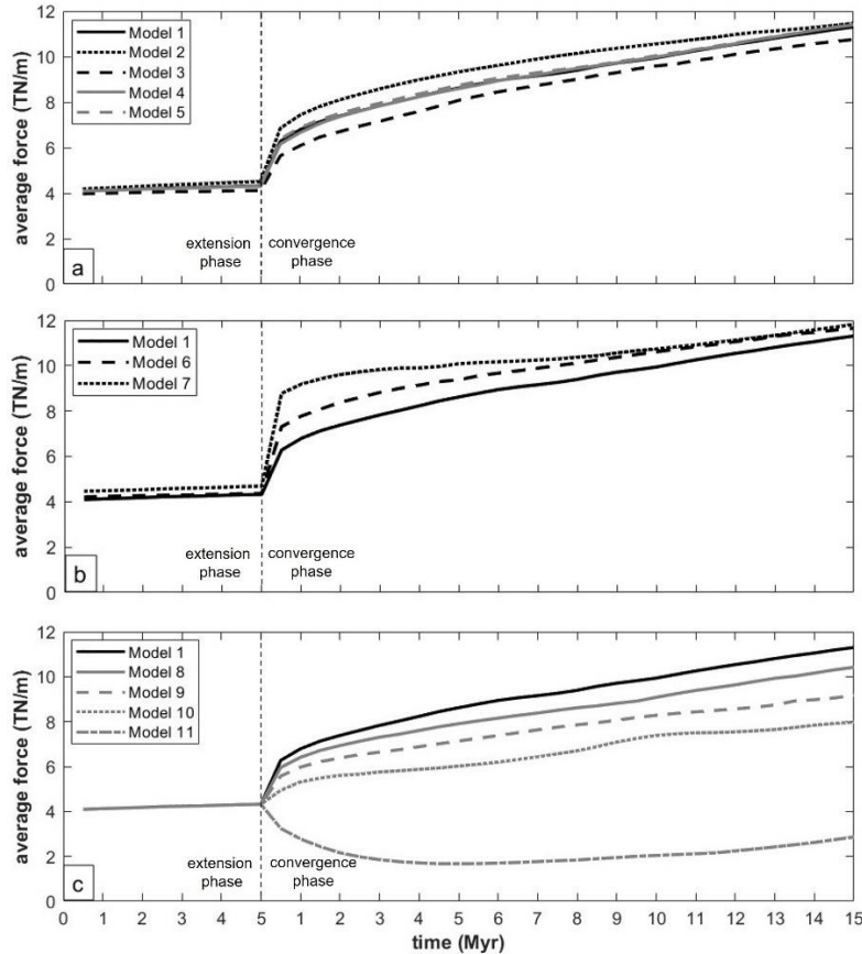
550 Figure 12: Horizontally-averaged boundary force over time. (a) Models with variable salt thickness and salt rheology. (b) Models with variable fault geometry. (c) Models with variable basement shortening rate. Model characteristics are listed in Table 2.
