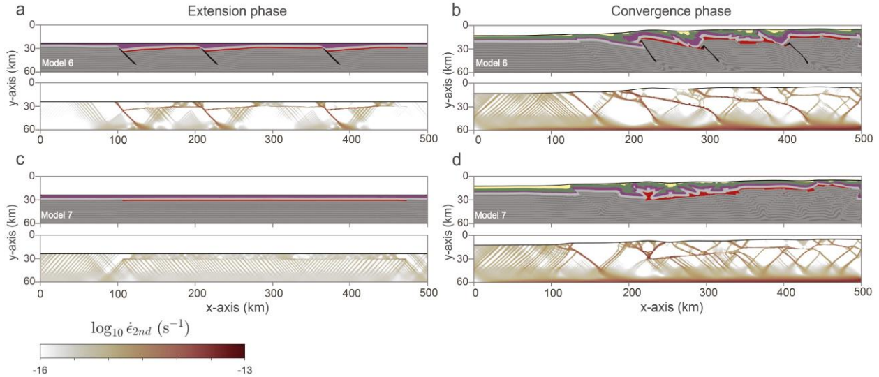
Figure 9: Composition inferred from Lagrangian markers and the second invariant of the strain-rate tensor, affected by different type of inherited faults after 5 Myr of extension and 15 Myr of convergence. (a-b) In the presence of planar inherited faults. (c-d) in the absence of any inherited faults.
