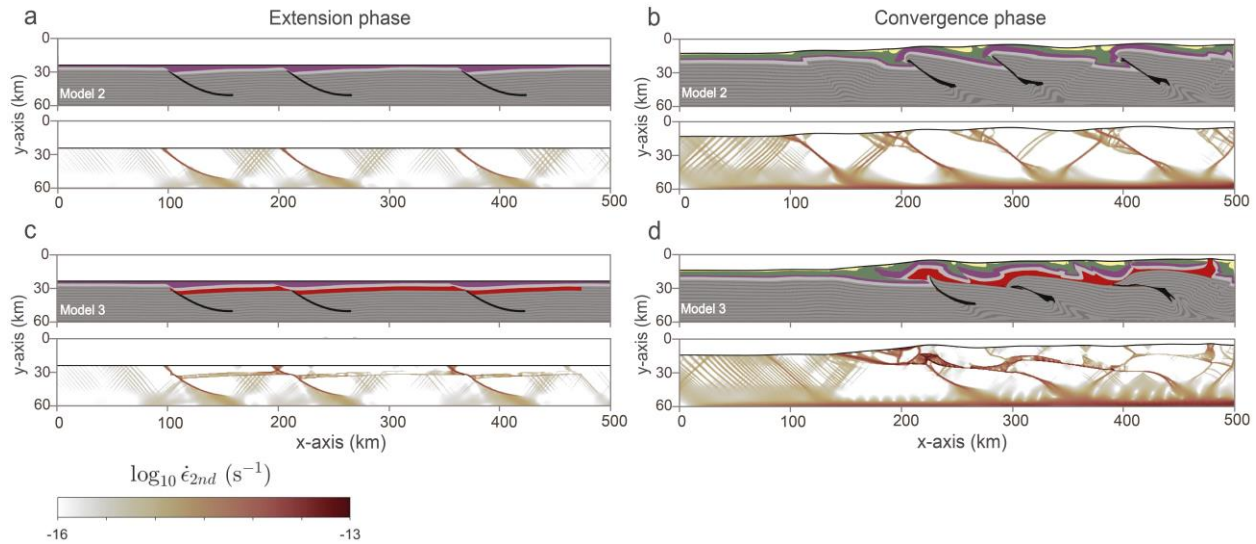
410 Figure 6: Composition inferred from Lagrangian markers and the second invariant of the strain-rate tensor, affected by salt thickness after 5 Myr of extension and 15 Myr of convergence. (a-b) In the absence of salt layer. (c-d) In the presence of a salt layer with 4 km thickness.
