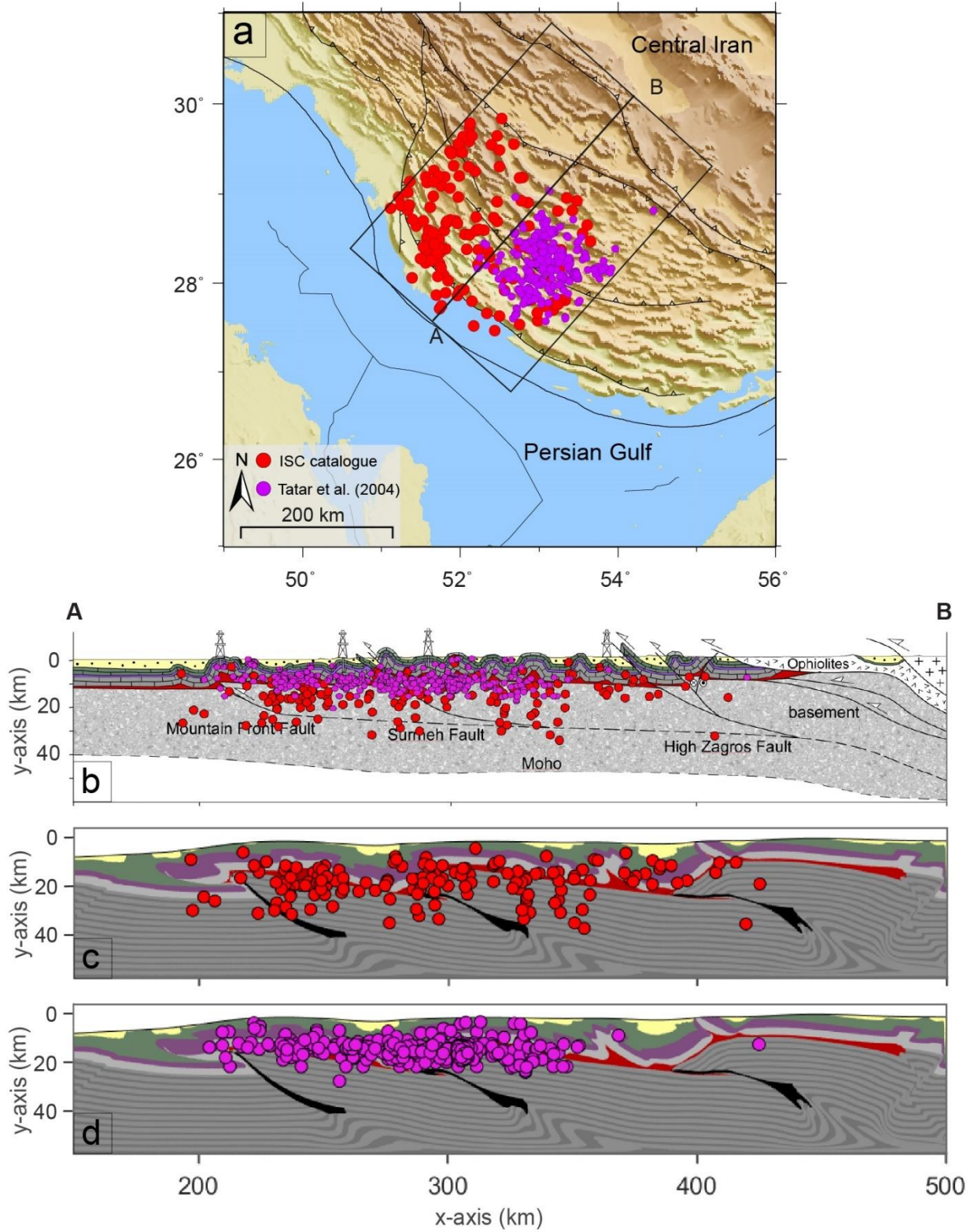
Figure 14: (a) Seismicity of Zagros fold-and-thrust belt reported by ISC during the years 2000 to 2023 with magnitudes M_L > 4 and local temporary network data by Tatar et al (2004) with magnitudes M_L < 4 , superimposed on a shaded relief map derived from Global Topography. (b, c, d) Projection of earthquakes along profile A–B after removing fixed depths on geological cross section and the reference model (Model 1) after 15 Myr of convergence.
