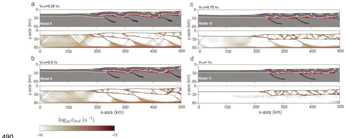
Figure 10: Composition inferred from Lagrangian markers and the second invariant of the strain-rate tensor, affected by different values of basement velocity after 15 Myr of convergence. (a) v_{x,b} = 0.25 , (b) v_{x,b} = 0.5 , (c) v_{x,b} = 0.75 and (d) v_{x,b} = 1 .
