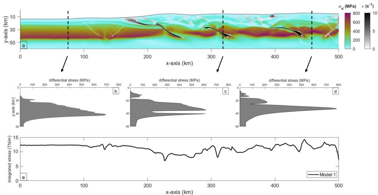
545 Figure 11: (a) strain tensor superimposed on differential stress tensor. (b-d) Differential stress profiles of front of the deformation front, with décollement and basement fault, and without basement fault involved respectively. (e) The integrated stress profile for reference model.
