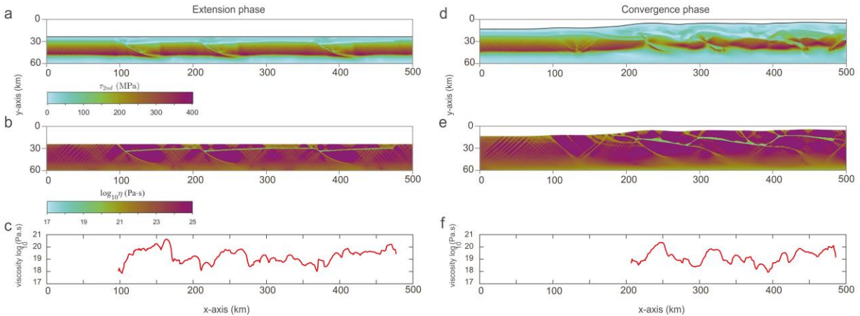
Figure 5: Second invariant of the stress tensor and viscosity after full extension (a, b) and full convergence (d, e). c, f Vertically-averaged viscosity of the nonlinear salt horizon after 5 Myr of extension (c) and 15 Myr of convergence (f), respectively.
