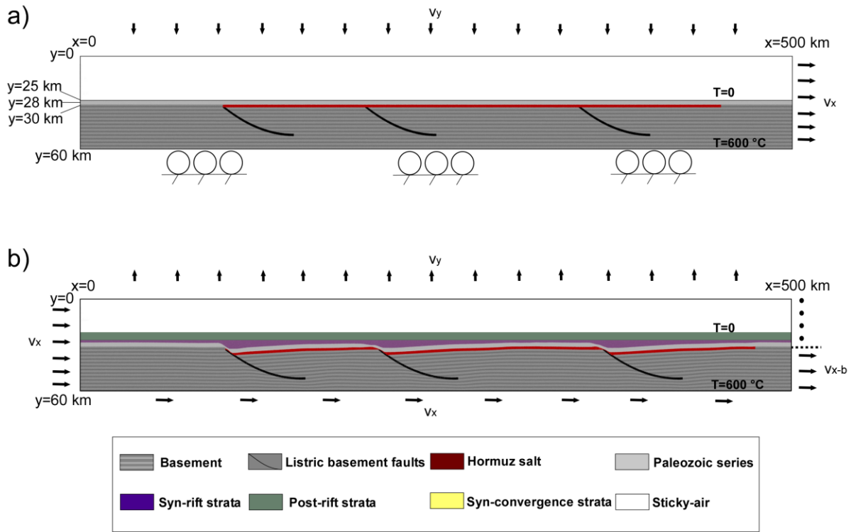
Figure 3: Setup and boundary conditions of numerical modeling. (a) Initial compositional setup for extension phase with listric faults. (b) Fully extended model (5 Myr) with listric faults before convergence. v_x , v_y and v_{x-b} is horizontal velocity, vertical velocity, and basement horizontal velocity, respectively.
