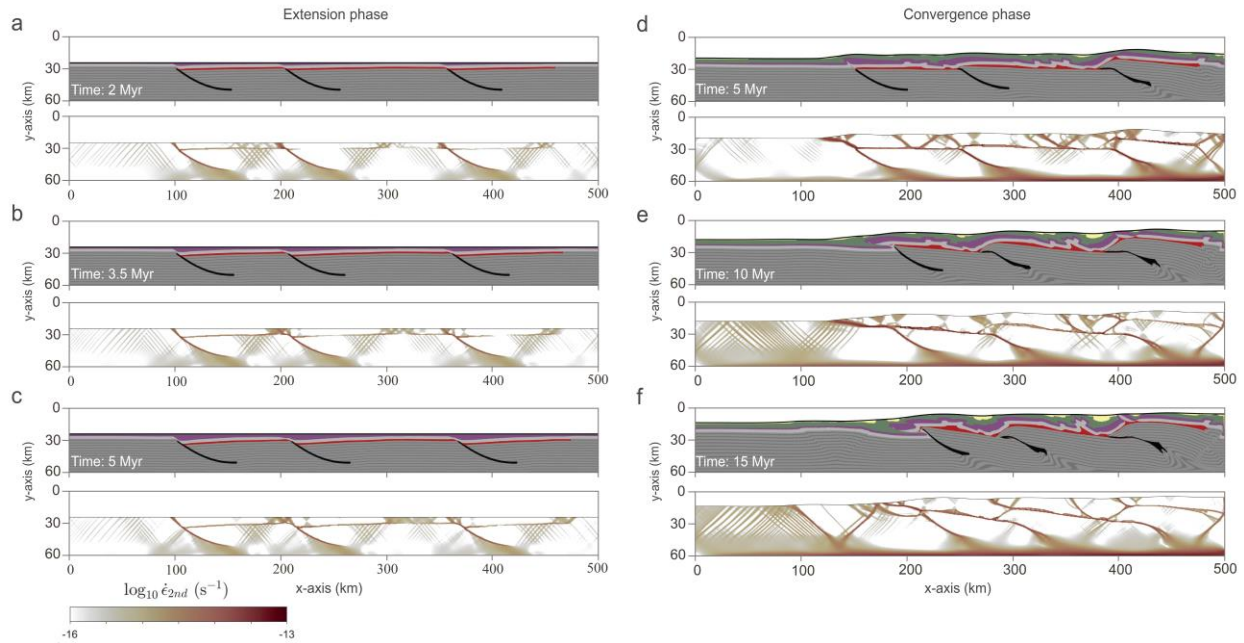
360 Figure 4: Temporal evolution of the reference model during extensional (a-c) and compressional (d-f) phases. For each time panel, the compositional layers (top) derived from the Lagrangian markers, and the second invariant of the strain-rate tensor (bottom) are shown.
