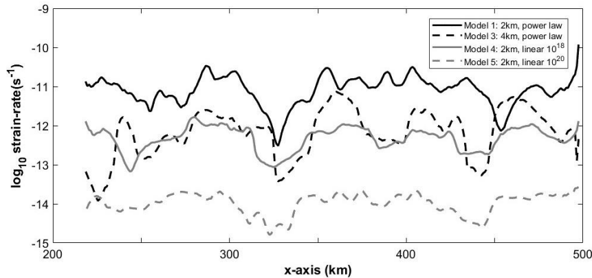
440 Figure 8: Vertically-averaged strain-rate over model width for models with variable salt rheology after 15 Myr of shortening.
