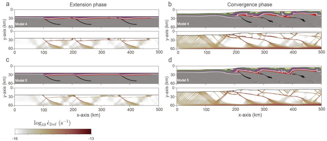
435 Figure 7: Composition inferred from Lagrangian markers and the second invariant of the strain-rate tensor, affected by different viscosity for linear salt layer after 5 Myr of extension and 15 Myr of convergence. (a-b) linear salt horizon with 10^{18} Pa·s viscosity. (c-d) linear salt horizon with 10^{20} Pa·s viscosity.
