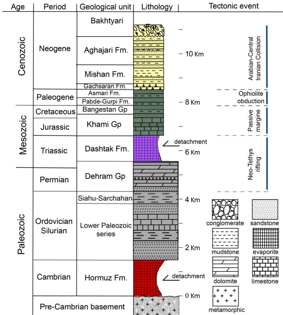
195 Figure 2: Stratigraphic column of the sedimentary cover in the Fars Arc (modified from Callot et al., 2007; Jahani et al. 2009; Motamedi et al., 2012; Mouthereau et al. 2007; Najafi et al. 2014; Sepehr and Cosgrove 2004; Sherkati et al. 2006). Violet and red lithologies represent regional décollement horizons.
