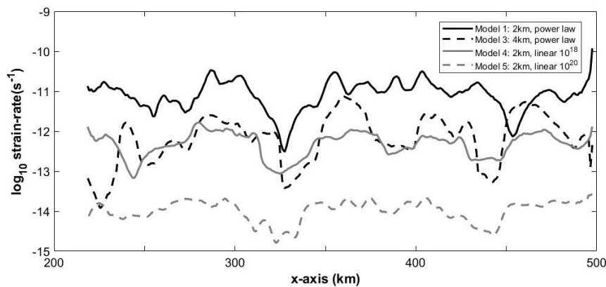
435 Figure 8: Vertically-averaged strain-rate over model width for models with variable salt rheology after 15 Myr of shortening.
