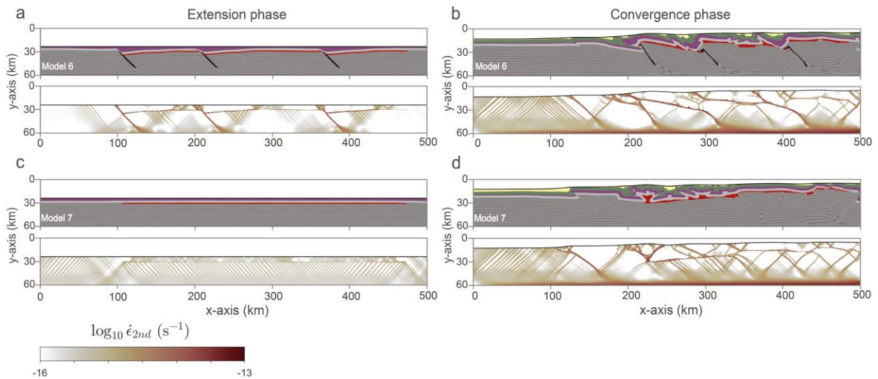
460 Figure 9: Composition inferred from Lagrangian markers and the second invariant of the strain-rate tensor, affected by different type of inherited faults after 5 Myr of extension and 15 Myr of convergence. (a-b) In the presence of planar inherited faults. (c-d) in the absence of any inherited faults.
