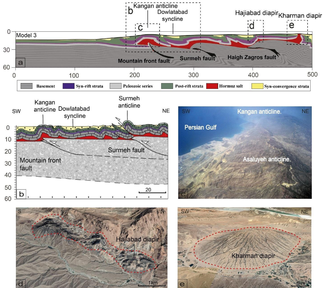
690 Figure 13: (a) The result of numerical modeling with thick salt and basement involved (Model 3). (b) Geological cross section of the Dowlatabad syncline and Kangan anticline (modified from Najafi et al. 2021). (c) Aerial image of Asalouyeh and Kangan anticlines. (d) Satellite image of the Hajiabad Diapir (© Google Earth). (e) Satellite image of the Kharman Diapir (© Google Earth).
