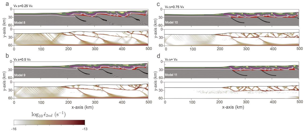
490 Figure 10: Composition inferred from Lagrangian markers and the second invariant of the strain-rate tensor, affected by different values of basement velocity after 15 Myr of convergence. (a) v_{x-b} = 0.25 , (b) v_{x-b} = 0.5 , (c) v_{x-b} = 0.75 and (d) v_{x-b} = 1 .
