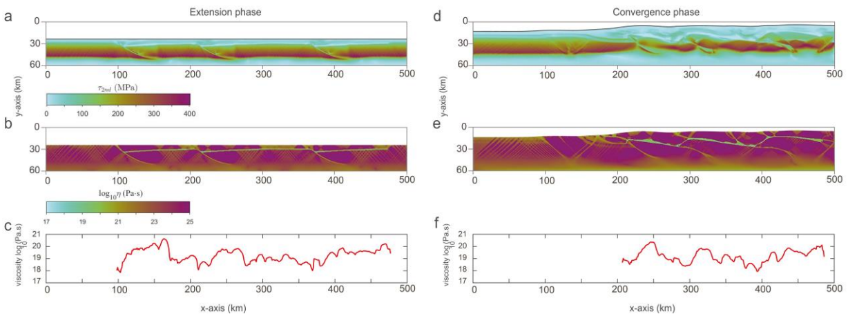
Figure 5: Second invariant of the stress tensor and viscosity after full extension (a,b) and full convergence (d,e). c, f Vertically-averaged viscosity of the nonlinear salt horizon after 5 Myr of extension (c) and 15 Myr of convergence (f), respectively.
