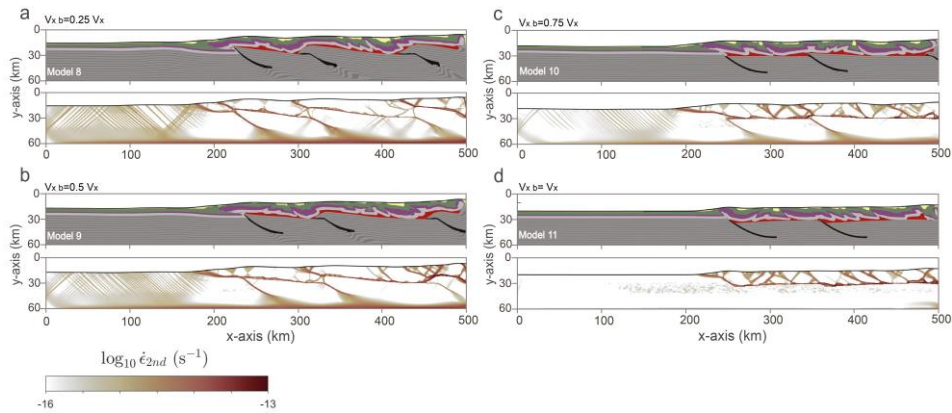
525 Figure 10: Composition inferred from Lagrangian markers and the second invariant of the strain-rate tensor, affected by different values of basement velocity after 15 Myr of convergence. (a) v_{x,b} = 0.25 v_x , (b) v_{x,b} = 0.5 , (c) v_{x,b} = 0.75 and (d) v_{x,b} = 1 .
