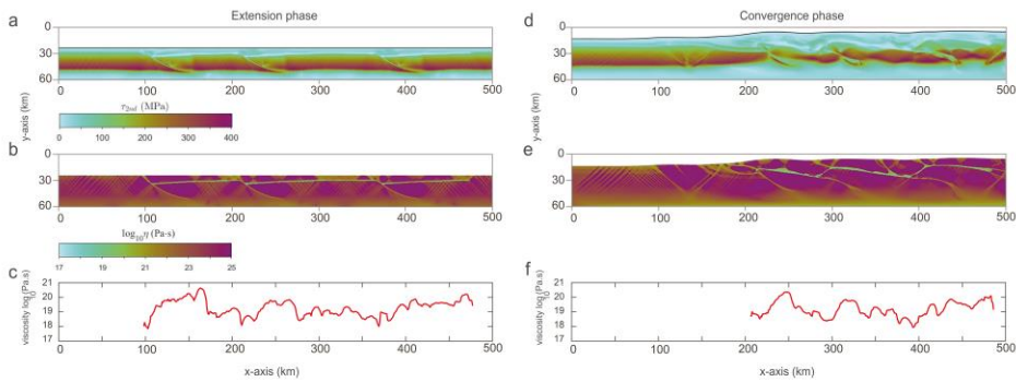
415 Figure 5: Second invariant of the stress tensor and viscosity after full extension (a, b) and full convergence (d, e). c, f Vertically-averaged viscosity of the nonlinear salt horizon after 5 Myr of extension (c) and 15 Myr of convergence (f), respectively.
