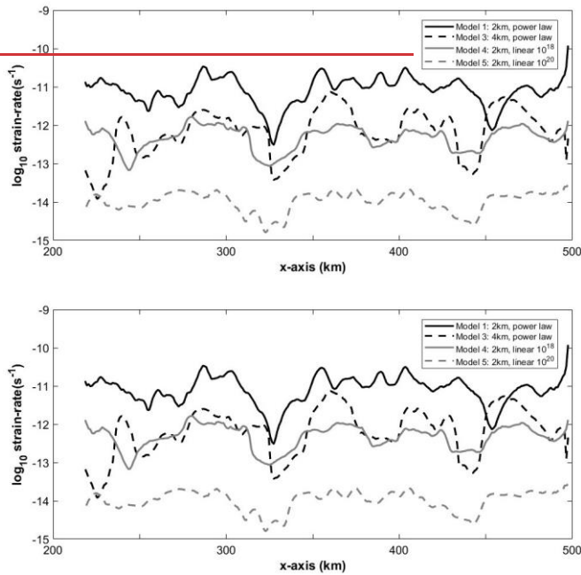
Figure 8: Vertically-averaged strain-rate over model width for models with variable salt rheology after 15 Myr of shortening.
