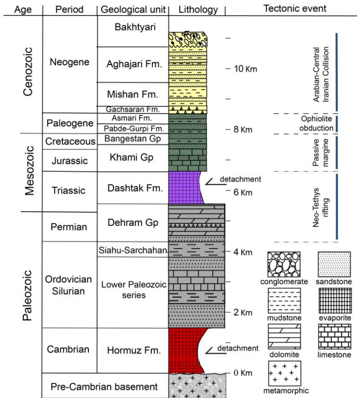
215 Figure 2: Stratigraphic column of the sedimentary cover in the Fars Arc (modified from Callot et al., 2007; Jahani et al. 2009; Motamedi et al., 2012; Mouthereau et al. 2007; Najafi et al. 2014; Sepehr and Cosgrove 2004; Sherkati et al. 2006). Violet and red lithologies represent regional décollement horizons.
