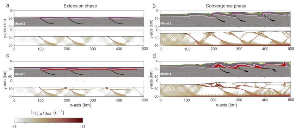
Figure 6: Composition inferred from Lagrangian markers and the second invariant of the strain-rate tensor, affected by salt thickness after 5 Myr of extension and 15 Myr of convergence. (a-b) In the absence of salt layer. (c-d) In the presence of a salt layer with 4 km thickness.
