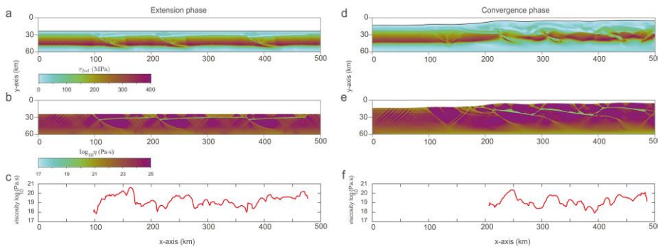
Figure 5: Second invariant of the stress tensor and viscosity after full extension (a, b) and full convergence (d, e). c, f) Vertically-averaged viscosity of the nonlinear salt horizon after 5 Myr of extension (c) and 15 Myr of convergence (f), respectively.
