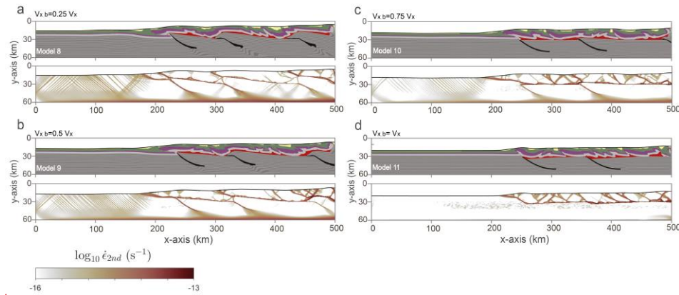
Figure 910: Composition inferred from Lagrangian markers and the second invariant of the strain-rate tensor, affected by different values of basement velocity after 15 Myr of convergence. (a) v_{x,b} = 0.25 , (b) v_{x,b} = 0.5 , (c) v_{x,b} = 0.75 and (d) v_{x,b} = 1 .
