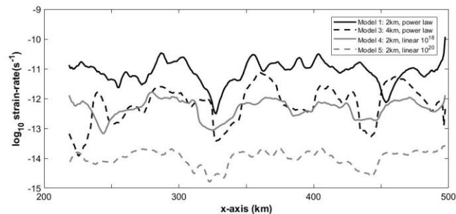
Figure 78: Vertically-averaged strain-rate over model width for models with variable salt rheology after 15 Myr of shortening.
