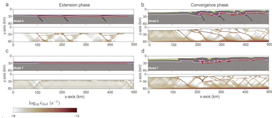
Figure 89: Composition inferred from Lagrangian markers and the second invariant of the strain-rate tensor, affected by different type of inherited faults after 5 Myr of extension and 15 Myr of convergence. (a-b) In the presence of planar inherited faults. (c-d) In the absence of any inherited faults.
