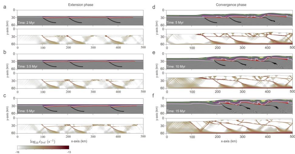
Figure 4: Temporal evolution of the reference model during extensional (a-c) and compressional (d-f) phases. After 15 Myr, the intensity of thin skinned folding within the sedimentary cover increases (Fig. 4g). For each time panel, the compositional layers (top) derived from the Lagrangian markers, and the second invariant of the strain-rate tensor (bottom) are shown.
