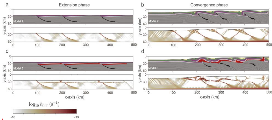
Figure 56: Composition inferred from Lagrangian markers and the second invariant of the strain-rate tensor, affected by salt thickness after 5 Myr of extension and 15 Myr of convergence. (a-b) In the absence of salt layer. (c-d) In the presence of a salt layer with 4 km thickness.
