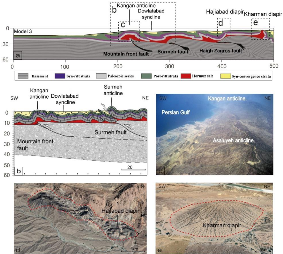
Figure 1213: (a) The result of numerical modeling with thick salt and basement involved (Model 3). (b) Geological cross section of the Dowlatabad syncline and Kangan anticline (modified from Najafi et al. 2021). (c) Aerial image of Asalouyeh and Kangan anticlines. (d) Satellite image of the Hajlabad Diapir (© Google Earth). (e) Satellite image of the Kharman Diapir (© Google Earth).
