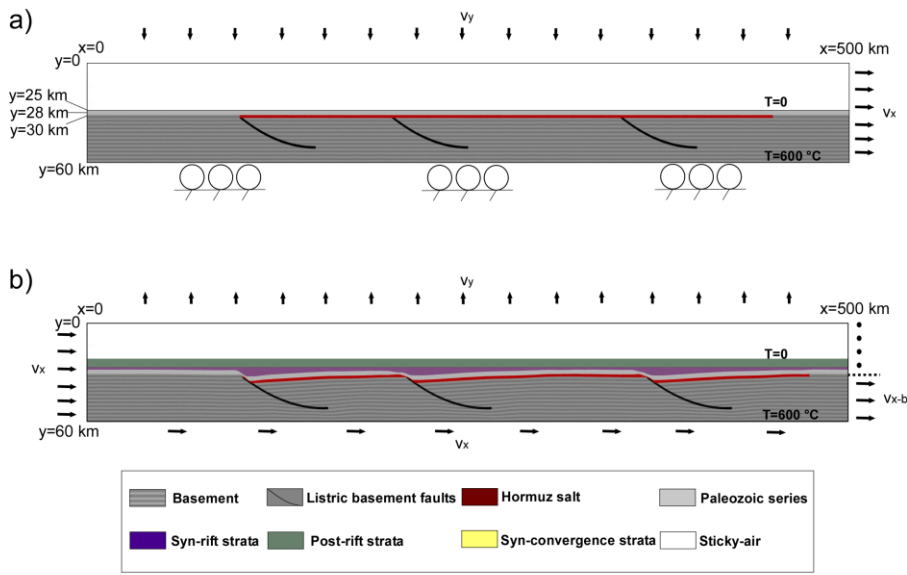
325 Figure 3: Setup and boundary conditions of numerical modeling. (a) Initial compositional setup for extension phase with listric faults. (b) Fully extended model (5 Myr) with listric faults before convergence. v_x , v_y and v_{x-b} is horizontal velocity, vertical velocity, and basement horizontal velocity, respectively.
