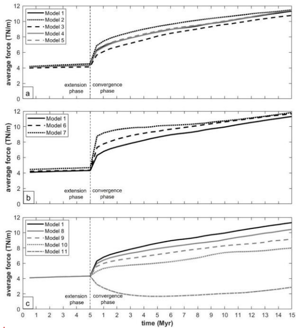
Figure 14.12: Horizontally-averaged boundary force over time. (a) Models with variable salt thickness and salt rheology. (b) Models with variable fault geometry. (c) Models with variable basement shortening rate. Model characteristics are listed in Table 2.
