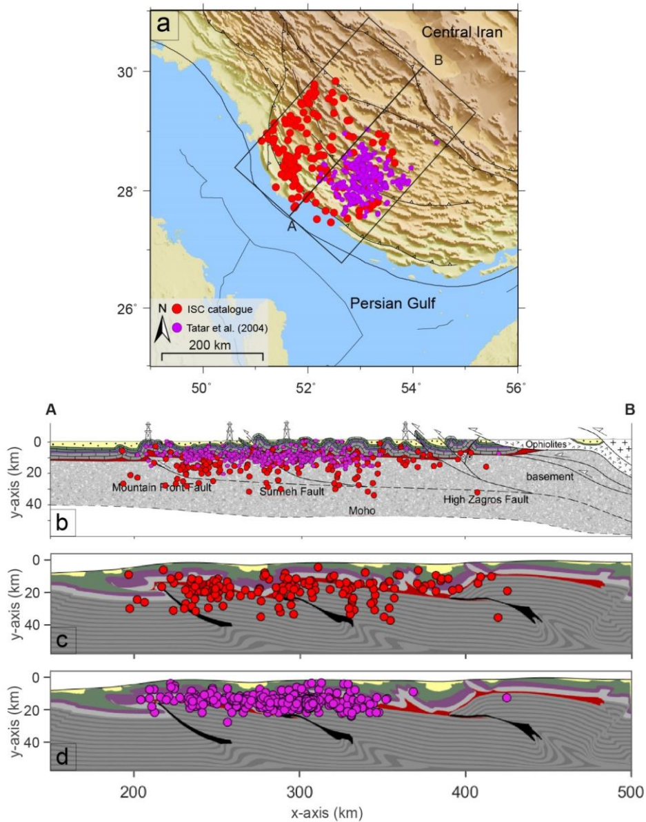
Figure 1314: (a) Seismicity of Zagros fold-and-thrust belt reported by ISC during the years 2000 to 2023 with magnitudes M_L \gg 4 and local temporary network data by Tatar et al (2004) with magnitudes M_L < 4 , superimposed on a shaded relief map derived from Global Topography. (b, c, d) Projection of earthquakes along profile A–B after removing fixed depths on geological cross section and the reference model (Model 1) after 15 Myr of convergence.
