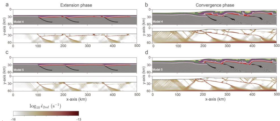
Figure 67: Composition inferred from Lagrangian markers and the second invariant of the strain-rate tensor, affected by different viscosity for linear salt layer after 5 Myr of extension and 15 Myr of convergence. (a-b) linear salt horizon with 10^{18} Pa-s viscosity. (c-d) linear salt horizon with 10^{20} Pa-s viscosity.
