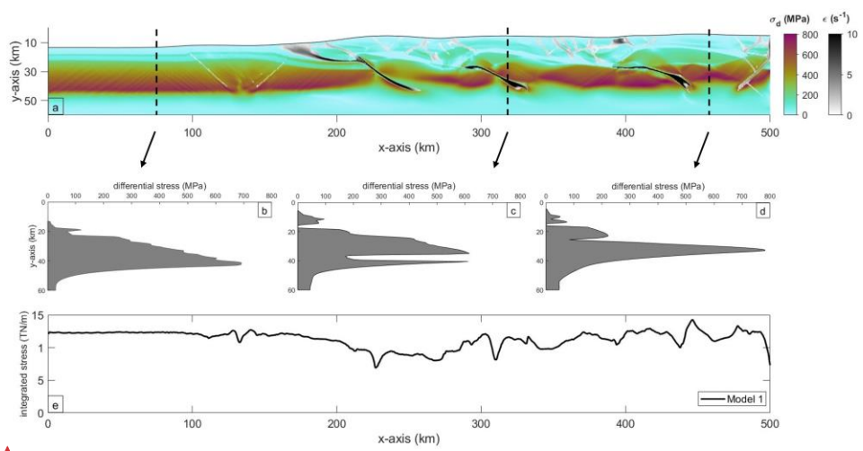
570 Figure 10: (a) strain tensor superimposed on differential stress tensor. (b-d) Differential stress profiles of front of the deformation front, with décollement and basement fault, and without basement fault involved respectively. (e) The integrated stress profile for reference model.
