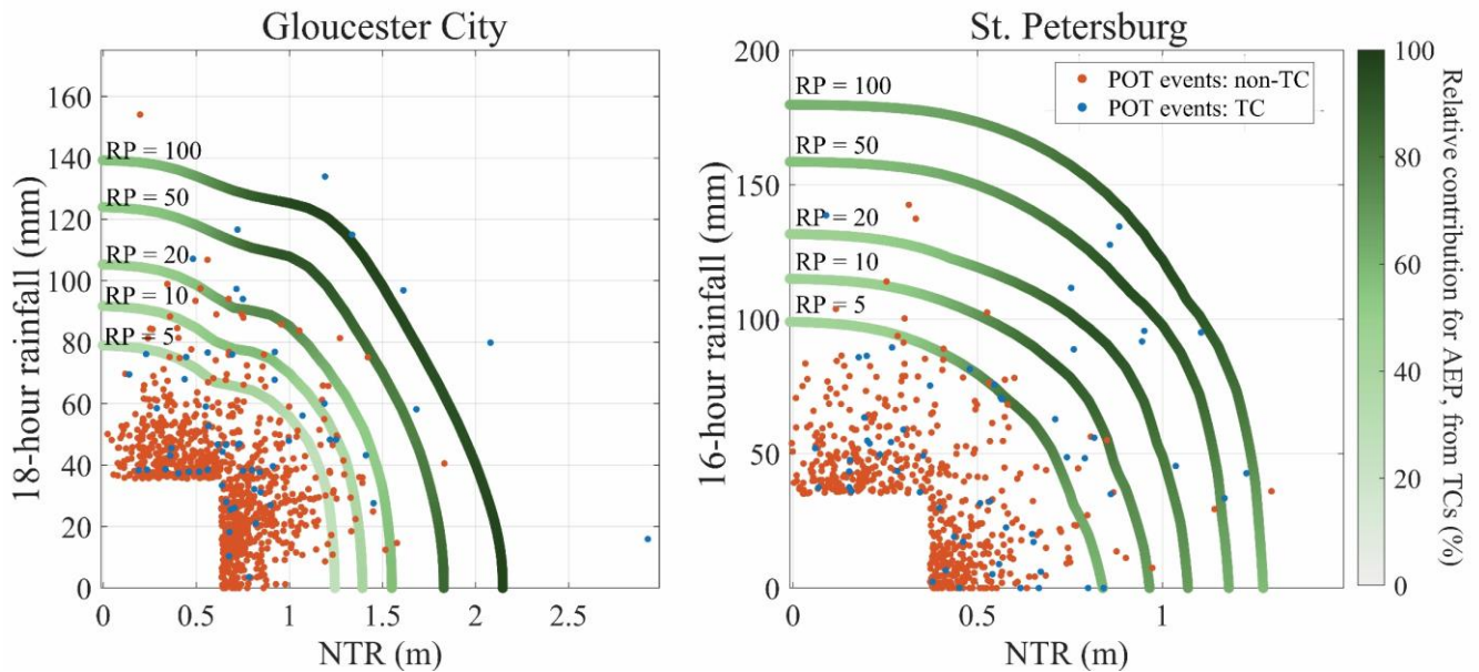
360 Figure 10: Relative contribution of TCs to the AEP along the joint probability isolines for the two study locations. The color scale indicates the ratio of AEP associated with TCs to the combined AEP of both populations.
