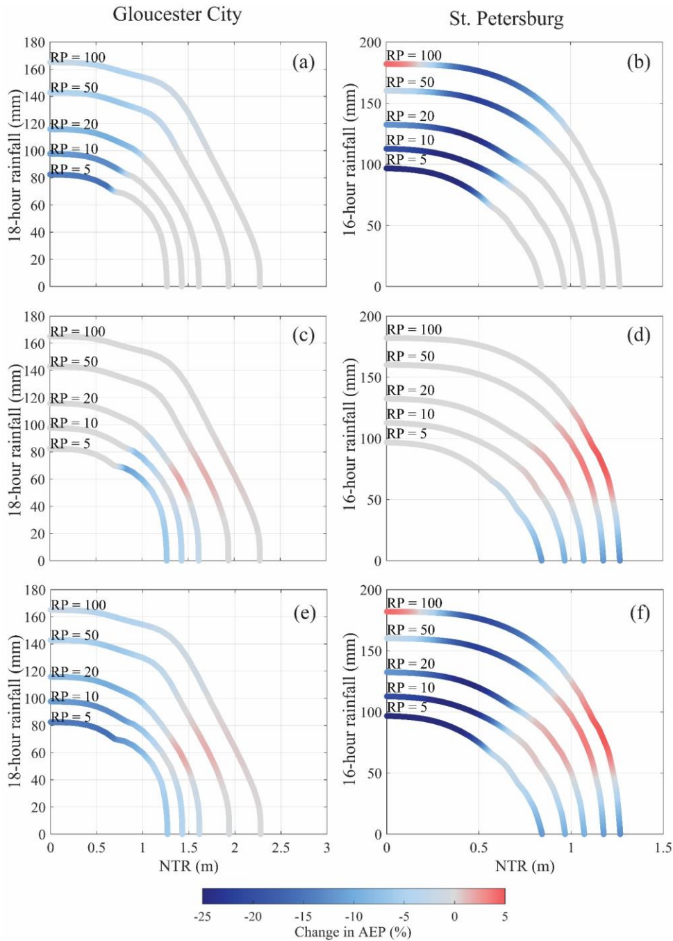
380 Figure 11: Change in AEP of combined populations in Gloucester City (left) and St. Petersburg (right): (a), (b) when omitting the non-classified POT RF events; (c), (d) when omitting the non-classified POT NTR events; and (e), (f) when omitting all non-classified events. The change in AEP was calculated along the joint probability isolines derived for the analysis where events are stratified as TC and non-TC.
