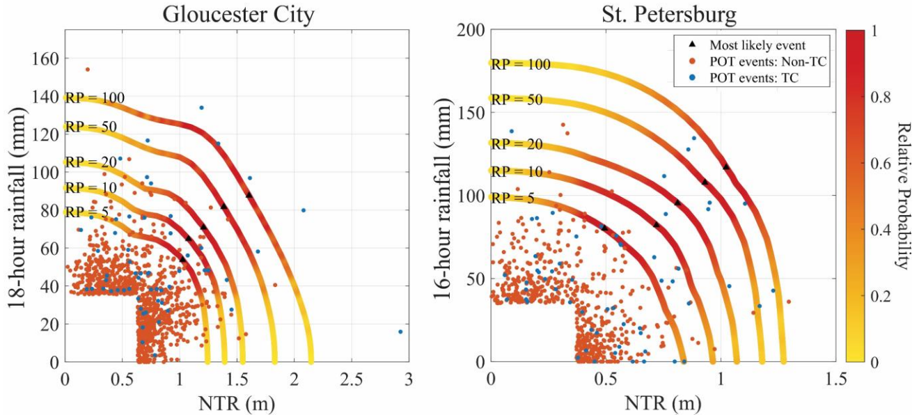
355 Figure 9: Joint probability isolines for the two study sites after combining the AEPs of the two populations (TC and non-TC). The color scale indicates the relative probability of events along the isolines. The location of the “most likely” event is assigned to the point with the highest relative probability density on an isoline.
