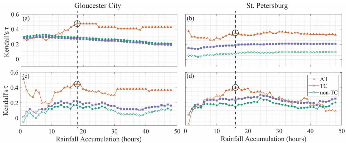
Figure 3: Kendall's \tau between NTR and RF for different RF accumulation times for all events (purple), TCs (orange), and non-TCs (green) for samples conditioned on NTR (a and b) and RF (c and d). Filled markers indicate values that are significant at 5% level. The black circles with vertical dashed line show the selected RF accumulation for each location.
