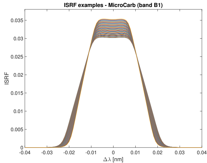
Figure 1. Illustration of a superposition of 1024 ISRFs with centered wavelengths \lambda_l = 758.3, \dots, 768.3\text{nm} around their central wavelengths. The ISRFs have been simulated for the band B1 of the MicroCarb instrument using uniform scenes.
