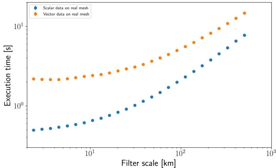
Figure 7. Execution time of implicit filter on FESOM2 output. Results show computation time of both vector and scalar data on 11 M node mesh (see Sec. 3).
