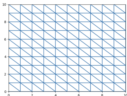
Figure 2. A regular rectangular mesh is converted into a triangular mesh by bisecting each rectangle into two triangles.
