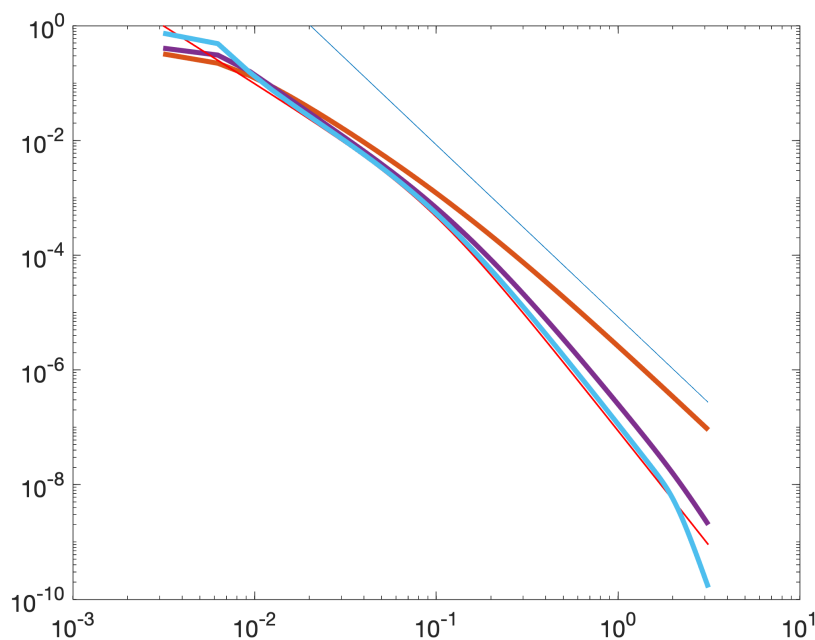
Figure 8. Theoretical energy spectra obtained using Laplacian (thick red), bi-Laplacian (violet) and four-Laplacian implicit filters. The Fourier spectrum is shown by thin red line and the straight line corresponds to a slope of -3 .
