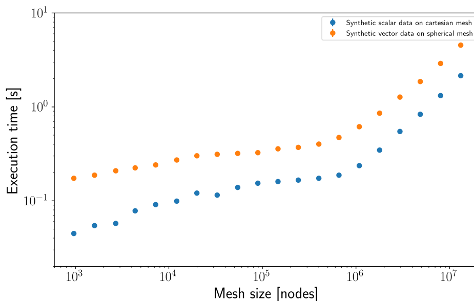
Figure 6. Execution time of implicit filter on synthetic data. Presenting both data on a Cartesian and spherical mesh. Filter size of 100 km was used at all cases.
