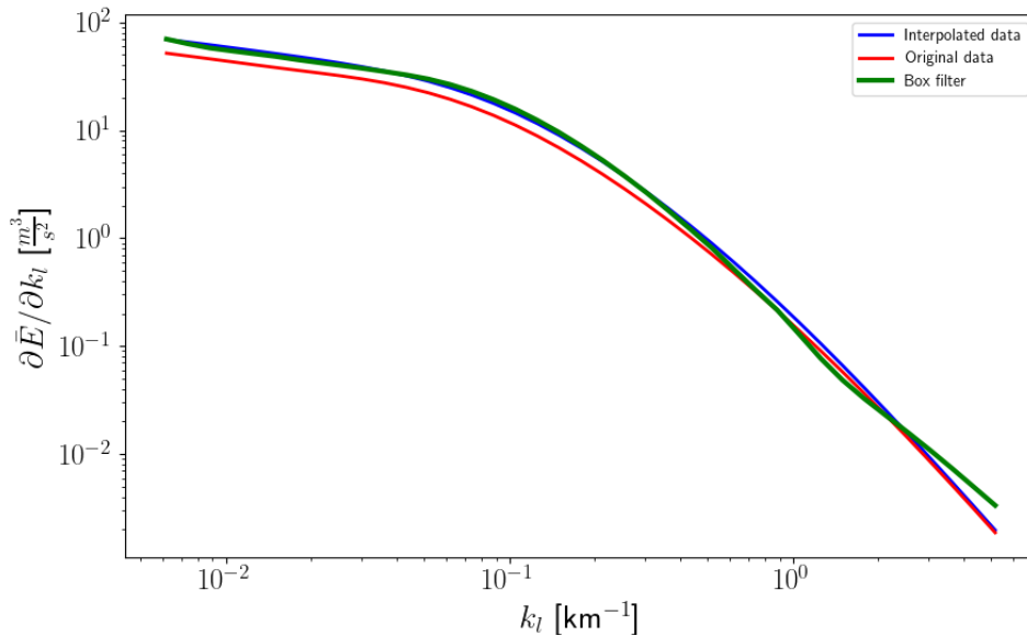
Figure 4. Wavenumber spectra for entire Arctic Ocean. Red line corresponds to the implicit harmonic filter applied to the data on the original grid. The blue and green lines correspond to the implicit harmonic and explicit box filter applied to the interpolated data. The highest wavenumber is \pi/h , where h is the height of triangles of the original grid.
