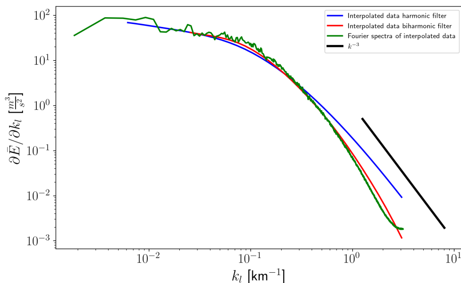
Figure 9. Fourier energy spectrum compared to the spectra obtained with implicit harmonic and biharmonic filters for the data interpolated to a regular grid.
