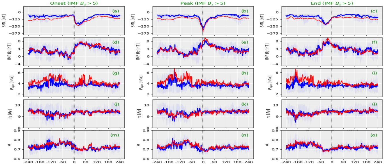
Figure 3. Superposed epoch analysis (median (blue), mean (red), interquartile range (shaded)) of the ( a-c ) SML index, ( d-f ) IMF B_Z , ( g-i ) dynamic pressure P_{dyn} , and magnetopause location parameters ( j-l ) r_0 , ( m-o ) \alpha for strongly northward IMF ( \langle B_Z \rangle > 5 nT). Three zero epoch times are used: (left) substorm onset, (center) substorm peak, and (right) substorm end.
