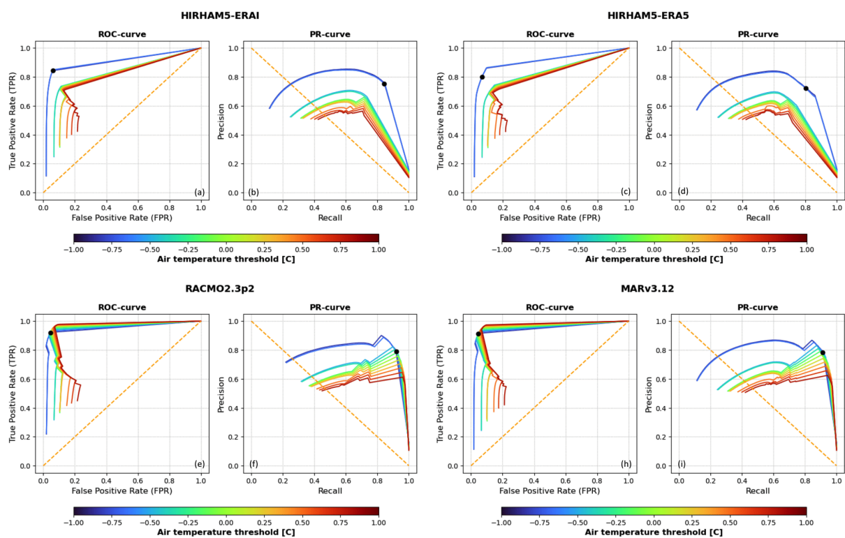
Figure 5. ROC- and PR-curves for possible RCM melting thresholds using varying AWS temperature thresholds. The black dot indicates the optimal melting threshold for each RCM given in Table 1.
