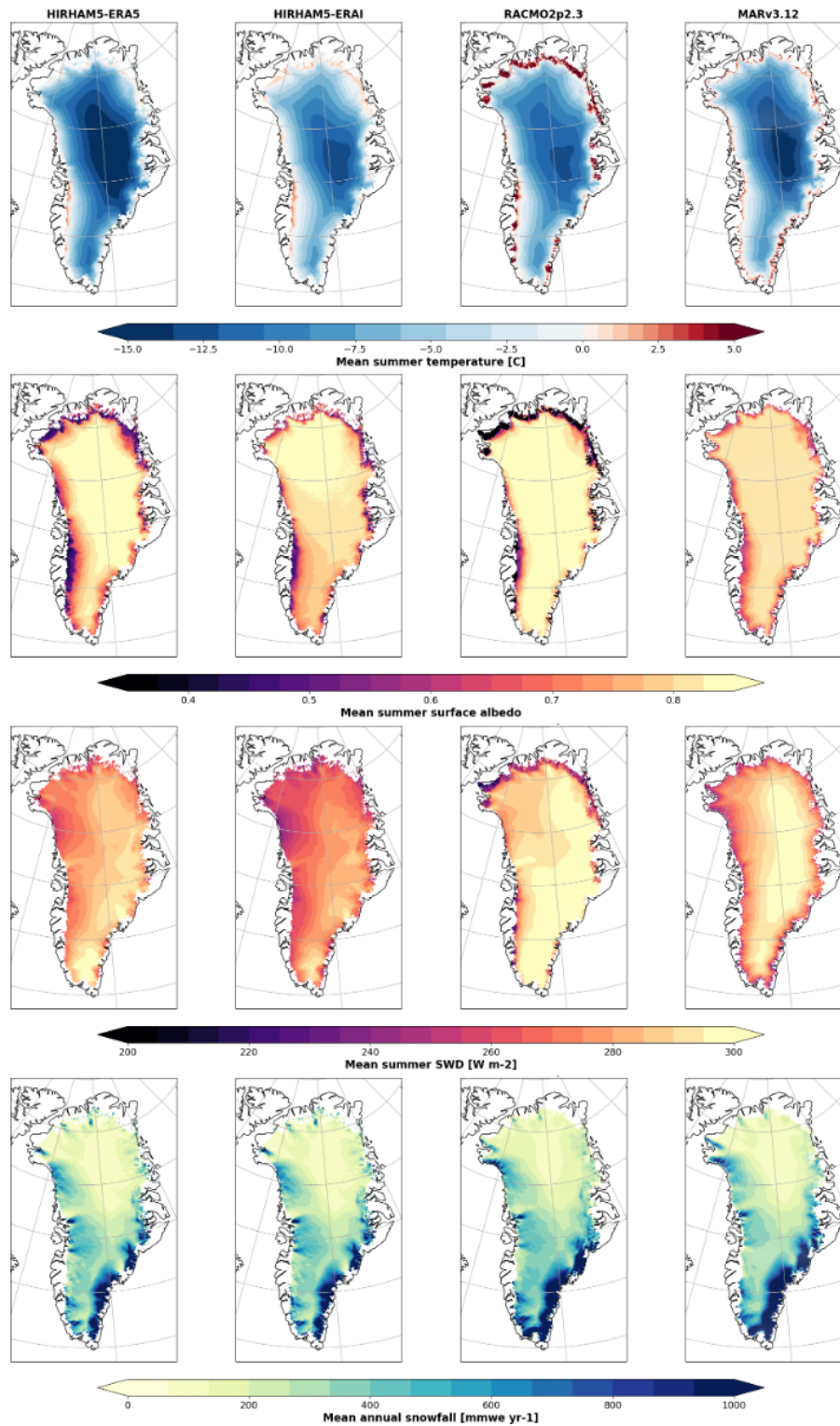
Figure 3. RCM simulated variables from 2007-2020 for HIRHAM-ERA5, HIRHAM-ERA1, MARv3.12 and RACMO2.3p2. (a-d): mean JJA temperatures in °C, (e-f): the JJA surface albedo, (g-h): the JJA SWD in W m -2 , and (i-l): the mean annual snowfall in mm w.e. yr -1 .
