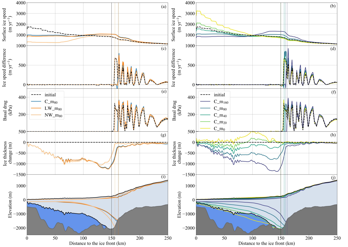
Figure 7. Surface ice speed (a, b), ice speed difference (c, d; surface minus basal), basal drag (e, f) ice thickness change (g, h), and ice-sheet profiles (i, j) along FL1 in the initial year 2015 (black solid line) and the year 2100 (coloured solid line) from experiments (Table 3) in the Sliding parameterization group (left column) and the year 2050 (coloured solid line) in the Melt rate group (right column). grounding line positions are marked with black vertical dashed line for the year 2015 and coloured vertical dashed line for the year 2100 in the Sliding parameterization group (left column) and the year 2050 (coloured solid line) in the Melt rate group (right column). The figure is shaded to show the geometry of the TG along the flow line in 2015, where dark grey is the bedrock, light blue the ice shelf and dark blue seawater. The elevations are exaggerated by a factor of 25.
