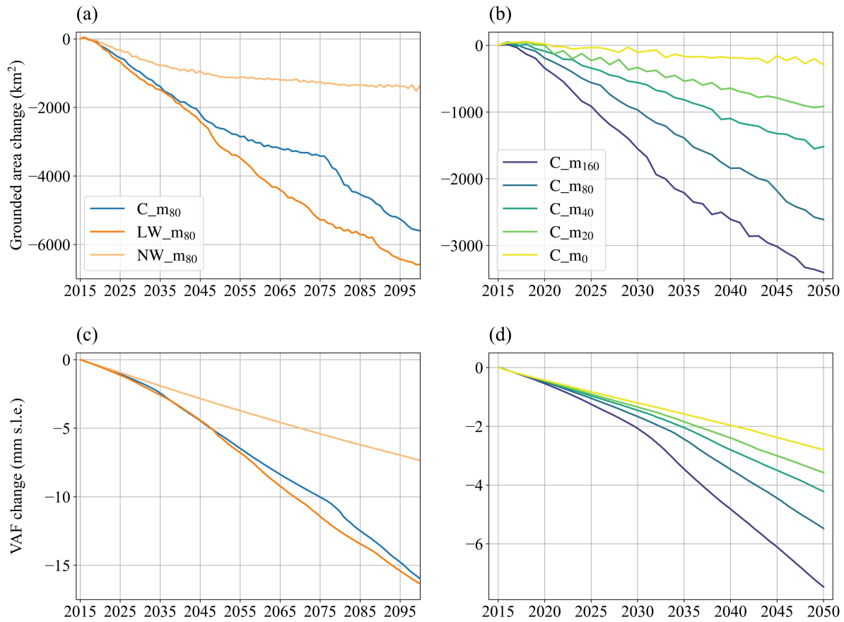
485 Figure 9. Grounded area change (a, b) and VAF change (c, d) of Sliding parameterization group (a, c) over the period 2015-2100 and Melt rate group (b, d) over the period 2015-2050.
