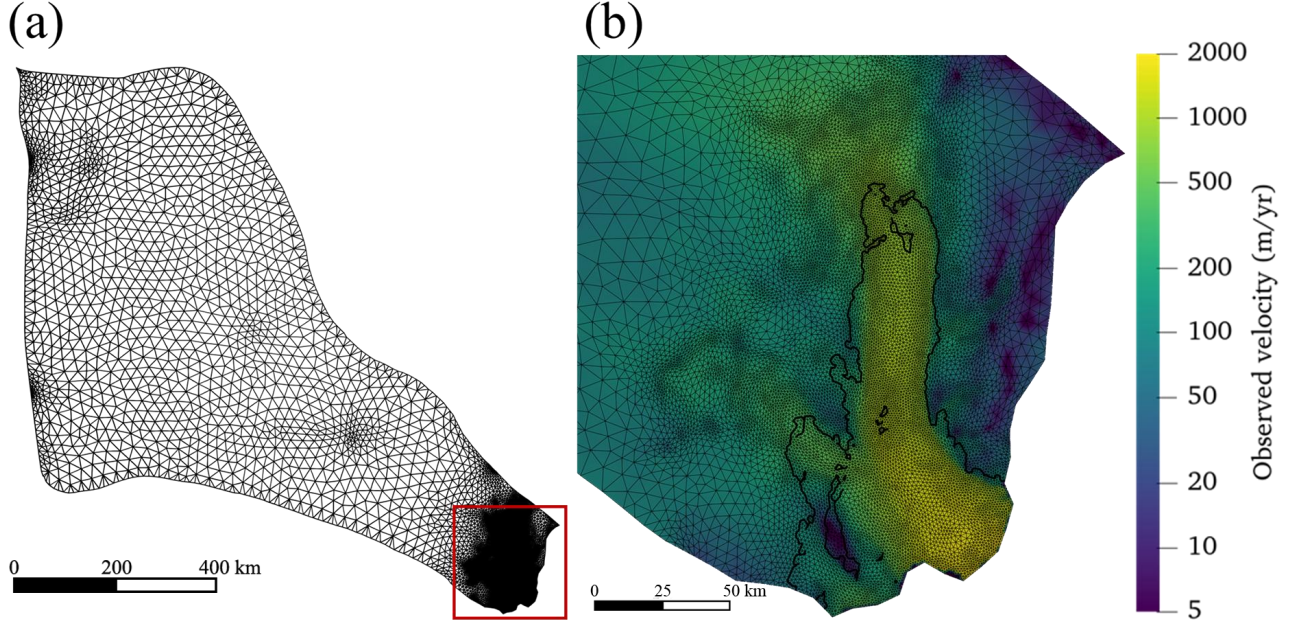
140 Figure 2. The refined 2D horizontal domain footprint mesh (a) . Boxes outlined in panel (a) are shown in detail and overlain with surface ice velocity in panel (b) . The solid black curves in (b) represent the positions of the grounding line.
