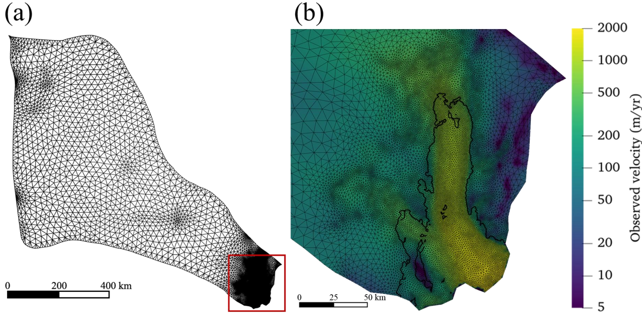
Figure 2. The refined 2D horizontal domain footprint mesh (a). Boxes outlined in panel (a) are shown in detail and overlain with surface ice velocity in panel (b). The solid black curves in (b) represent the positions of the grounding line.
