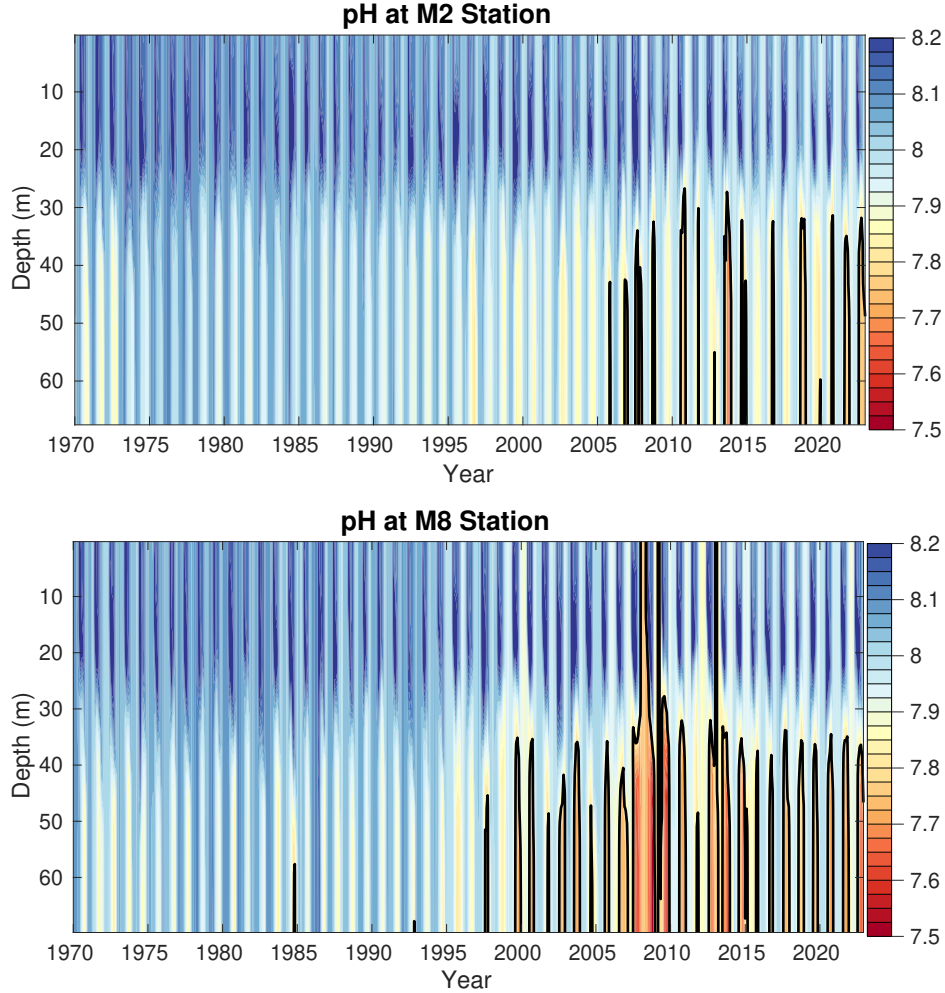
495 Figure 9: Model monthly averaged pH over the entire model timeseries at the M2 (top) and M8 (bottom) approximate model locations. The black contour line denotes the threshold for pH values < 7.8, which are conditions harmful to red king crab.
