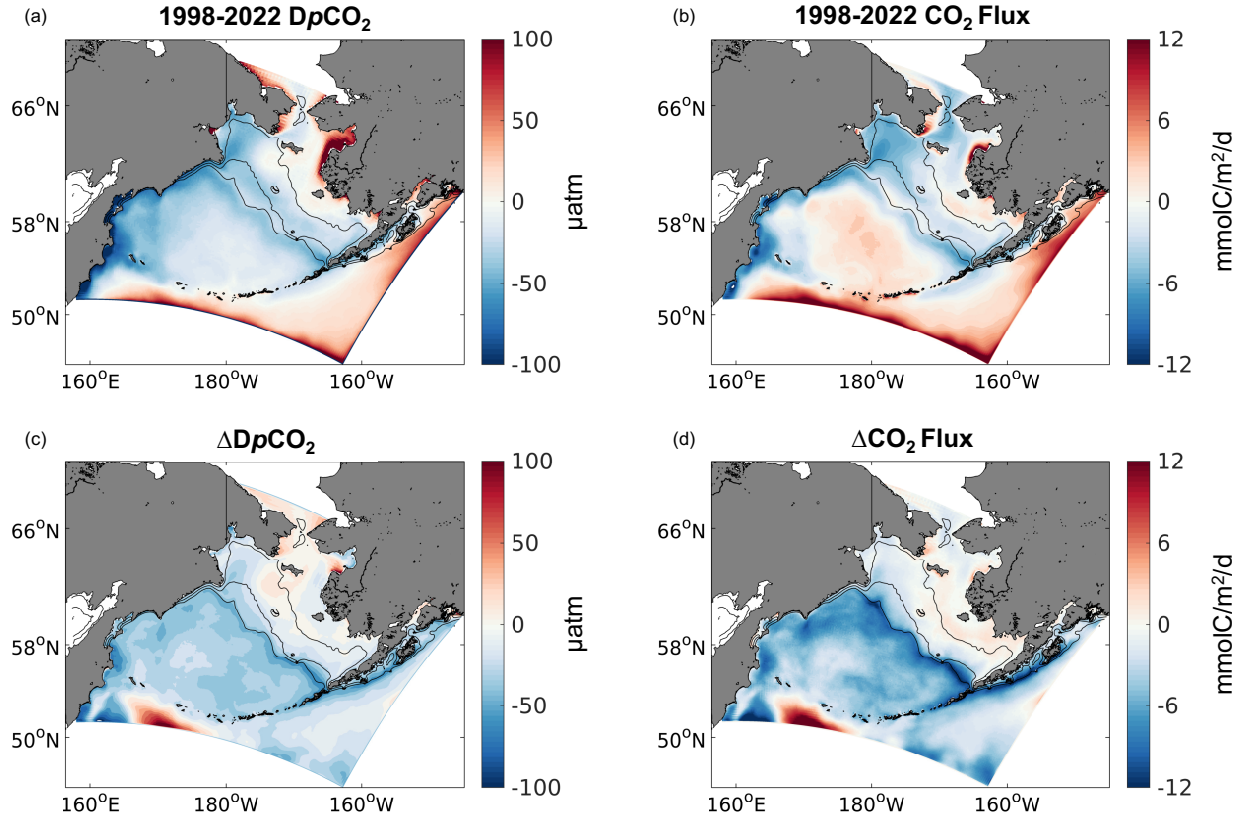
Figure 11: Spatial plots of model annual average surface (a) DpCO 2 and (b) CO 2 flux from 1998-2022. Also shown is (c) ΔDpCO 2 and the (d) ΔCO 2 flux calculated as the difference between the 1998-2022 and the 1970-1994 timeframes.
