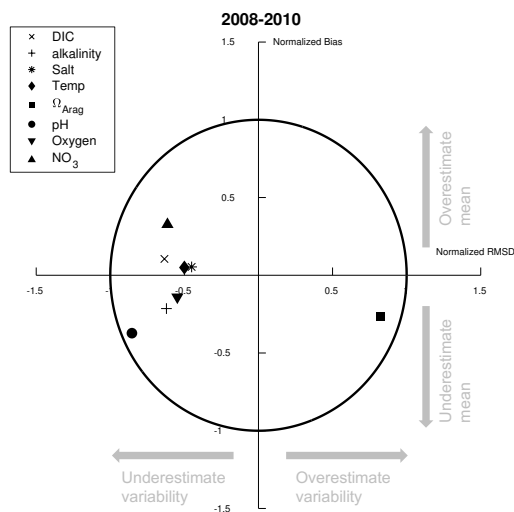
340 Figure 3: Target diagram summarizing the data comparison from Fig. 2. Here, the X-axis is the normalized unbiased RMSD between the model and data, multiplied by the sign of the difference between model and observed standard deviation. The Y-axis is the normalized mean bias.
