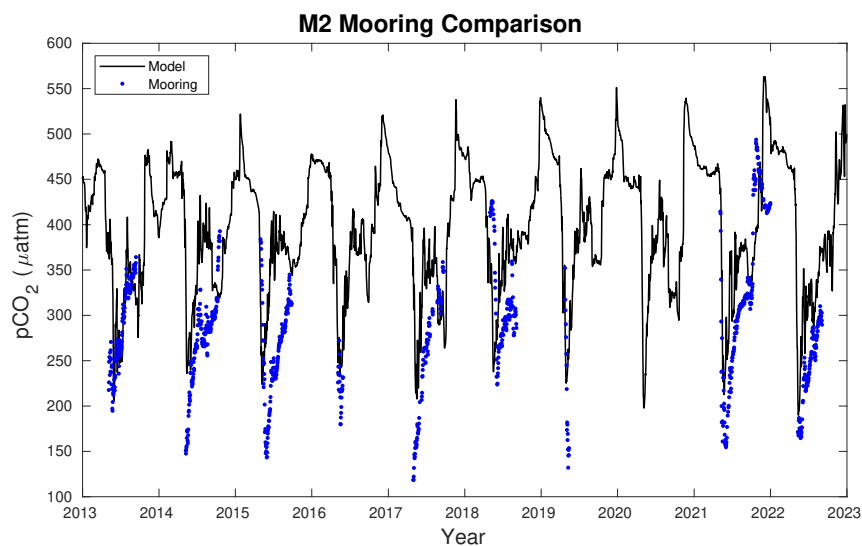
345 Figure 4: M2 mooring p\text{CO}_2 data (blue dots) compared to model daily p\text{CO}_2 values (black line) at the equivalent model grid cell location. The mooring is generally deployed in spring and retrieved in fall, though was out much later in 2021.
