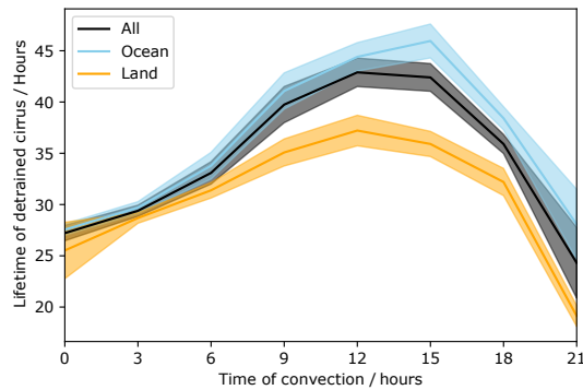
Figure 5. Total distribution-Lifetime of detrained cirrus as a function of the lifetimes-timing of ocean-origin the initial convection for all, land, and land-origin ocean origin cirrus. The error bars represent the interannual variability over the study period.
