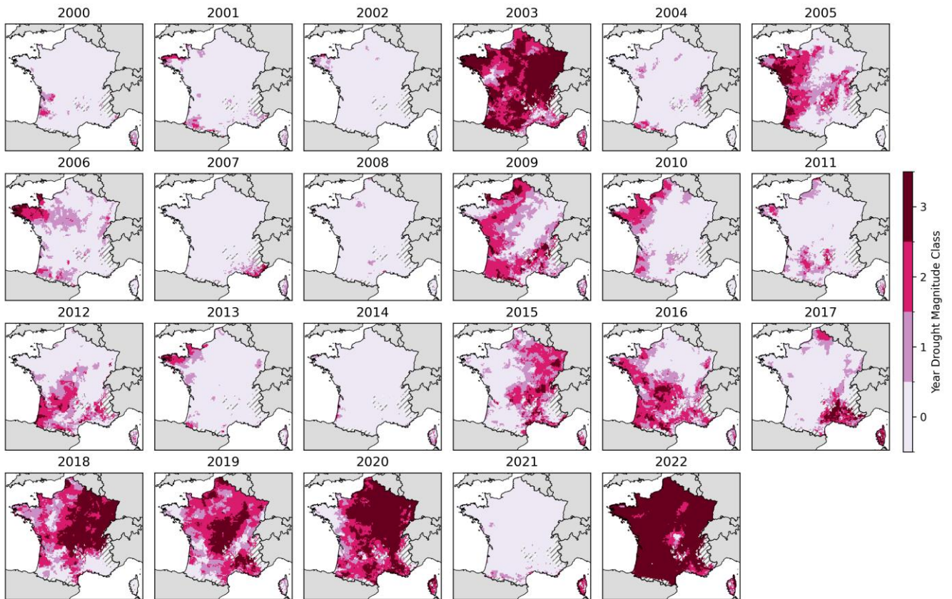
Figure S3 – Year drought magnitudes in classes for years 2000 to 2022, computed over France in each grid point from the ISBA historical simulation. Areas with gray hatching correspond to filtered mountain areas (average altitude > 1100 meters).
