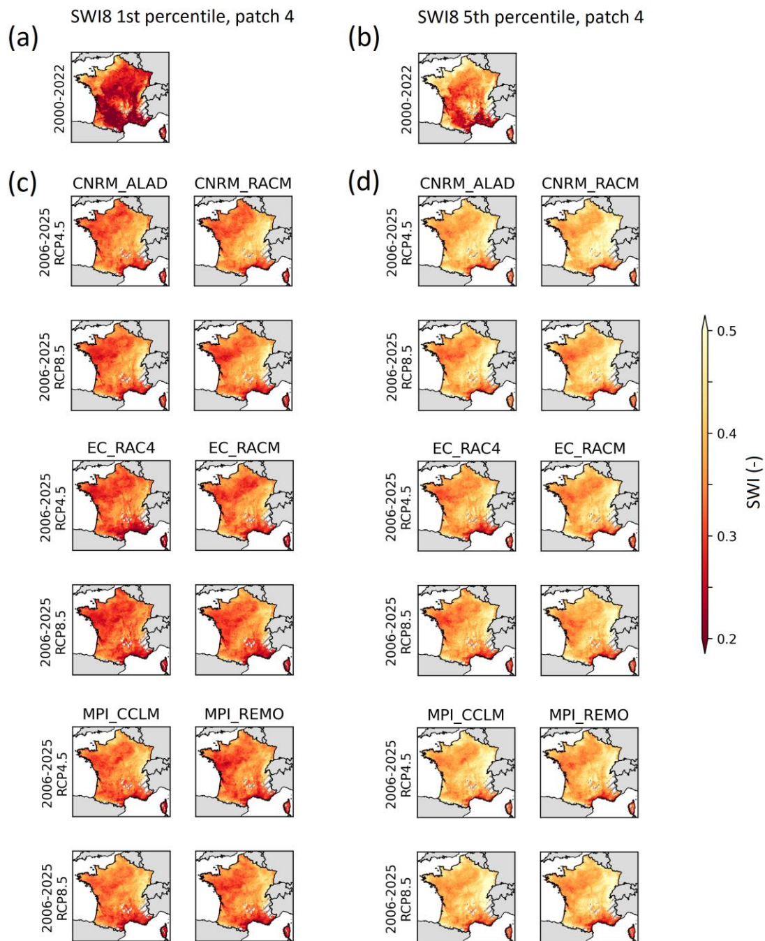
Figure S2 – Drought threshold values for (a,b) historical, and (c,d) projected simulations: (a,c) 1 st percentile, (b,d) 5 th percentile, for deciduous broadleaf trees (patch number 4), soil layer 8 (80-100 cm).
