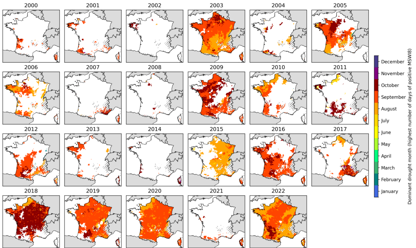
Figure S4 – Dominant drought month (highest number of days with positive magnitude) for years 2000 to 2022, computed over France in each grid point from the ISBA historical simulation. Areas with gray hatching correspond to filtered mountain areas (average altitude > 1100 meters).
