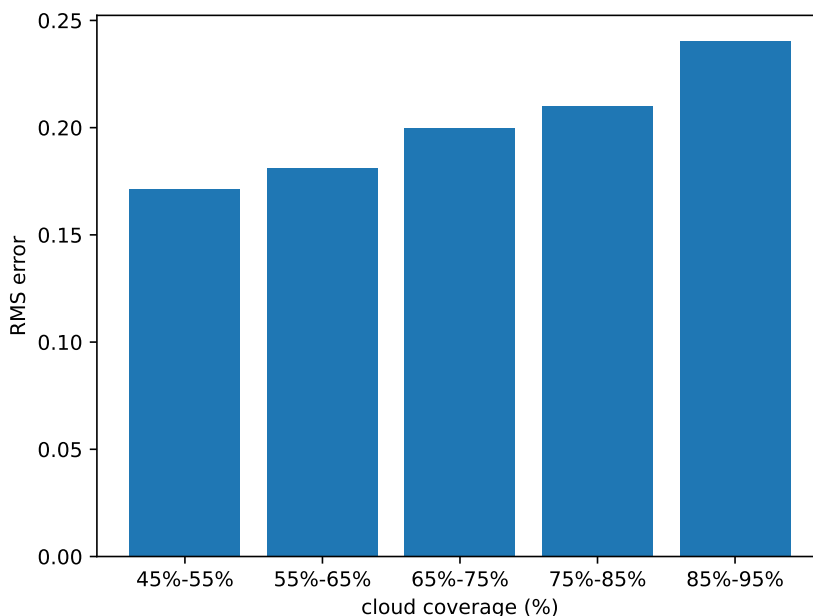
Figure 11. Impact of cloud coverage on the RMS computed relative to independent data (units \log_{10} \text{mg m}^{-3} )
