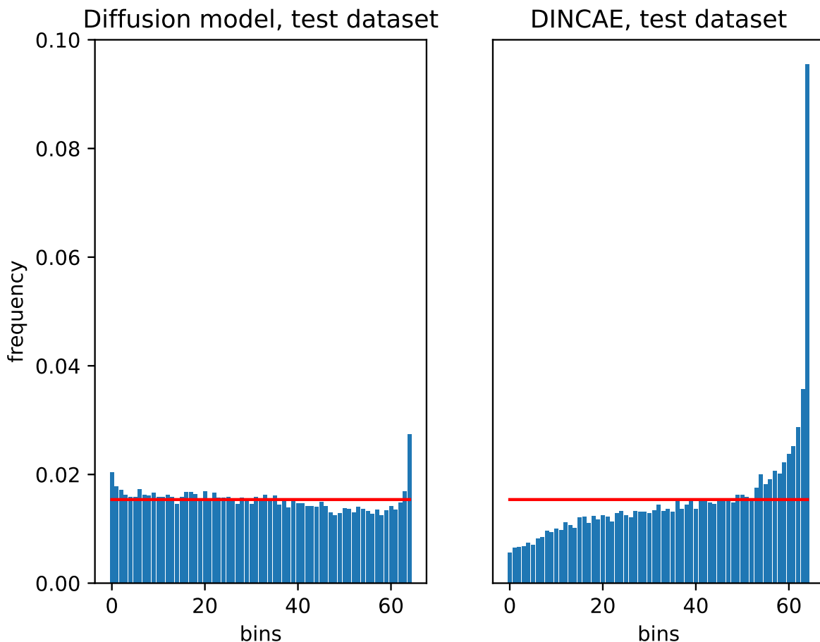
Figure 10. Talagrand diagram of the diffusion model and the DINCAE method for the independent test datasets.
