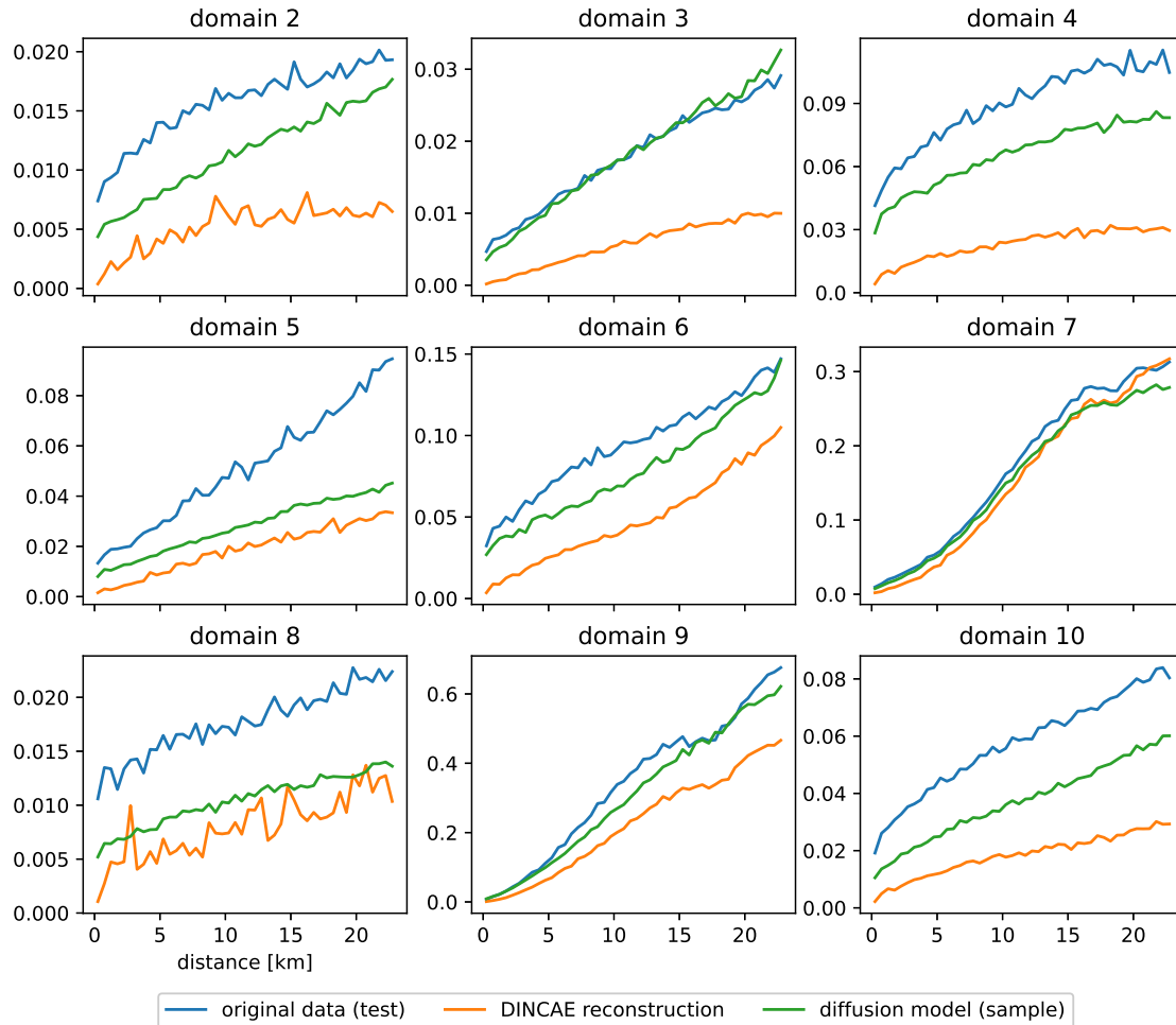
Figure 13. Variogram for the independent test data for the additional domains
