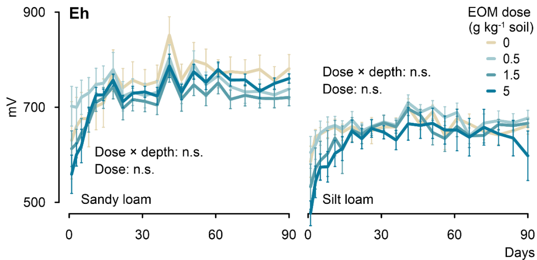
300 Figure 5. Evolution of the soil redox potential measured at 5 and 15 cm depth across the 90-day incubation experiment for the sandy loam and silt loam soils amended with different doses of EOM (ryegrass). Error bars show standard errors of means ( n = 6 ).
