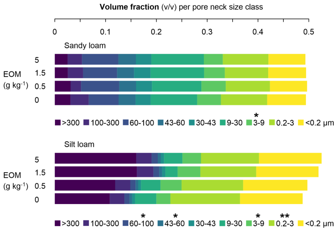
315 Figure 6. Volume fraction (unitless) of nine pore neck size classes (i.e. pores with given intervals of the pore neck diameter) in the sandy loam and silt loam soils after the application of EOM (ryegrass) doses and an unamended control (n = 4). * represent significant differences (one-way ANOVA) of the volume fraction of the pore neck class between EOM doses within each soil texture, with *** < 0.001, ** < 0.01, * < 0.05, and • < 0.1.
