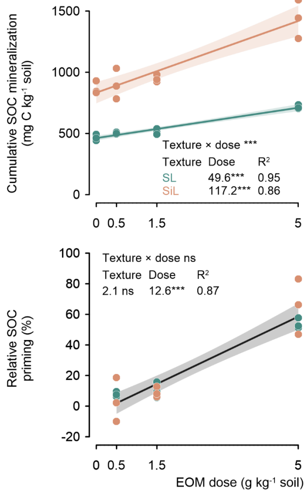
Figure 3. Cumulative mineralized native SOC (mg C kg -1 ) after 90 days for a sandy loam (SL) and a silt loam (SiL) soil as a function of EOM (ryegrass) application dose (upper figure). The lower graph compares the extra amount of SOC mineralized vs. the unamended controls and relative to the unamended controls, i.e. EOM addition induced priming of native SOC in both soil textures. * denote significance levels of the linear model interaction effect between soil texture and EOM dose, and for the linear response of cumulative and primed SOC mineralization to EOM dose, with *** <0.001, ** <0.01, * <0.05, and n.s. = not significant. Polygons around regression lines represent 95% confidence intervals.
