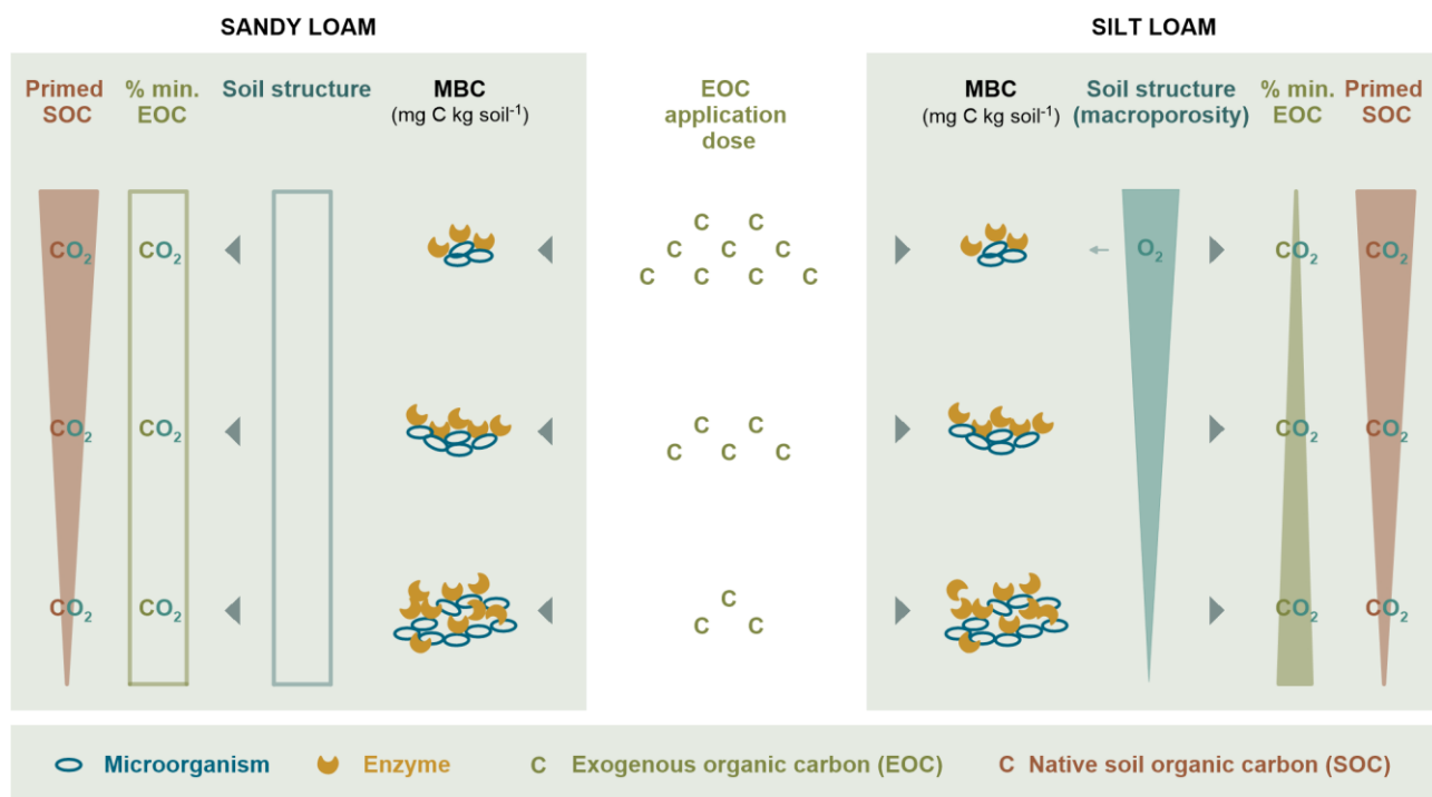
Figure 8. Overview of the mechanisms shaping the relative EOC mineralization (% min. EOC) and SOC priming effects in response to EOM application dose. In the sandy loam soil (left-hand side), increasing EOM dose supplied energy for microbial growth and extracellular enzyme production, which possibly degraded native SOC (i.e. co-metabolism), but did not affect the mineralized EOM fraction. Soil Eh decreased slightly with increasing EOM dose, but C mineralization remained aerobic as expected in the sandy loam soil. Here, soil structure was not much affected by EOM dose. In the silt loam soil (right-hand side), where O 2 diffusion is expected to be inherently constrained, increasing EOM dose induced macroporosity which also compensated the large O 2 consumption due to larger microbial growth. Here, mainly co-metabolism could explain the positive priming effects with increasing EOM dose in the silt loam soil. The decreasing percentage of decomposed EOM with increasing EOM application dose observed in the silt loam soil might be related to larger EOM protection within aggregates, but further confirmation of this hypothesis is required.
