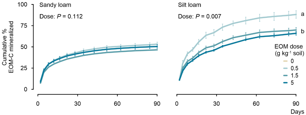
Fig. A1. Cumulative % EOM-C mineralized over the 90-day incubation experiment for a sandy loam and silt loam soils as a function of application dose. P values indicate the effect of application dose on the percentage of EOM mineralized at the end of the experiment. Error bars show standard errors of means ( n = 3).
