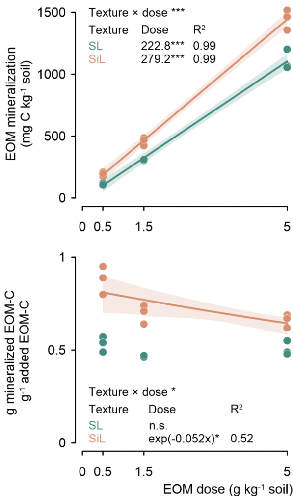
Figure 2. Cumulative mineralized EOM C (ryegrass) after 90 days since incorporation in sandy loam (SL) or silt loam (SiL) soil as a function of its application dose (upper figure). The lower figure presents the proportion of mineralized ryegrass C as a function of EOM dose. * denote significance levels of the linear model interaction effect between soil texture and EOM dose, and for the linear or exponential response of EOM mineralization to EOM dose, with *** < 0.001 , ** < 0.01 , * < 0.05 , and n.s. = not significant. Polygons around regression lines represent 95% confidence intervals.
