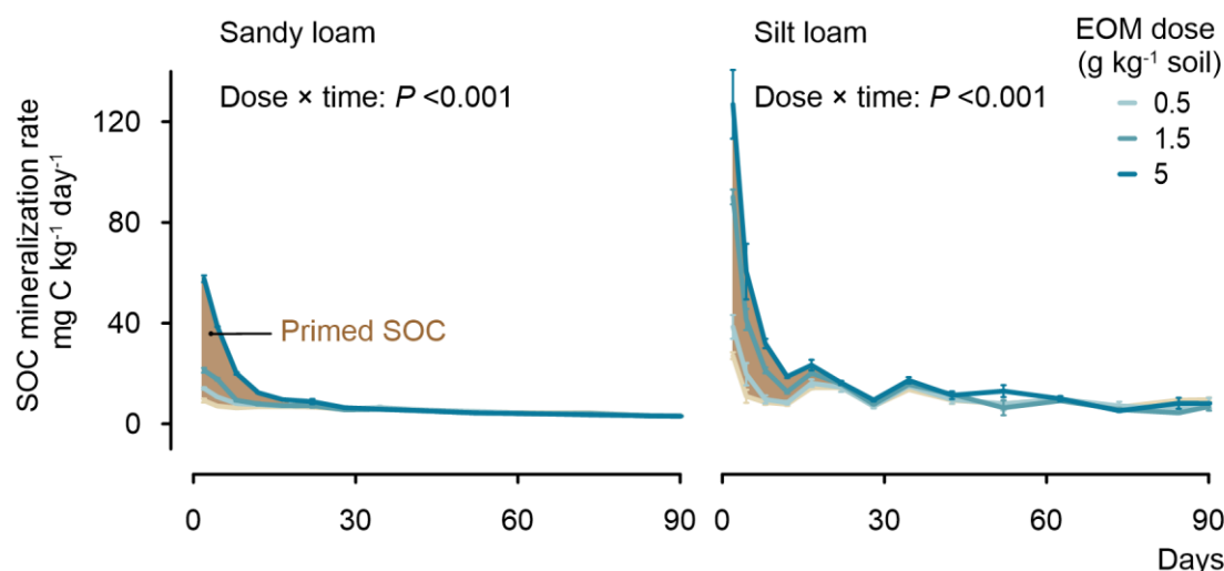
510 Fig. B1. The SOC mineralization rates over the 90-day incubation experiment for a sandy loam and a silt loam soil in response to EOM application dose. Shadow brownish areas depict priming of SOC mineralization caused by EOM application dose. In sandy loam soil, EOM dose induced SOC priming between days 2 and 12 of the incubation ( P values for 1.5 g kg -1 vs. control = 0.03; 5 g kg -1 vs. control <0.001; 5 vs. 0.5 g kg -1 <0.001; and, 5 vs. 1.5 g kg -1 <0.001), whereas priming remained not significant during day 12 to 90. In silt loam 515 soil, EOM dose induced SOC priming between days 2 and 17 of the incubation ( P values for 5 g kg -1 vs. control = 0.001; 5 vs. 0.5 g kg -1 = 0.002; and, 5 vs. 1.5 g kg -1 = 0.01), while priming was not significantly different between EOM doses from day 17 to 90. Error bars show standard errors of means ( n = 3 ).
