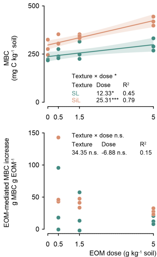
Figure 4. Microbial biomass carbon (MBC) after 45 days of incubation of the sandy loam (SL) and silt loam (SiL) soils amended with EOM (ryegrass) at various application doses (upper figure). The corresponding EOM-mediated MBC increase is presented in the lower figure. * denote significance levels effects of the linear model interaction between soil texture and EOM dose, and the effect of EOM dose on MBC and EOM-mediated MBC increase, with *** <0.001, ** <0.01, * <0.05, and n.s. = not significant. Polygons around regression lines represent 95% confidence intervals.
