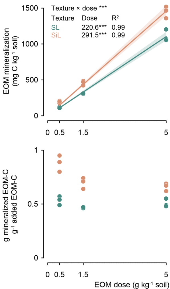
265 Figure 2. Cumulative mineralized EOM-C (ryegrass) after 90 days since incorporation in sandy loam (SL) or silt loam (SiL) soil as a function of its application dose (upper figure). The lower figure presents the proportion of mineralized ryegrass C as a function of EOM dose. *** denote significance levels < 0.001 of the linear model interaction effect between soil texture and EOM dose, and for the linear response of EOM mineralization to EOM dose. Since no EOM mineralization was expected in the absence of added EOM, a linear model through the origin was fitted for the cumulative EOM mineralization. Polygons around regression lines represent 95% confidence intervals.
