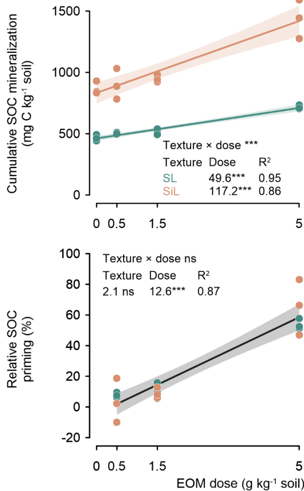
Figure 3. Cumulative mineralized native SOC (mg C kg -1 ) after 90 days for a sandy loam (SL) and a silt loam (SiL) soil as a function of EOM (ryegrass) application dose (upper figure). The lower graph compares the extra amount of SOC mineralized vs. the unamended controls and relative to the unamended controls, i.e. EOM addition induced relative priming of native SOC mineralization in both soil textures. * denote significance levels of the linear model interaction effect between soil texture and EOM dose, and for the linear response of cumulative and primed SOC mineralization to EOM dose, with *** < 0.001, ** < 0.01, * < 0.05, and n.s. = not significant. Polygons around regression lines represent 95% confidence intervals.
