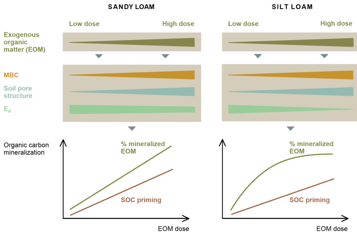
Figure 1. Expected outcomes and hypotheses of the EOM application dose effect on EOM and native SOC mineralization in a sandy loam and a silt loam soils. Overall, we expect the proportion of EOM mineralization to increase with higher EOM doses in sandy loam soil due to closer contact between EOM and microbes at higher doses. In silt loam soil, the proportion of EOM mineralization is expected to level off at higher doses, due to a higher chance of limited O 2 supply, which may restrict aerobic microbial activity compared to sandy loam soil. Priming of SOC mineralization is expected to increase with higher EOM doses because of enhanced co-metabolism and formation of macroporosity, macroporosity, and co-metabolism.
