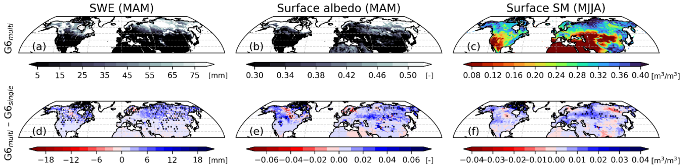
490 Figure 3: Spatial distribution of climatological (a) snow water equivalent (March–May), (b) surface albedo (March–May), (c) surface soil moisture (May–August) from GloSea6 ( G6_{multi} ) initiated on 1 st March of 1993–2016. (d, e, f) Their difference maps compared to G6_{single} , where the dotted area indicates the difference is statistically significant at a 95% confidence level after FDR control across the grid.
