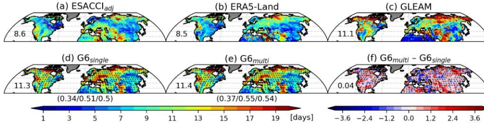
Figure 4: Surface SMM from (a) ESACCI adj , (b) ERA5-Land, (c) GLEAM, (d) G6_{single} , (e) G6_{multi} , and (f) the difference between G6_{multi} and G6_{single} . NH mean values are denoted in the middle-left in each panel. The bracketed values indicate the spatial correlation of the modelled soil moisture memory compared to ESACCI adj (left), ERA5-Land (middle), and GLEAM (right). Dotted areas represent statistical significance of SMM difference between models and observations (d–e) and between models (f) at the 99% confidence level from a Monte Carlo method.
