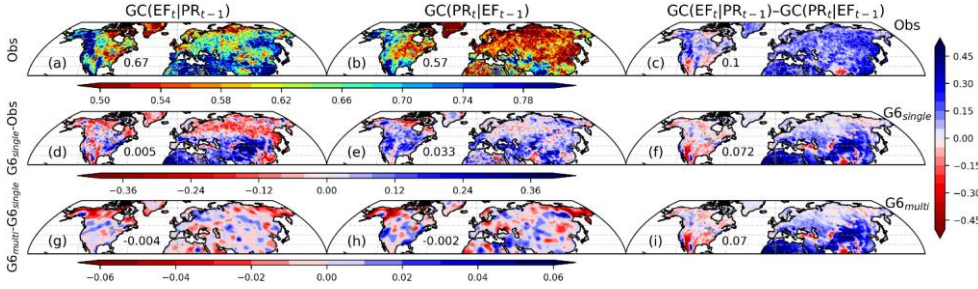
Figure 6: Spatial distribution of 1-day lagged Granger causality (1- p value) with evaporative fraction and precipitation. The observed causalities (a) GC(EF_t|PR_{t-1}) , (b) GC(PR_t|EF_{t-1}) , and (c) their difference in which blue and red color indicates the dominance of feedback direction in GC(EF_t|PR_{t-1}) and GC(PR_t|EF_{t-1}) , respectively. The model biases of G6_{single} compared to observations for the causality in (d) GC(EF_t|PR_{t-1}) , (e) GC(PR_t|EF_{t-1}) , and (f) the difference between GC(EF_t|PR_{t-1}) and GC(PR_t|EF_{t-1}) in G6_{single} . The difference maps of (g) GC(EF_t|PR_{t-1}) and (h) GC(PR_t|EF_{t-1}) between G6_{single} and G6_{multi} and (i) the difference between GC(EF_t|PR_{t-1}) and GC(PR_t|EF_{t-1}) in G6_{multi} .
