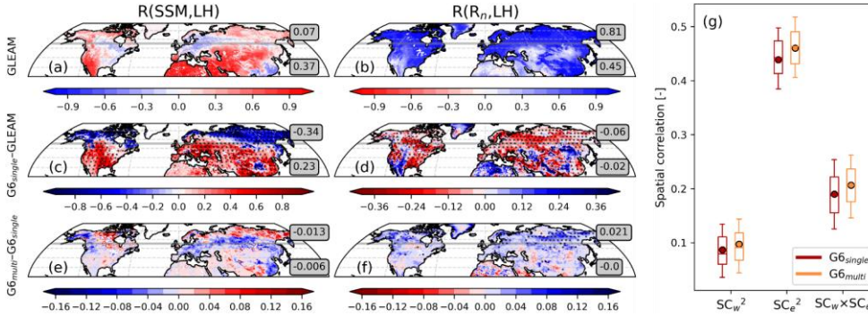
Figure 7: Spatial distribution of R(SSM, LH) (left column; water-limited coupling) and R(R_n, LH) (middle column; energy-limited coupling) in (a, b) GLEAM, (c, d) model biases of G6_{single} compared to observations, and (e, f) differences between G6_{single} and G6_{multi} , where grey horizontal lines in each panel separate to mid- (20–55N) and high-latitude (55–80N) areas and area averaged values is denoted within grey shaded box. The dotted areas in (c)–(f) indicate statistical significance at a 95% confidence level after FDR control across the grid. (g) Boxplot of the squared spatial pattern correlation coefficient as a measure of the spatial agreement of R(SSM, LH) ( SC_w ) and R(R_n, LH) ( SC_e ) in G6_{single} (red) and G6_{multi} (orange) over the northern hemisphere against GLEAMv4.2a. Boxes show the median and interquartile range (IQR: 25th and 75th percentiles), and whiskers represent \pm 0.5IQR from the 25th and 75th percentiles, respectively, and dotted circles indicate the sampled average. In the rightmost column, SC_w \times SC_e quantifies the coherency of water- and energy-limited processes in both models.
