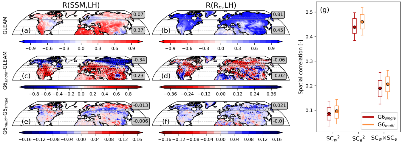
580 Figure 7: Spatial distribution of R(SSM, LH) (left column; water-limited coupling) and R(R_n, LH) (middle column; energy-limited coupling) in (a, b) GLEAM, (c, d) model biases of G6_{single} compared to observations, and (e, f) differences between G6_{single} and G6_{multi} , where grey horizontal lines in each panel separate to mid- (20–55N) and high-latitude (55–80N) areas and area averaged values is denoted within grey shaded box. The dotted areas in (c)–(f) indicate statistical significance at a 95% confidence level after FDR control across the grid. (g) Boxplot of the squared spatial pattern correlation coefficient as a measure of the spatial agreement of R(SSM, LH) ( SC_w ) and R(R_n, LH) ( SC_e ) in G6_{single} (red) and G6_{multi} (orange) over the northern hemisphere against GLEAMv4.2a. Boxes show the median and interquartile range (IQR: 25th and 75th percentiles), and whiskers represent \pm 0.5IQR from the 25th and 75th percentiles, respectively, and dotted circles indicate the sampled average. In the rightmost column, SC_w \times SC_e quantifies the coherency of water- and energy-limited processes in both models.
