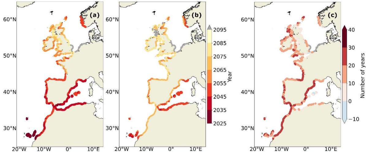
Figure S2.1: (a) Year in which the HCE will occur once a year in the future under the SSP5-8.5 scenario for the ESWL. (b) same for the ETWL. (c) Differences between (b) and (a). The grey dots indicate the locations where HCEs recur annually after 2095.
