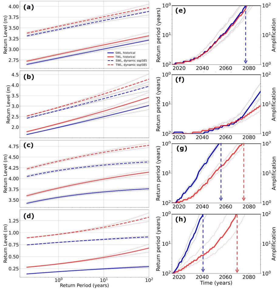
Figure S2.2: Left: Return period curves for ESWL (blue) and ETWL (red) over the 1995-2014 period (solid lines) and under the SSP5-8.5 scenario over the 2081-2100 period (dashed lines) at the four different locations of Figure S2.1: (a) the Scottish coasts (b) the southern North Sea coasts (c) the Brittany coasts in France (d) the western Mediterranean coasts. Right: Amplification of the HCE under the SSP5-8.5 scenario as a function of time for the same 4 locations for ESWL (blue) and TWL (red). The arrows represent the year in which the HCE will occur once a year in the future.
