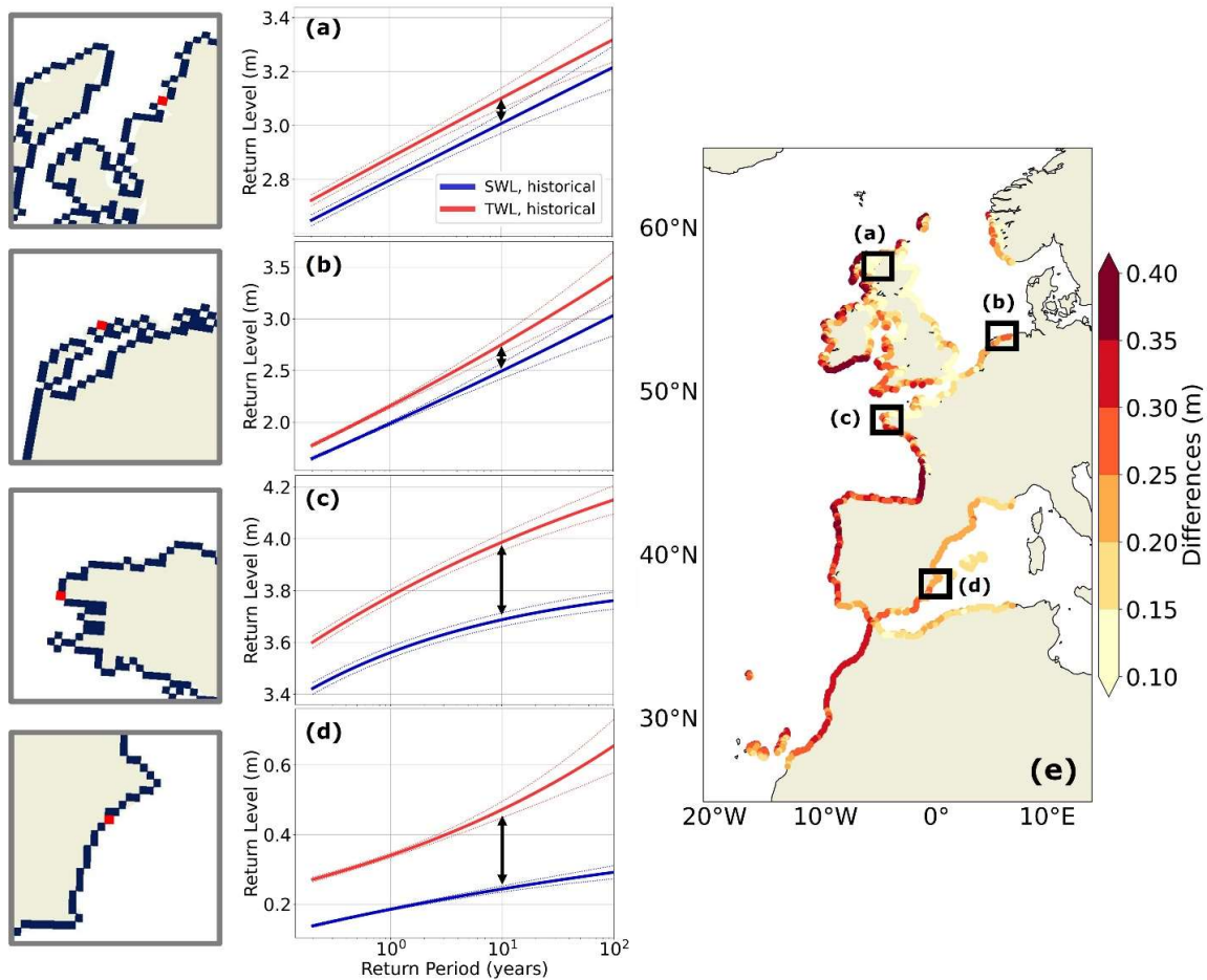
Figure S1.1: Return period curves for ESWL (blue) and ETWL (red) computed over 1995-2014 at 4 different locations marked on the map on the right (a) the Scottish coasts (b) the southern North Sea coasts (c) the Brittany coasts in France (d) the western Mediterranean coasts. Note the different y-axes for the different panels. The 4 thumbnails on the left highlight in red the selected coastal points in the regional ocean simulations corresponding to a horizontal resolution of about 10 km. (e)
