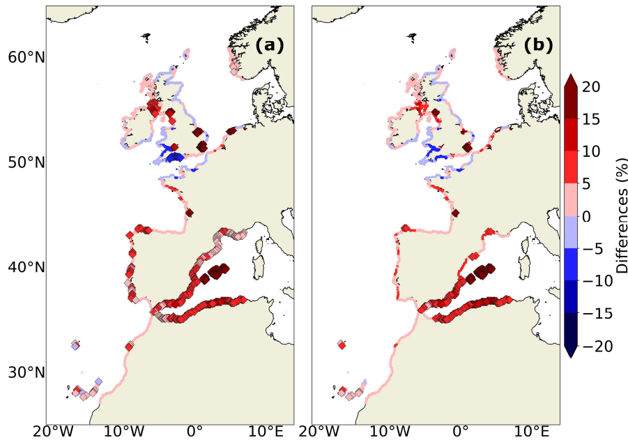
Figure S5.1: (a) Differences (in %) in the projected changes (2081-2100 minus 1995-2014) in the 1-in-5-year ESLs between the dynamic and static approaches. (b) same for the 1-in-100-year ESLs. The diamonds represent the locations where the differences are significant i.e. where the 95% confidence intervals associated with return level calculations for the static and dynamic approaches are disjoint (Fig. 2b).
