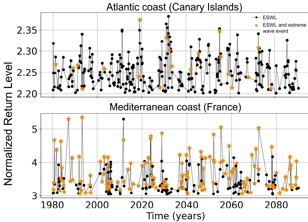
Figure 9: Illustration of the selected ESWLs (black dots and yellow stars) as a function of time for the whole period at two different locations, with black dots when ESWLs did not co-occur (i.e. within a 3-day window) with an extreme wave event, and with yellow stars when the ESWL co-occurred (within a 3-day window) with an extreme wave event (defined by the wave scaling \sqrt{H_s L_p} ). The more yellow stars in the graph, the more ESWL and extreme wave events co-occur. Note that the y-axis shows normalized extremes levels (by the trend and variability, see Sect. 2.4, eq (4)) and not the simulated extremes in meters.
