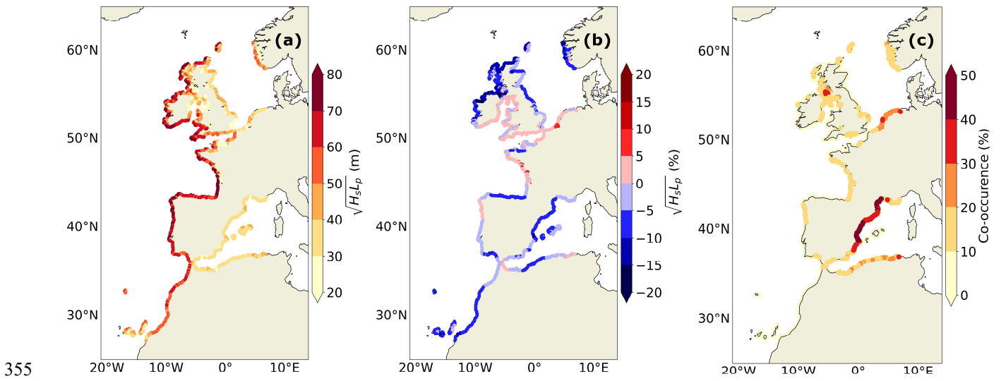
Figure 8: (a) The 1-in-10-year wave contribution scaling ( \sqrt{H_s L_p} , in m) for the 1995-2014 historical period. (b) Future changes (2081-2100 minus 1995-2014) in the 1-in-10-year event for the wave contribution scaling ( \sqrt{H_s L_p} , in %) under the SSP5-8.5 scenario. (c) Percentage of time when ESWL and extreme wave events (defined by the wave scaling \sqrt{H_s L_p} ) co-occur during the 1970-2100 period. It is defined as the ratio between the number of co-occurrences within a 3-day period and the total number of selected ESWL peaks, as illustrated in Figure 9.
