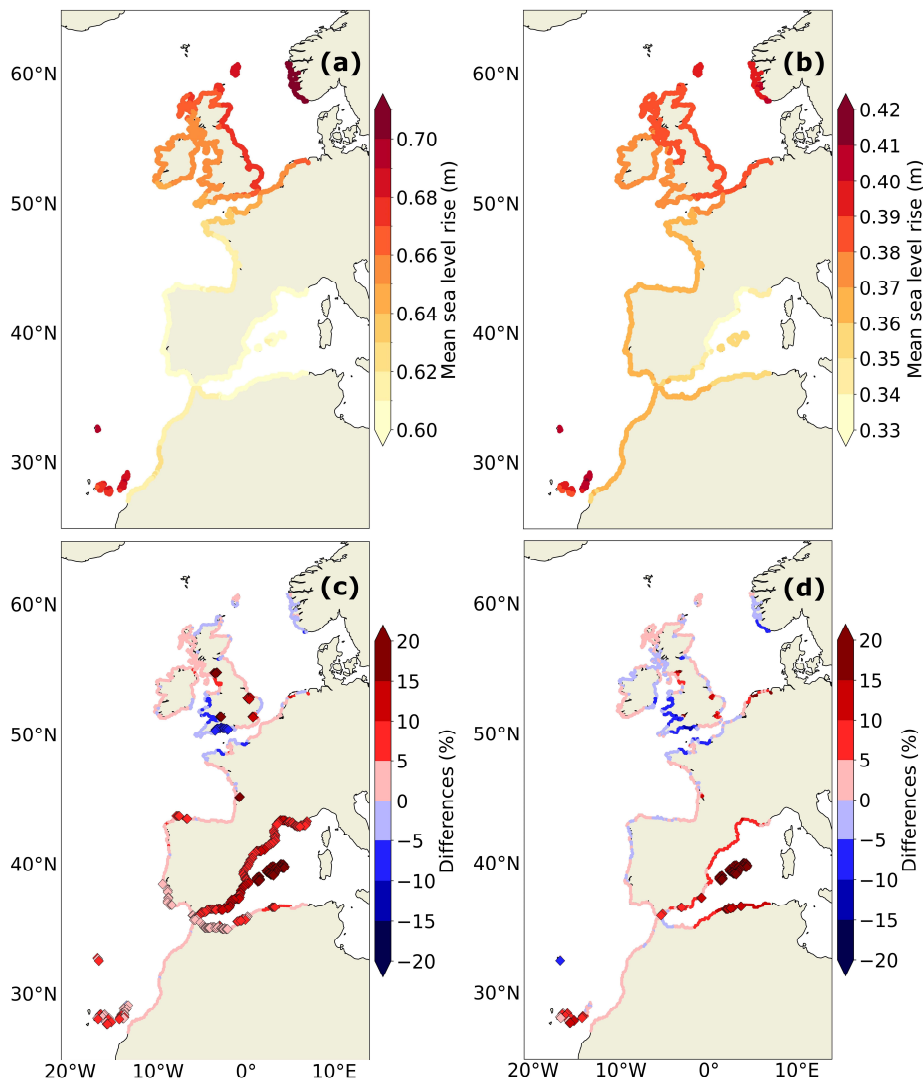
310 Figure 6: (a) Future changes (2081-2100 minus 1995-2014) in ESWLs using the static approach (i.e. corresponding to the mean SLR shift from the GCM) for the SSP5-8.5 scenario. (b) Same for the SSP1-2.6 scenario. The 1-in-10-year return levels for the historical baseline (1970-2014) are shown in Fig. 3a. (c) Differences (in %) in the projected changes (2081-2100 minus 1995-2014) in the 1-in-10-year ESWLs between the dynamic and static approaches for the SSP5-8.5 scenario. (d) same for the SSP1-2.6 315 scenario. The diamonds represent the locations where the differences are significant i.e. where the 95% confidence intervals associated with the 1-in-10-year return level calculation for the static and dynamic approaches are disjoint (Fig. 2b).
