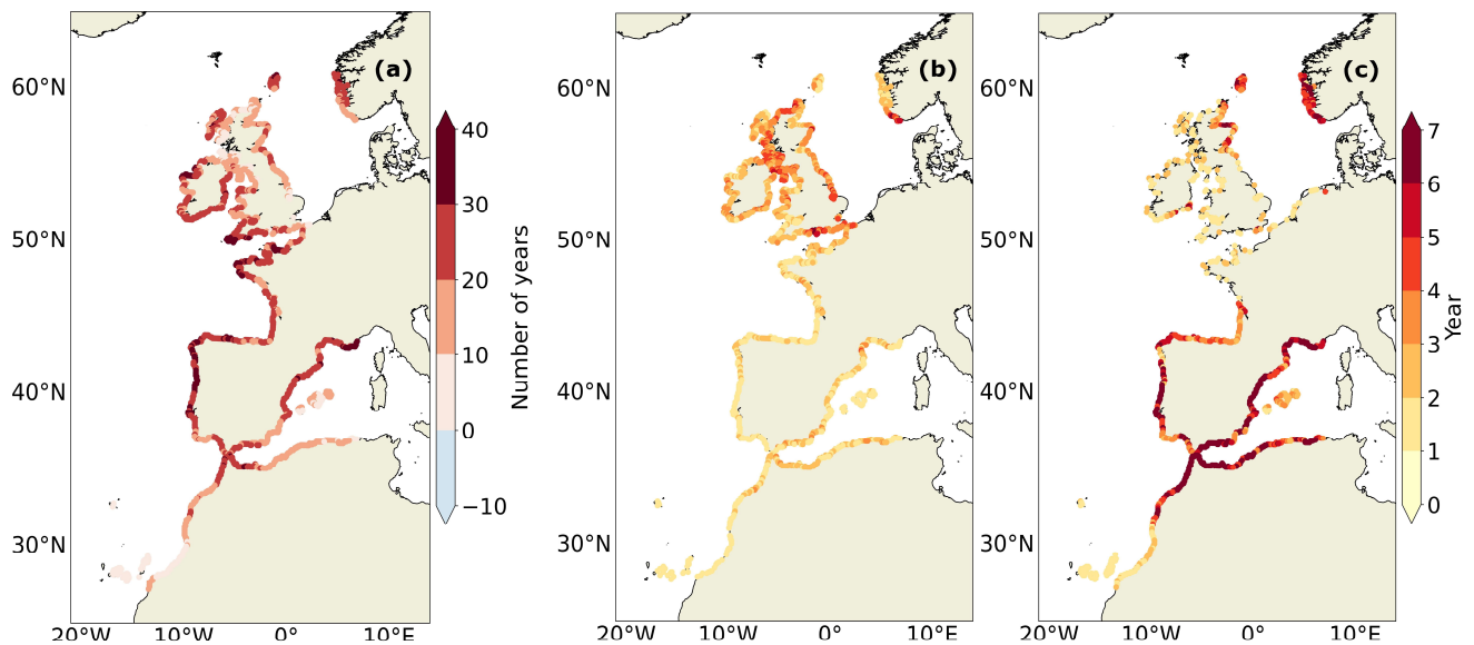
Figure 5: Differences in the year in which the HCE will occur once a year between the SSP1-2.6 and the SSP5-8.5 scenarios for the SWL (Fig. 4b minus Fig. 4a). Only the regions where the confidence intervals of the two scenarios do not overlap are indicated. (b) Confidence intervals for the SSP5-8.5 scenario. (c) Same for the SSP1-2.6 scenario.
