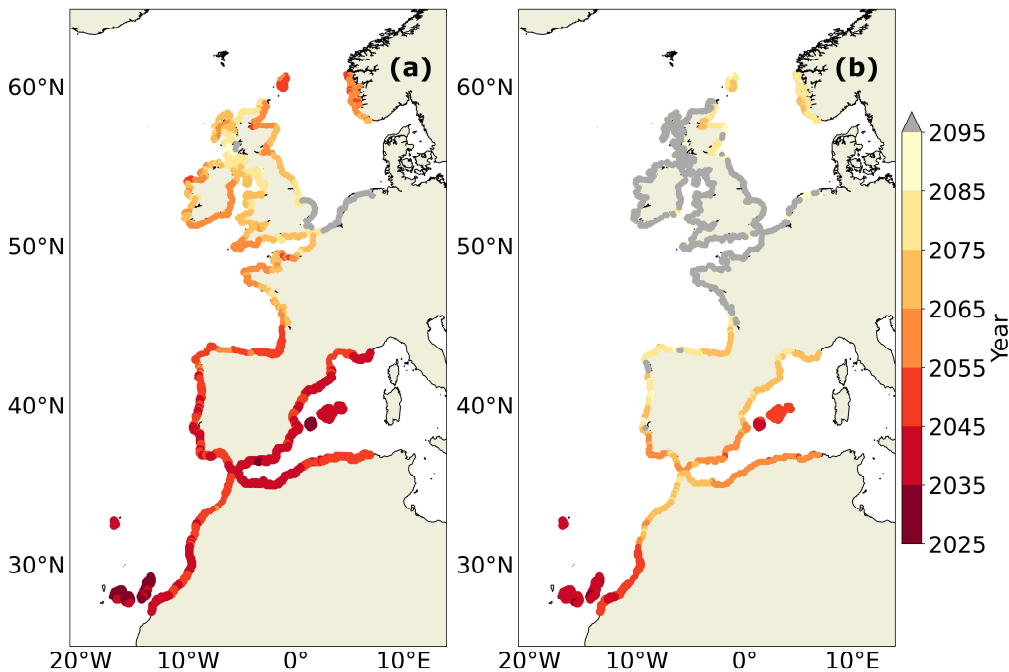
280 Figure 4: (a) Year in which the HCE will occur once a year in the future under the SSP5-8.5 scenario for the SWL. The grey dots indicate the locations where HCEs do not recur annually before 2095. (b) same under the SSP1-2.6 scenario.
