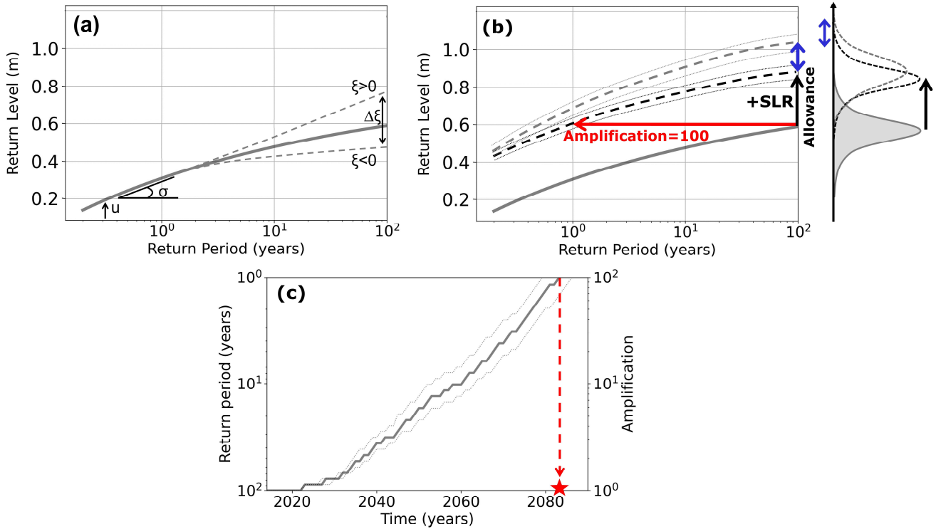
205 Figure 2: Diagram with the different concepts used in the extreme event analyses. (a) Relation between ESLs (return levels, in m) and associated return periods (in years). The distribution parameters are represented in black: u the location parameter (threshold), \sigma the scale parameter and \xi the shape parameter for the past period (grey solid line). Graphically, the threshold for the selection of extremes corresponds to the return level reached for a return period of 1/3 years as 3 events per year are selected. (b) Same as a) but adding the curves for a future scenario (dashed lines), in black with the static approach which consists in adding an offset to the return level corresponding to mean SLR (black arrows), in grey with a dynamic approach which consists in considering also changes in the different coastal sea level contributions. The differences are also schematized with distributions on the right side of panel (b). The blue arrows indicate the difference between both approaches. The difference is considered significant when the confidence intervals (dotted lines) are disjoint. (c) Amplification of the past centennial event (HCE, 1-in-100-year event) as a function of time. The red star highlights the year in which the HCE will become a yearly event i.e., when the amplification factor reaches 100.
