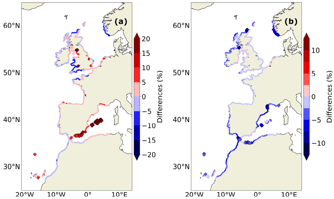
330 Figure 7: (a) Differences (in %) in the future changes (2081-2100 minus 1995-2014) in the 1-in-10-year ETWLs between the dynamic and static approaches under the SSP5-8.5 scenario (i.e., same as Fig. 6c but for the ETWLs, therefore including waves). (b) Impact of the inclusion of the dynamic changes in waves on the future ESLs (i.e., differences between Fig. 7a and Fig. 6c). Diamonds represent the locations where the differences between the static and dynamic approaches are significant (Fig. 2b).
