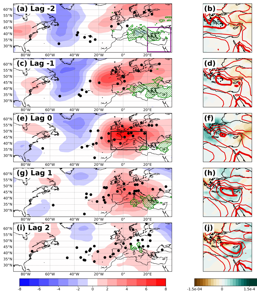
Figure 5. Time lag composite for the development of M cluster events. Lag 0 is defined as the day with maximum SLP value averaged over the Western Mediterranean (black box in (e)). (a,c,e,g,i) daily SLP anomalies (shading), RWB locations (full black circles) and statistically significant PV streamer positive density anomaly (green hatches). Negative anomalies omitted for clarity. (b,d,f,h,j) Time lag composite for the Eastern Mediterranean (purple box in (a)). Daily precipitation anomaly is shown in shading and SLP in contours (contour interval is 1 hPa and the lowest value is highlighted by a thick line).
