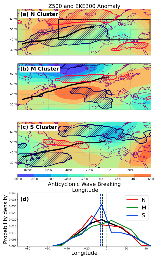
Figure 4. (a-c) Composite monthly geopotential height anomalies at 500 hPa (shading, 15m contour interval) and statistically significant EKE anomalies (defined the same as in fig. 2). Positive EKE anomalies are marked by red hatches, and negative in blue hatches. The thick curve denotes the average location of the Atlantic jet stream axis (300 hPa U maxima). (d) Longitude distribution of anticyclonic Rossby wave breaking events occurring at 200 hPa over the eastern Atlantic and northern Europe (black box in (a)). The climatological distribution in shown by the thick black histogram. Dashed vertical lines denote the median longitude of the climatology and of every cluster.
