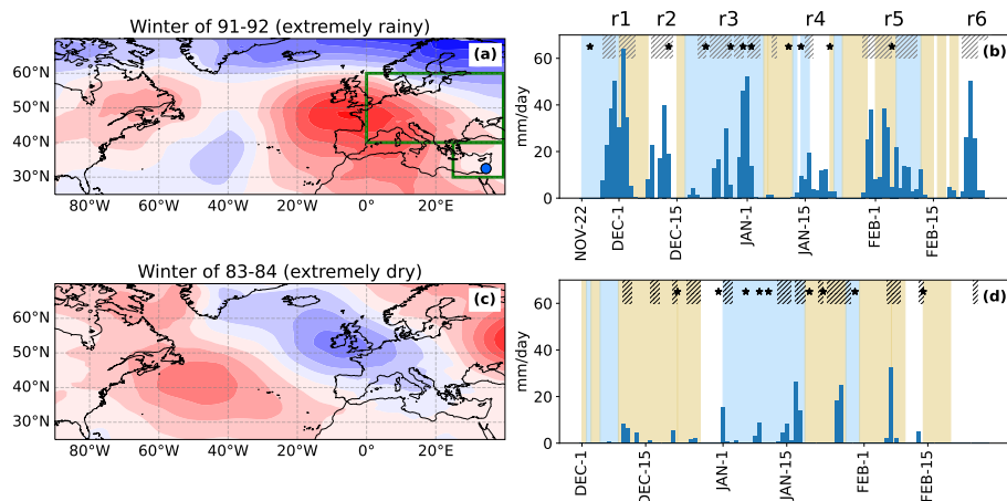
Figure 6. The course of two extreme winters in the Eastern Mediterranean. The top row shows the extremely rainy winter from December 1991 to February 1992, and the bottom row shows the December 1983-February 1984 dry winter. (a,c) SLP anomaly composites for all days belonging to the prominent cluster (cluster M for 91-92 and cluster S for 83-84). Blue and red shading denote negative and positive values, with a contour interval of 2 hPa. The top and bottom green boxes in (a) bound the domains used for RWB and PV streamer subset detection seen in (b,d). (b,d) Daily time series showing labeled days for the M cluster (blue shading), and the N+S clusters (yellow shading). Also shown are RWB events (star markers), PV streamers in the Eastern Mediterranean (hatches) and daily mean rainfall over Israel (blue bars; approximate rain gauge location marked by the blue circle in (a)). Both series show the entire season (DJF), with (b) extended back to November 22nd. The six major rain events during the 91-92 winter are labeled as r1-r6.
