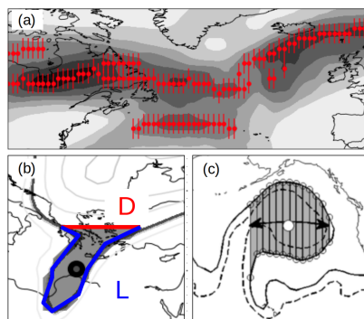
Figure 1. Examples of objectively detected features used in the analysis. (a) A snapshot of the daily EKE field (shading) and the EKE maxima used in the clustering (markers) for an example date (February 2nd 1979). The red markers denote the local meridional maxima in a 5 range, marked by vertical lines. (b) A PV streamer detected using the WaveBreaking algorithm. The thick grey isentrope is the 2PVU contour on a 315K surface. Shading marks the area of the streamer, and the red and blue lines mark its scale parameters (geographical distance D and contour length L , respectively). The center of the streamer is denoted by a circle marker. (c) An anticyclonic wave breaking event identified by the Strong & Magnusdottir algorithm. The solid and dashed lines mark the 5 and 3 isentropic PV contours on a 350K surface. Arrows show the zonal extent of the breaking and the white circle its centroid. (c) is adapted with permission from Figure 1 in Strong & Magnusdottir (2008).
