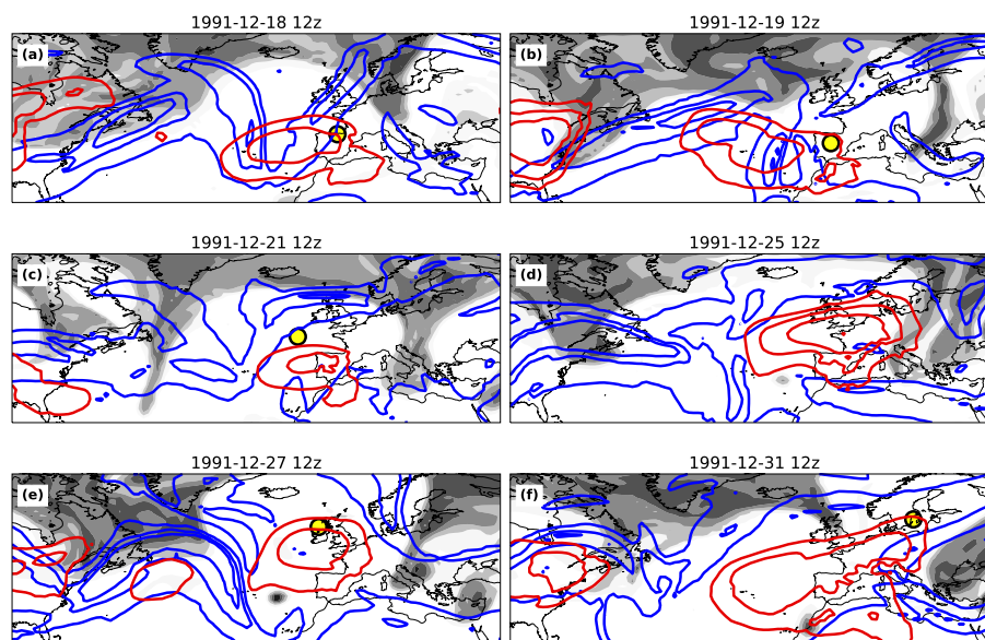
Figure 7. The progression of large scale flow during a 17-day rainy spell in Israel between Dec-18 1991 and Jan-3 1992 (r3 in figure 6b). Select days are shown to highlight the preceding conditions (a) and the following five PV streamers that crossed the region in succession (b-f). PV on a 315K isentropic surface is shown in shading (2 PVU minimal value, 1.5 PVU contour interval). The 300 hPa EKE field is denoted by blue contours ( 1000 \frac{m^2}{s^2} contour interval) and SLP is denoted by red contours (1030 hPa minimal value, 5 hPa interval). Yellow circles mark anticyclonic wave breaking events.
