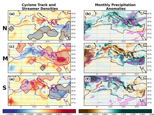
Figure 3. Composite cyclonic activity and precipitation for clusters N, M and S (top, middle and bottom row respectively). (a,c,e) Monthly cyclones track density anomaly (shading) and PV streamer density anomaly (hatches). For streamers, only statistically significant anomalies are shown (95% confidence on a 500 sample bootstrap test). (b,d,f) Monthly precipitation anomalies (shading). Areas with over 95% statistical significance are highlighted in pink hatches.
