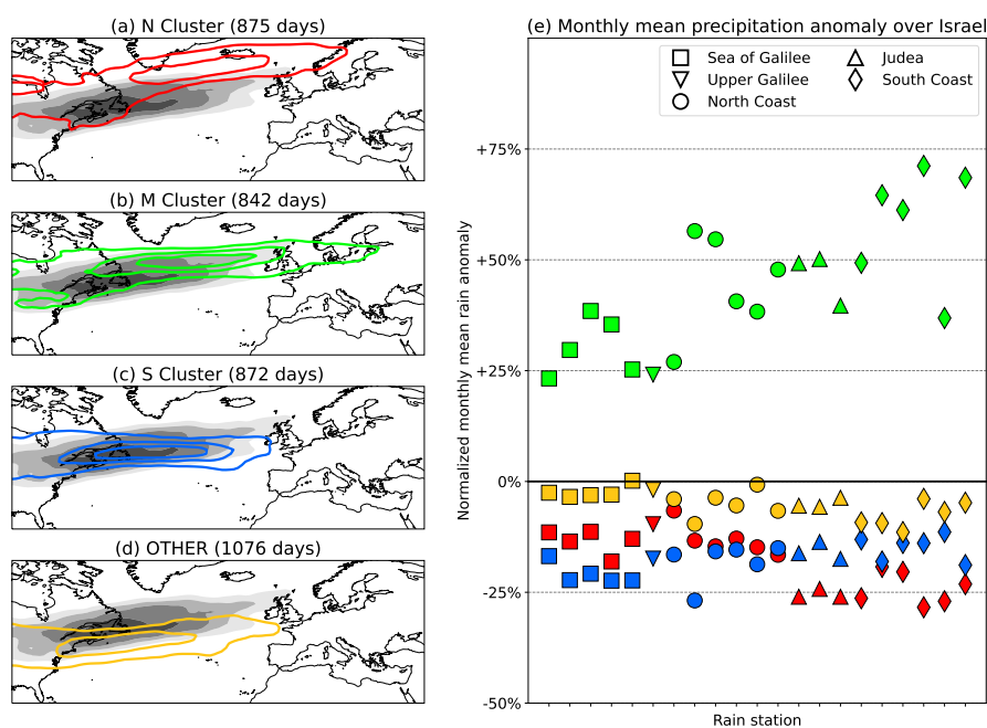
Figure 2. (a-d) North Atlantic storm track regimes, using k-means clustering on normalized daily DJF EKE data at 300 hPa. The clusters are represented by contours and the 1979-2019 climatology is in shading (contour interval is 0.05 for both). (e) The normalized mean monthly precipitation anomaly (%) for 21 rain stations in Israel for each cluster. Each anomaly is divided by the 1979-2019 DJF rain climatology of the corresponding station. The color of each marker denotes its cluster and its shape denotes its geographical location.
