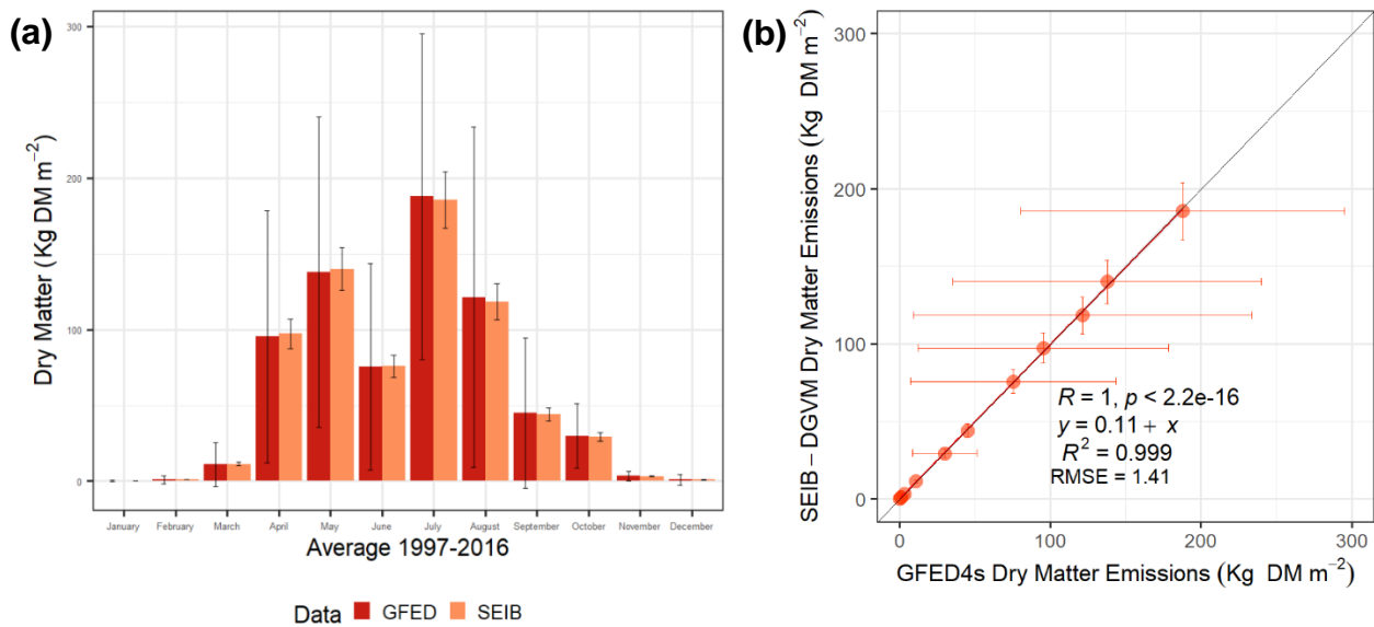
Figure 5. (a) Monthly temporal variability averaged dry matter emission of GFED4s and SEIB-DGVM from 1997 to 2016. (b) Comparison of monthly averaged dry matter emissions of GFED4s and SEIB-DGVM from 1997 to 2016. Standard deviation obtained from each monthly data from 1997 to 2016.
