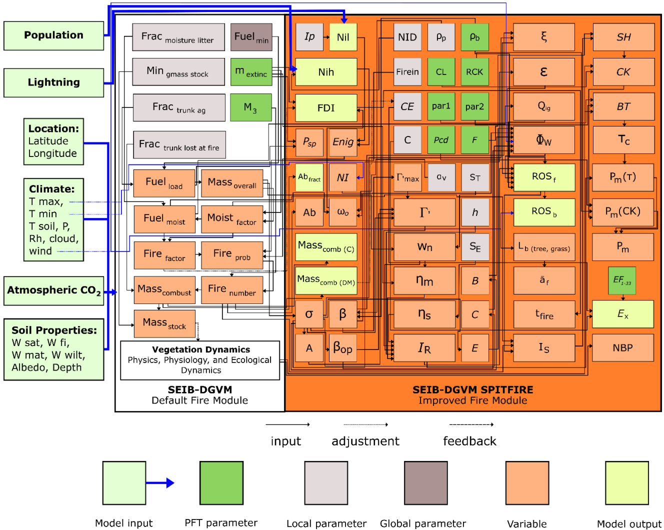
205 Figure 2. SEIB-DGVM SPITFIRE systems diagram. Describing the improvements (SPITFIRE), the interaction between the previous fire module (Glob-FIRM). All original SPITFIRE variables were integrated: ignition factor (lightning and population), PFT parameters, and other fire-related variables. In addition to the default annual output, the improved module had monthly outputs of all variables depending on the user needs. For the meaning of abbreviations, refer to the Appendix A.3.
