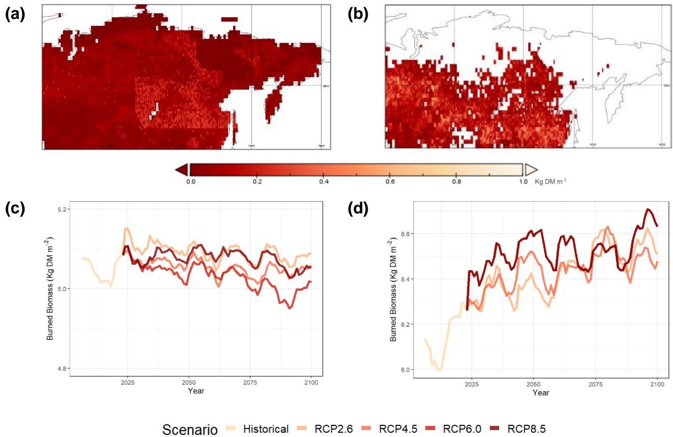
Figure 8. (a) Spatial distribution of annual averaged burned biomass of SEIB-DGVM GlobFIRM from 2006 to 2100. (b) Spatial distribution of annual averaged burned biomass of SEIB-DGVM SPITFIRE from 2006 to 2100. (c) Temporal variation of burned biomass of SEIB-DGVM GlobFIRM from 2006 to 2100. (d) Temporal variation of burned biomass of SEIB-DGVM SPITFIRE from 2006 to 2100.
