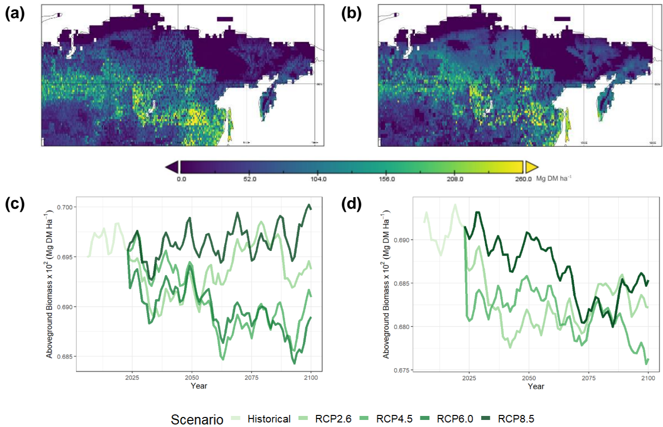
Figure 9. (a) Spatial distribution of annual averaged aboveground biomass of SEIB-DGVM GlobFIRM from 2006 to 2100. (b) Spatial distribution of annual averaged aboveground biomass of SEIB-DGVM SPITFIRE from 2006 to 2100. (c) Temporal variation of aboveground biomass of SEIB-DGVM GlobFIRM from 2006 to 2100. (d) Temporal variation of aboveground biomass of SEIB-DGVM SPITFIRE from 2006 to 2100.
