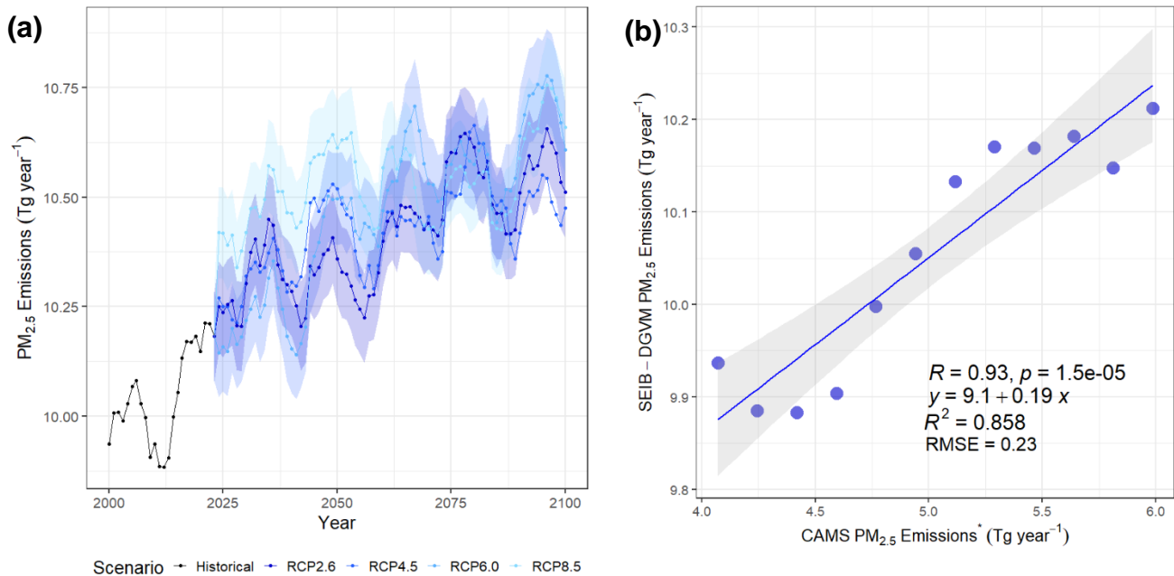
410 Figure 7. (a) Temporal variation of projected PM 2.5 emissions under several climate scenarios from 2000 to 2100. Standard deviation obtained from the annual PM 2.5 emission value of each climate scenarios (RCP8.5, RCP6.0, RCP4.5, and RCP2.6). (b) Comparison of PM 2.5 emissions from the SEIB-DGVM SPITFIRE model with the *trendline processed data from the Copernicus Atmosphere Monitoring Service in seven regions in Russia from 2004 to 2021 (Romanov et al., 2022).
