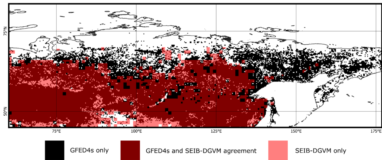
330 Figure 4. Spatial distribution comparison of annual averaged burned fraction variable (1997-2016) of SEIB-DGVM SPITFIRE and GFED4s
