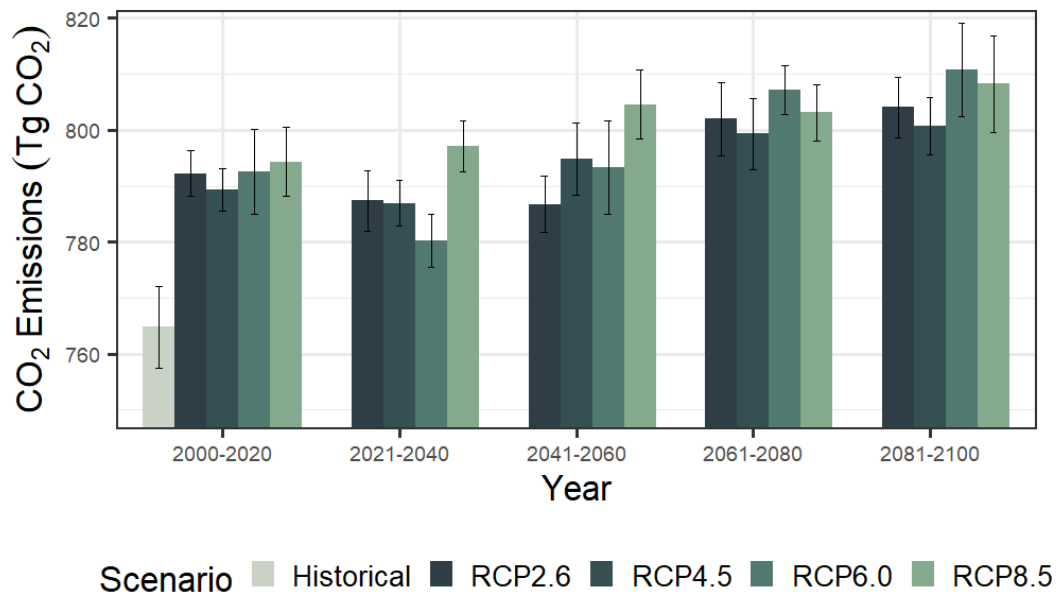
Figure 13. Temporal variation of projected CO 2 emissions from 2000 to 2100 under different RCPs scenarios.
