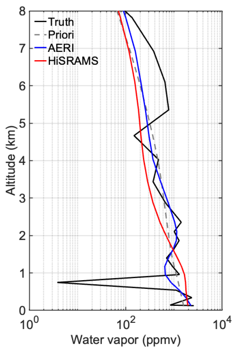
Figure 5: Comparing retrieved water vapor concentration profiles from ground-based AERI and HiSRAMS measurements with radiosonde-derived truth.
