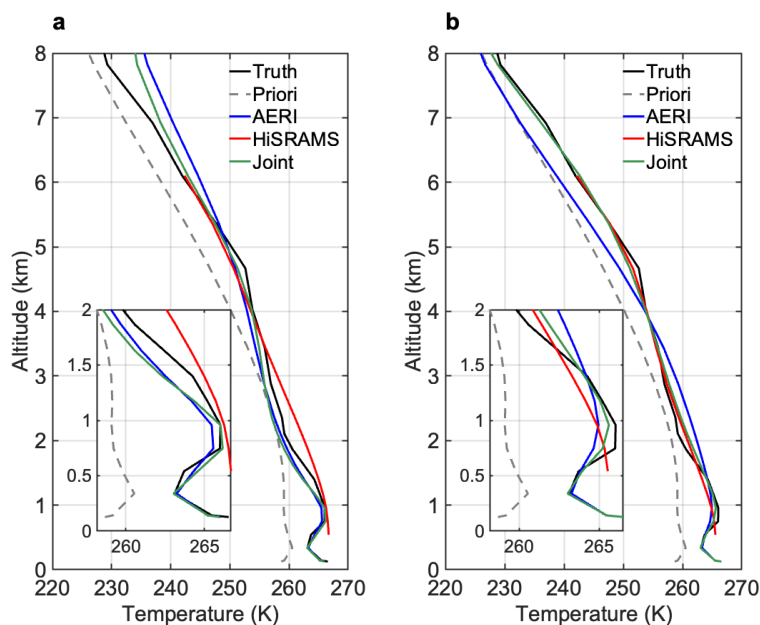
375 Figure 10: Retrieved temperature profiles for joint retrieval (combining AERI zenith-pointing measurements on the ground and HiSRAMS nadir-pointing measurements at 6.8 km) and single-instrument retrievals (utilizing either AERI zenith-pointing measurements on the ground or HiSRAMS nadir-pointing measurements at 6.8 km). (a) Retrieved temperature profiles based on actual measurements. (b) Retrieved temperature profiles based on synthetic measurements.
