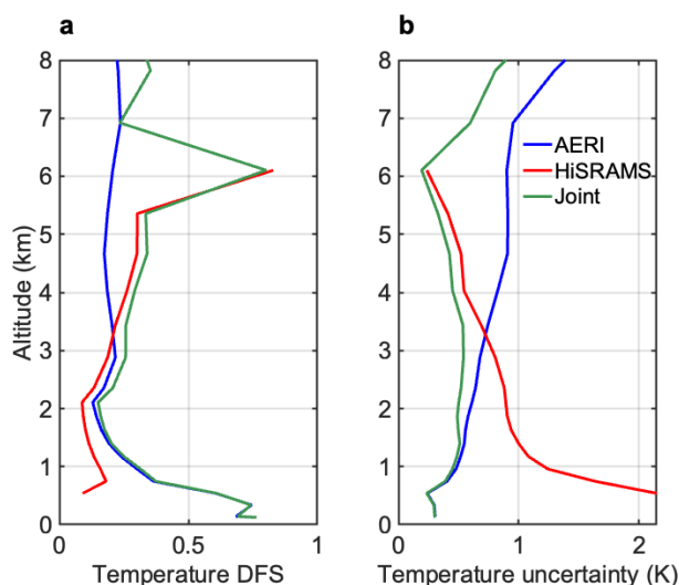
360 Figure 9: Comparison of information content and temperature retrieval uncertainty between joint airborne HiSRAMS and ground-based AERI retrievals versus single-instrument retrievals from either airborne HiSRAMS or ground-based AERI. (a) Temperature Degrees of Freedom for Signal (DFS). (b) Uncertainty in retrieved temperature.
