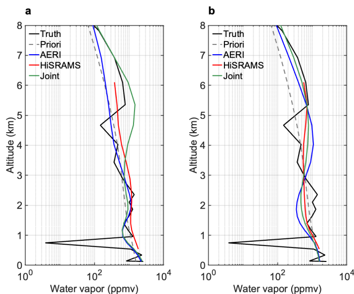
420 Figure 12: Retrieved water vapor concentration profiles for joint retrieval (combining both AERI zenith-pointing measurements on the ground and HiSRAMS nadir-pointing measurements at 6.8 km) and single-instrument retrievals (utilizing either AERI zenith-pointing measurements on the ground or HiSRAMS nadir-pointing measurements at 6.8 km). (a) Retrieved water vapor profiles based on actual measurements. (b) Retrieved water vapor profiles based on synthetic measurements.
