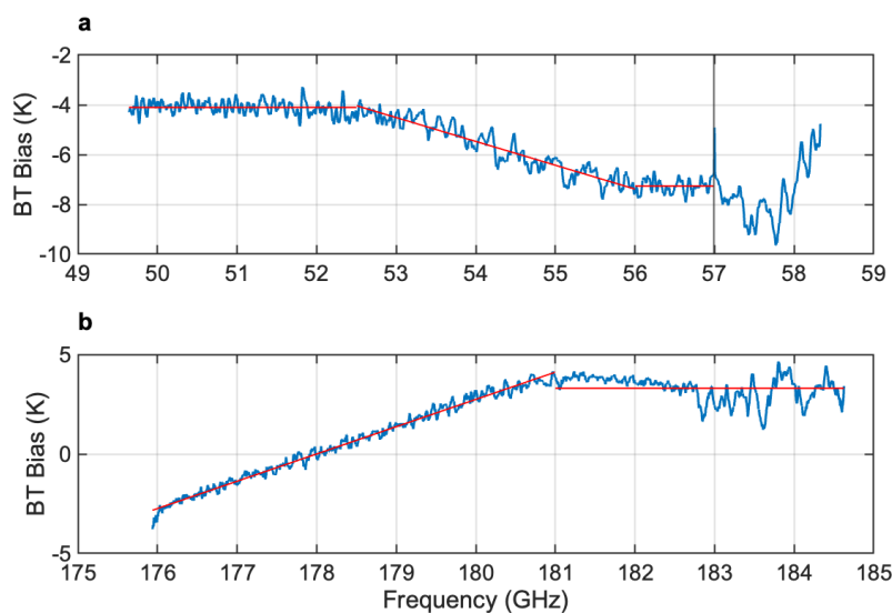
Figure A1. Correction of nadir-pointing HiSRAMS measurements bias in (a) oxygen band and (b) water vapor band. The blue lines represent the brightness temperature bias determined by the difference between measurements and forward model simulations (refer to Liu et al., 2023 for detailed methodology). The red lines represent the determined bias.
