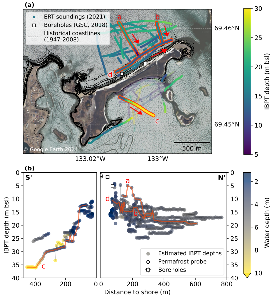
Figure 6. (a) Map view of IBPT depth around Tuktoyaktuk Island. The red arrows indicate the directions of the highlighted profiles a to d as shown in Fig. 5. South of the island, several profiles have been removed (transparent lines). The historical coastline since 1947 show the faster degradation of the northern shoreline facing the open ocean (Hynes et al., 2014). Most of the profiles however lay beyond the shoreline of 1947. (b) IBPT depth over the distance to the shore, south and north of Tuktoyaktuk Island. The remaining profiles south of the island indicated a steeper slope of the IBPT table compared to the northern side. The profiles shown in Fig. 5 are highlighted in red.
