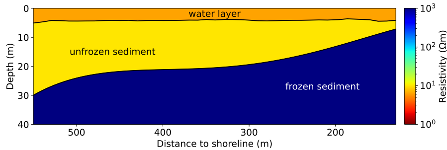
Figure 3. Synthetic model used to infer the most suitable inversion technique for this specific setting. The model consists of three layers: The upper layer represents the water body with a depth of 5 m and a resistivity of 6.1 \Omega\text{m} . The second and third layers have resistivities of 10 \Omega\text{m} and 1000 \Omega\text{m} , representing unfrozen and frozen sediment, respectively. The boundary between the two layers ranges from depths of 7 to 30 m and dips at varying angles, which is a plausible scenario for the IBPT in a profile perpendicular to the shoreline of Tuktoyaktuk Island.
