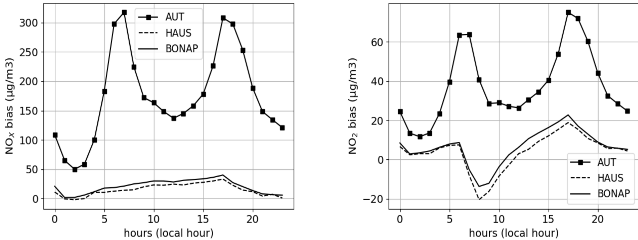
Figure 9. Daily profiles of the bias (in \mu\text{g}\cdot\text{m}^{-3} ) between MUNICH and Subgrid simulations over the period of February-March 2014, for \text{NO}_x and \text{NO}_2 concentrations.
